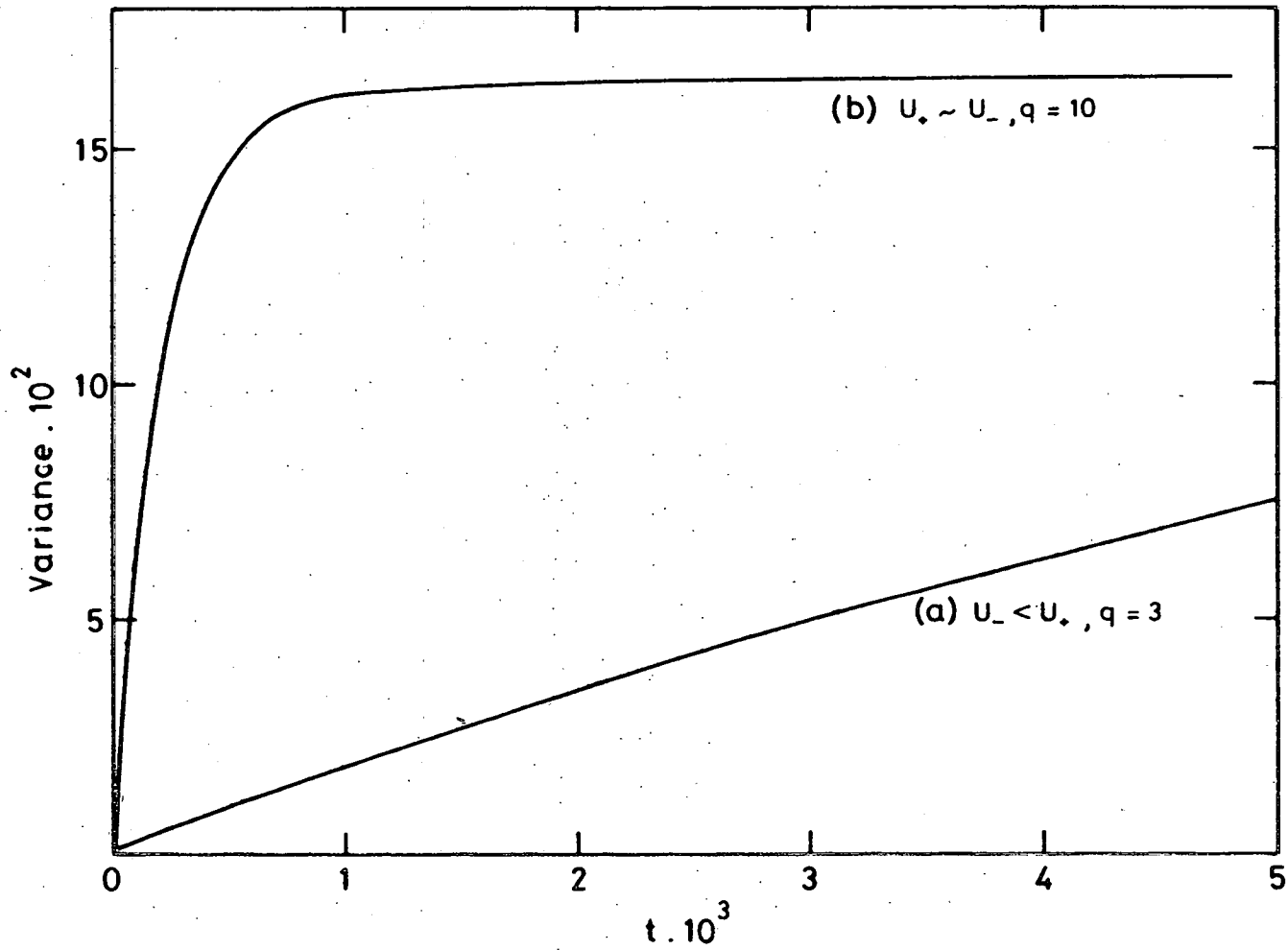
Fig. 7.- Time evolution of the variance of the probability distribution. curve (a) : State T_- is dominant and q = 3 \text{ yr}^{-1/2} \text{ } ^\circ\text{K} . curve (b) : States T_+ and T_- are equally dominant and q = 10 \text{ yr}^{-1/2} \text{ } ^\circ\text{K} .
