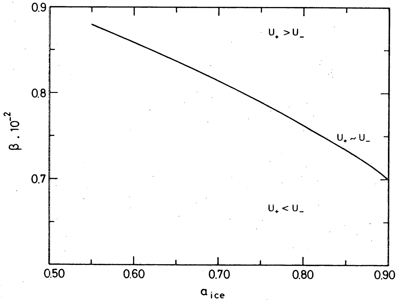
Fig. 3.- Climatic coexistence curve : Values of temperature feedback parameter \beta versus albedo of ice, a_{ice} for which U_+ \sim U_- .
