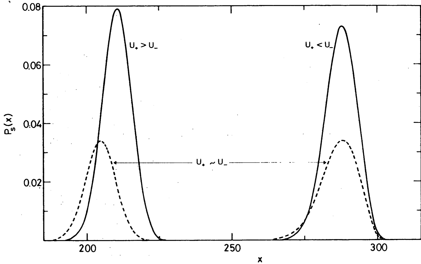
Fig. 2.- Steady-state probability distribution P_s(x) for three representative cases : U_+ > U_- , U_+ \sim U_- and U_+ < U_- and for q = 7 \text{ yr}^{-1/2} \text{ } ^\circ\text{K} . Note that, in the second case, P_s(x) is a two-hump distribution.
