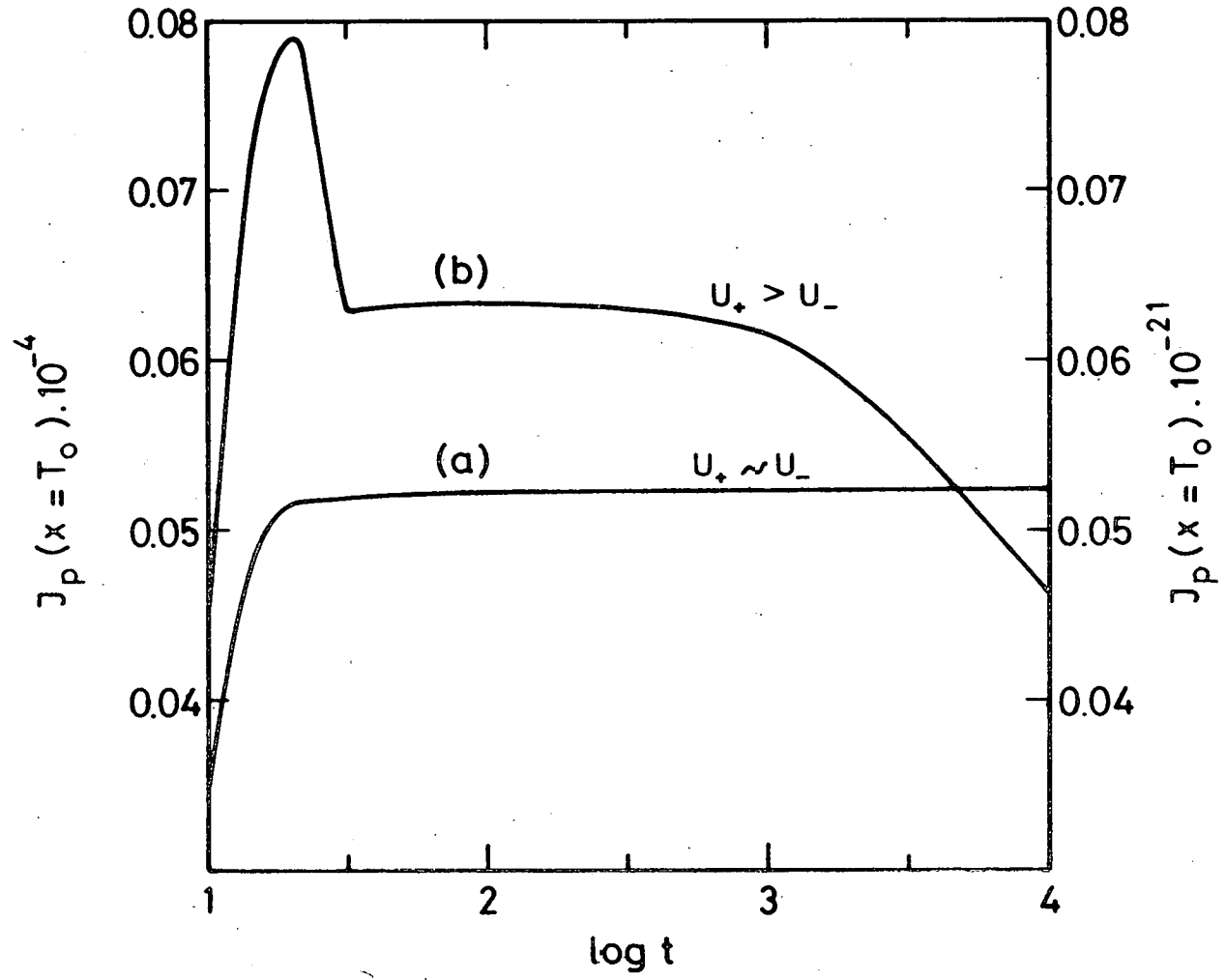
Fig. 6.- Time evolution of the probability flux J_p at the minimum T_0 of P , for q = 3 \text{ yr}^{-1/2} \circ K . The initial condition is a Gaussian distribution centered on T_+ . curve (a) : Probability flux when T_+ and T_- are equally dominant. curve (b) : Probability flux when T_- is dominant.
