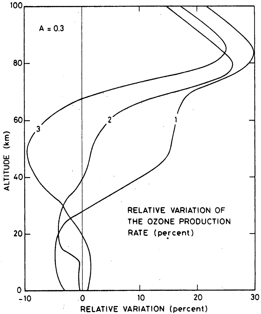
Fig. 2.- Relative variation of the ozone production rate during a solar cycle of 11 years when the solar irradiance variability suggested by Hinteregger is adopted. Curves 1, 2 and 3 refer to the different extrapolations suggested on fig. 1.
