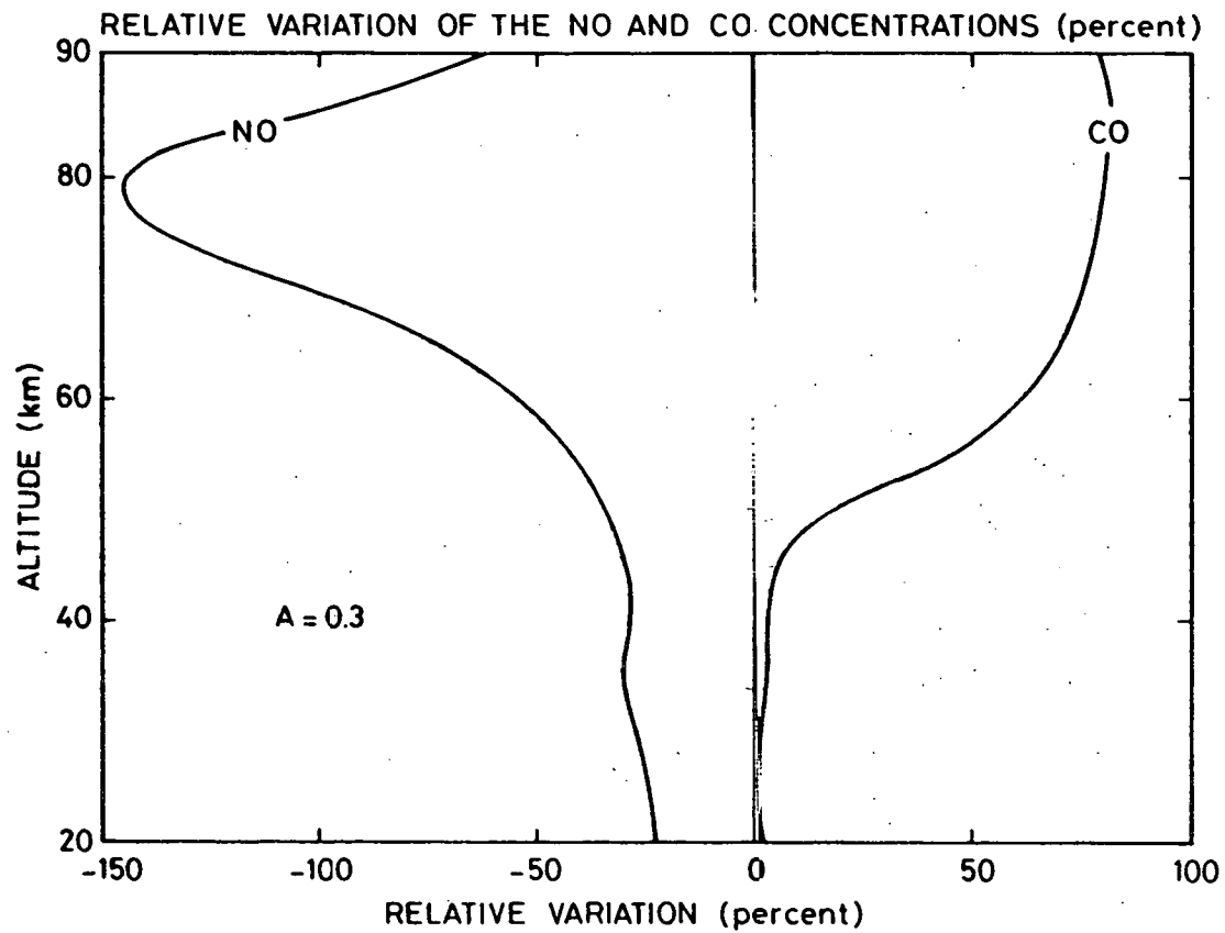
Fig. 4.- Relative variation in the concentration of carbon monoxide and nitric oxide during a solar cycle of 11-years. The calculations refer to the solar variability suggested by Brasseur and Simon (1980).
