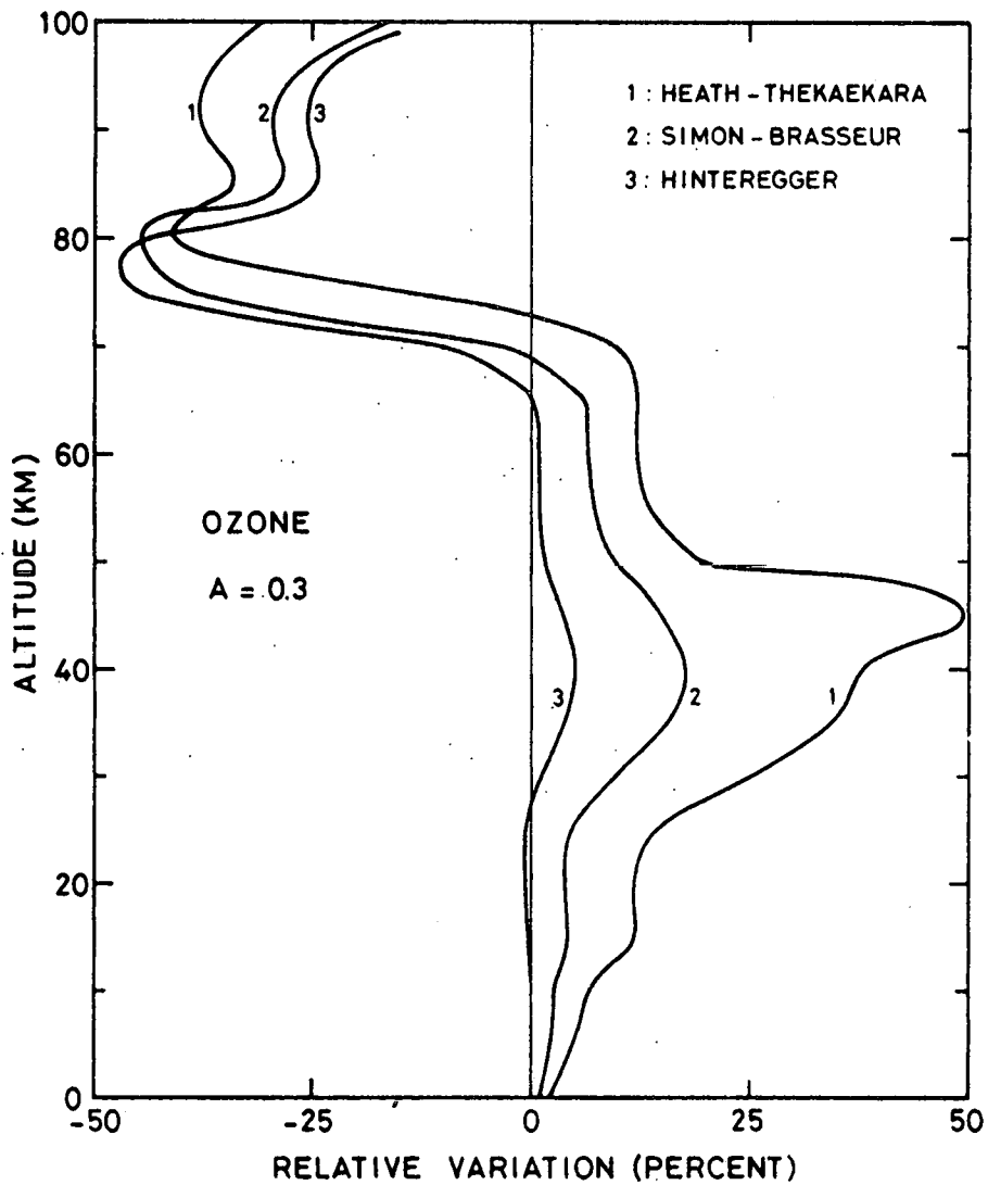
Fig. 3.- Relative variation of the ozone concentration computed for the solar variability suggested by Heath and Thekaekara (1977), Brasseur and Simon (1980) and Hinteregger (1980; extrapolation n° 2 on fig. 1). Ground albedo : 30 percent.
