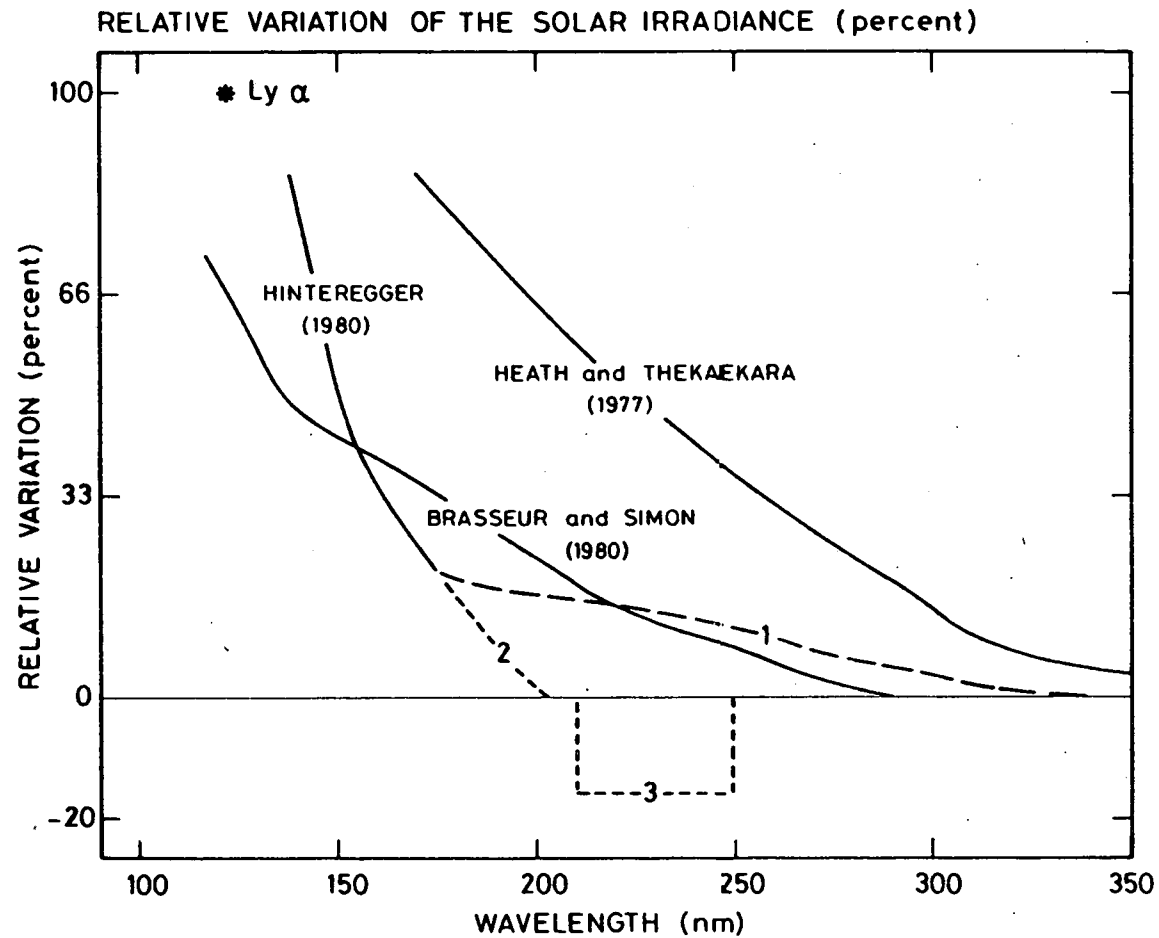
Fig. 1.- Relative variation of the solar irradiance during a cycle of solar activity (11 years). Spectral distribution suggested by various authors. The curve adopted by Brasseur and Simon (1980) has been extrapolated to reach 66% at 125 nm. For the extrapolation of the Hinteregger's curve, see text.
