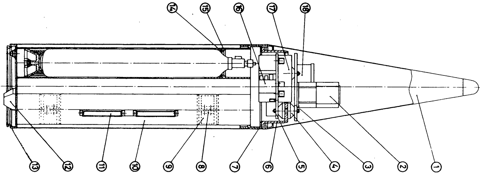
Fig. 1.- Schematic view of the NO-II payload. 1. Nose cone. 2. Security box. 3. Upper plate. 4. Shock mount. 5. Lower plate. 6. Intermediary plate. 7. Upper bulkhead. 8 and 9. Attachment ring. 10. Cylindrical pipes for the mounting of the bottles. 11. Explosive actuated miniature switch. 12. Mechanical stop unit for the preloaded spring system. 13. Lower bulkhead housing two manacle units. 14. Rubber seal (O-ring). 15. Stop flange ring. 16. Batteries. 17. Timer. 18. Radar transponder. The pyrotechnic devices used to make a hole in the bottles are fixed at the bottom of each cylinder.
