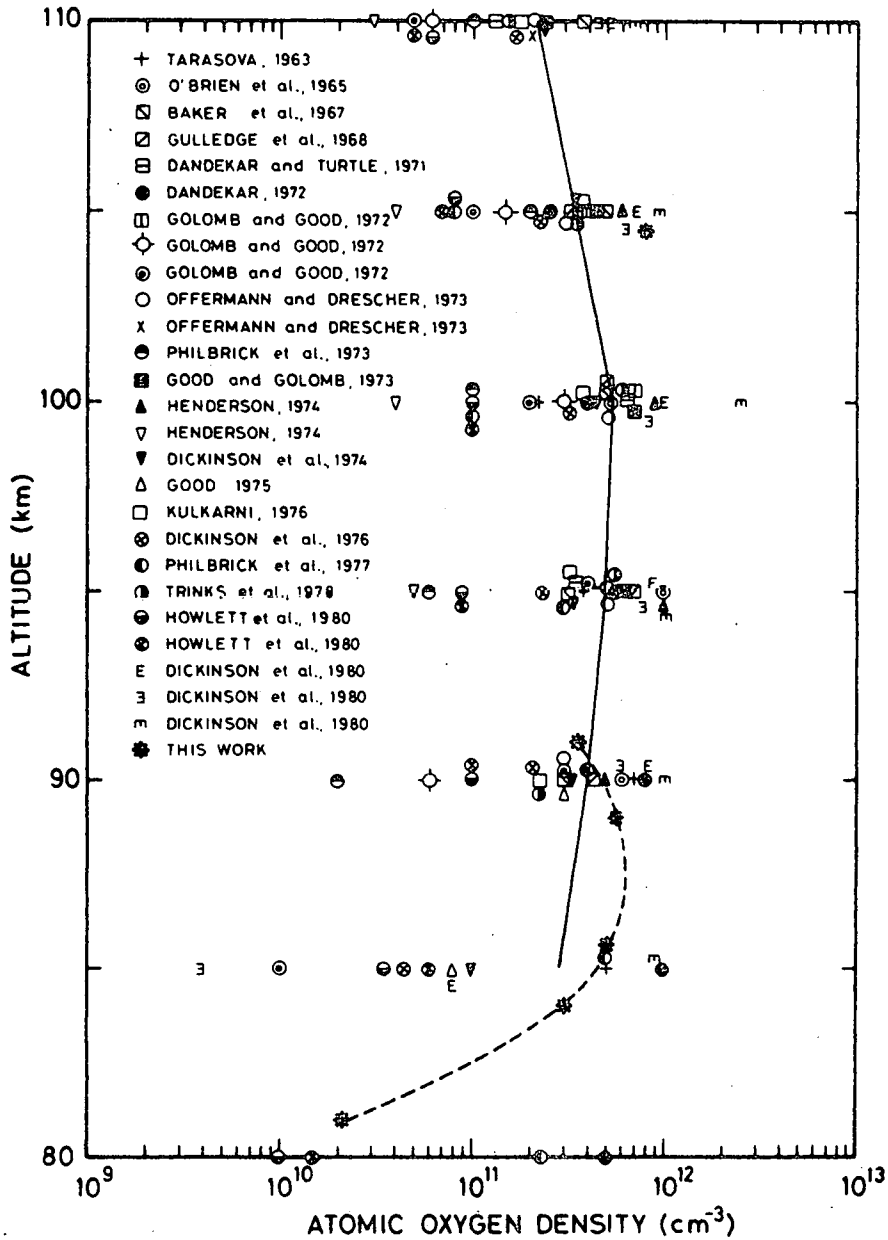
Fig. 6.- Atomic oxygen density values as a function of altitude for Kourou (dashed curve) compared with number densities reported by other workers. The solid trace represents the mean curve drawn through 5 km interval data points; the NO-II values are the arithmetic averages of all measurements made at a given altitude.
