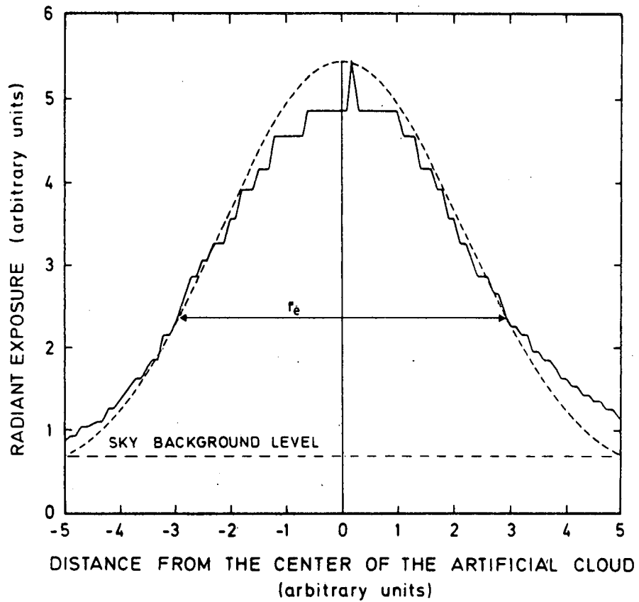
Fig. A.1.- Typical plot of the radiant exposure in function of the distance from the center of the artificial cloud (solid curve) compared with a best-fitted Gaussian density distribution (dashed curve) representing qualitatively the light energy deposited on the film during a time interval equal to the exposure time of the film.
