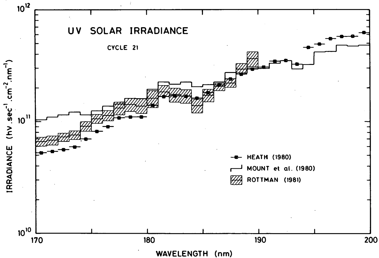
Fig. 5.- Comparison of ultraviolet solar irradiance integrated over 1 nm intervals from 170 to 200 nm measured during solar cycle 21. The shaded area represent the standard deviation of the five observations of Rottman (1981).
