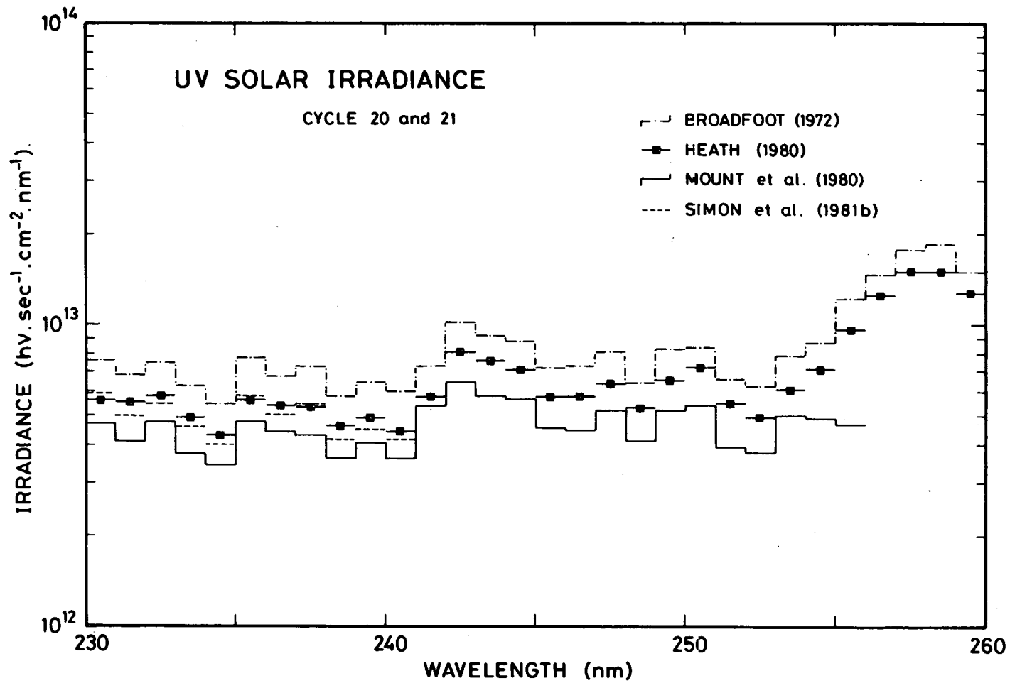
Fig. 9.- Comparison of ultraviolet solar irradiance integrated over 1 nm intervals from 230 to 260 nm. The measurements of Simon et al. (1981b) are not represented for the sake of clarity.
