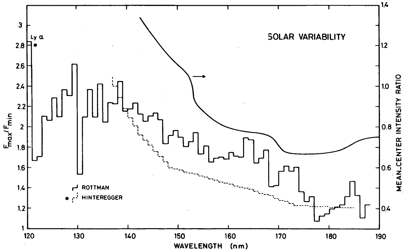
Figure 14 Solar irradiance variability ( F_{\max}/F_{\min} ) related to the rising phase of solar cycle 21, from 120 to 185 nm. The mean-to-center intensity ratios taken from Samain and Simon (1976) are also given for discussion (see text).
