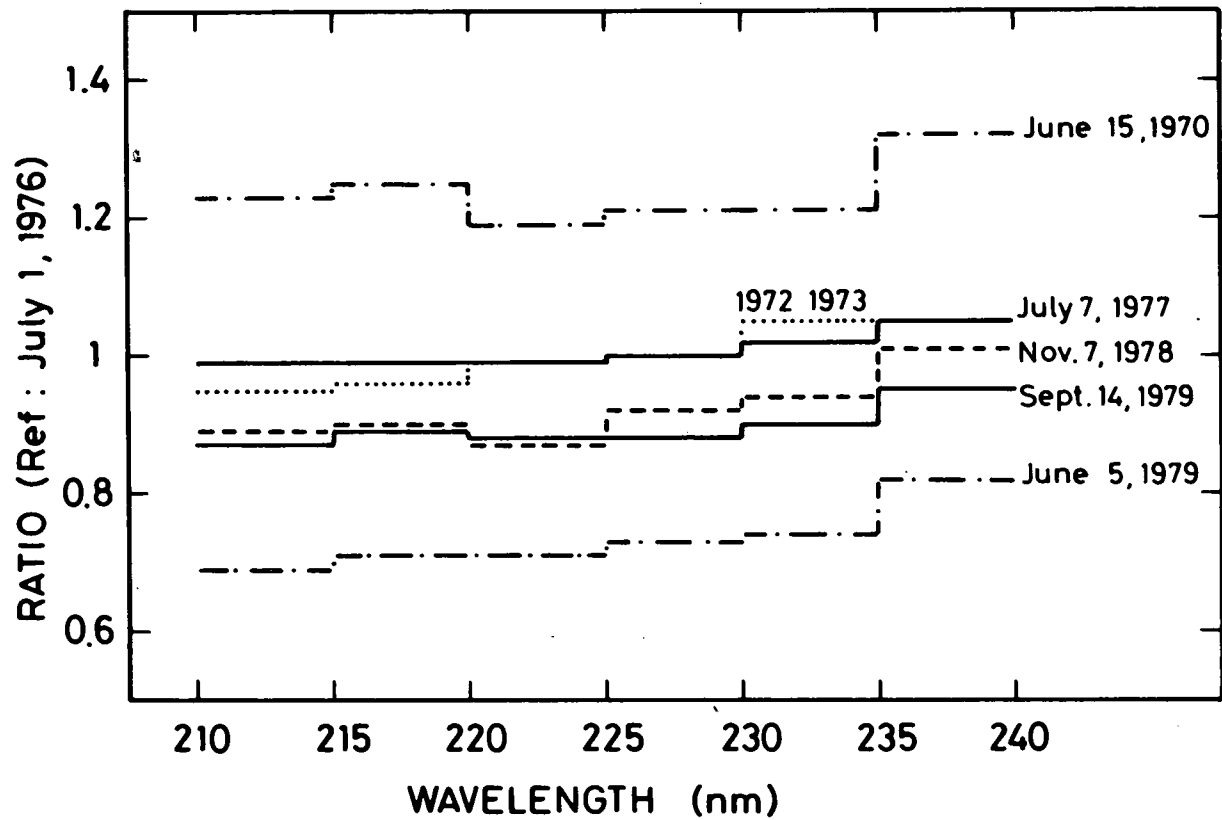
Fig. 8.- Ratio of solar irradiance measurements integrated over 5 nm intervals from 210 to 240 nm in comparison with the data of Simon et al. (1981a) obtained the 1st July 1976. See table 2 for references corresponding to the dates of observation.
