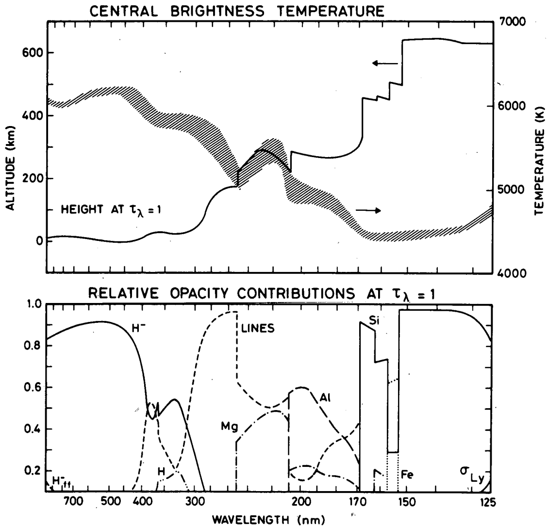
Fig. 13.- Continuum brightness temperature at the disc centre (shaded area) and height in the solar atmosphere for optical depth \tau_\lambda = 1 above \tau_{500} = 1 as a function of wavelength. The lower panel illustrates the relative contribution to the opacity at that height. ( \tau_\lambda = 1 ). The symbols H, Si, Al, Mg and Fe refer to neutral atom bound-free absorption, \sigma_{Ly} to scattering in the H I Lyman- \alpha line wing, and "lines" to a smoothly varying approximation to the effects of line blanketing. From Vernazza et al. (1976).
