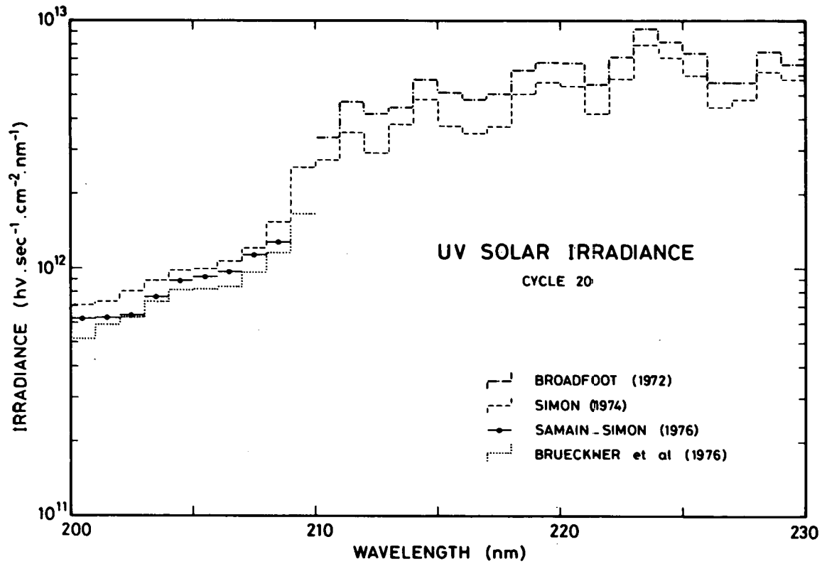
Fig. 6.- Comparison of ultraviolet solar irradiance integrated over 1 nm intervals from 200 to 230 nm, measured during solar cycle 20. The measurements of Ackerman et al. (1971) and Simon et al. (1981a) are not represented for the sake of clarity.
