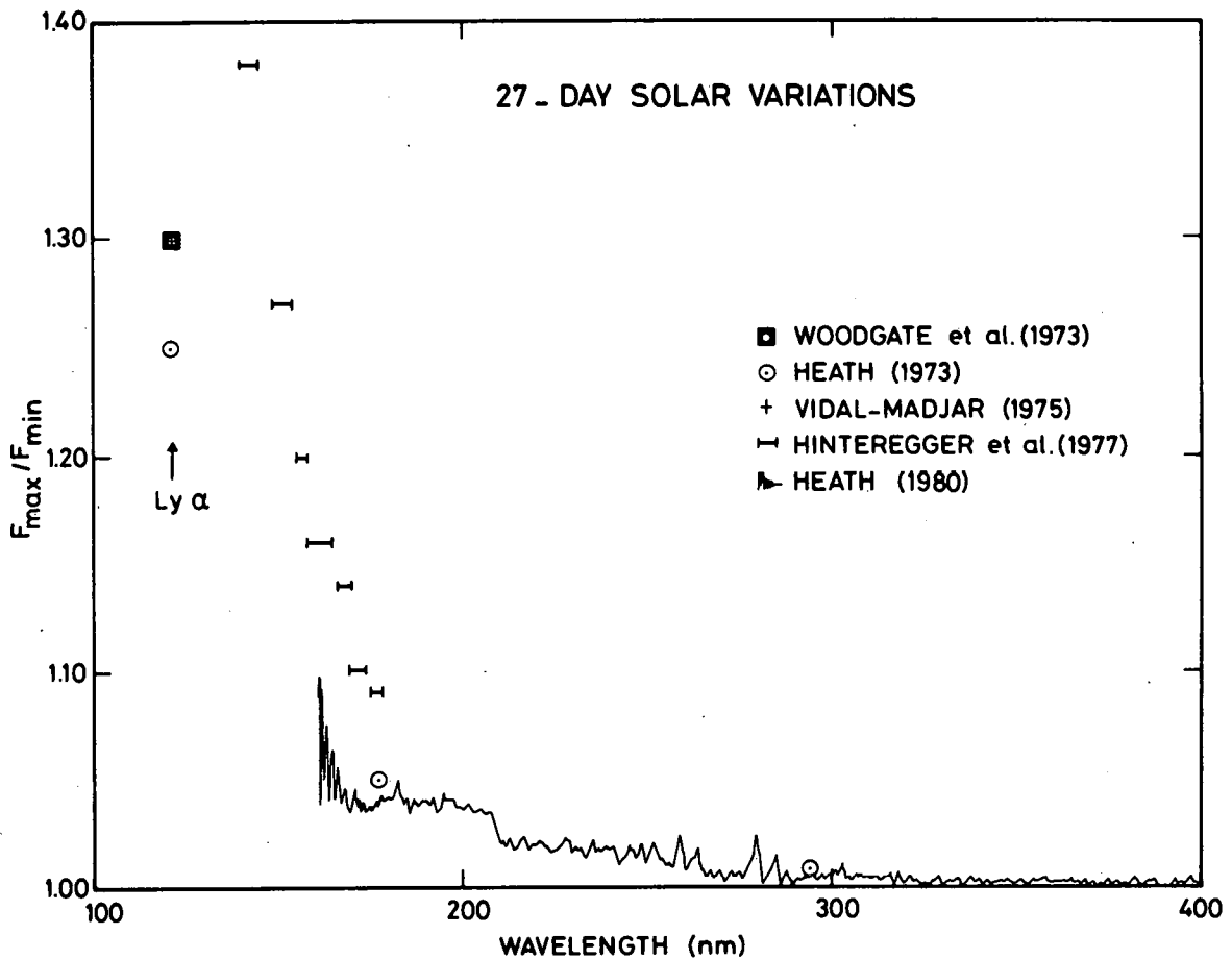
Fig. 12.- Solar irradiance variation related to the 27-day rotational period of the Sun from HI Lyman \alpha to 400 nm. The values of Hinteregger et al. (1977) correspond to the carrington rotation n o 1615 (June 1974) and those of Heath (1980) to Dec. 2, 1979, Jan. 2, 1979 and Feb. 5, 1979 for maximum values and to Dec. 21, 1978, Jan. 18, 1979 and Feb. 27, 1979 for minimum values.
