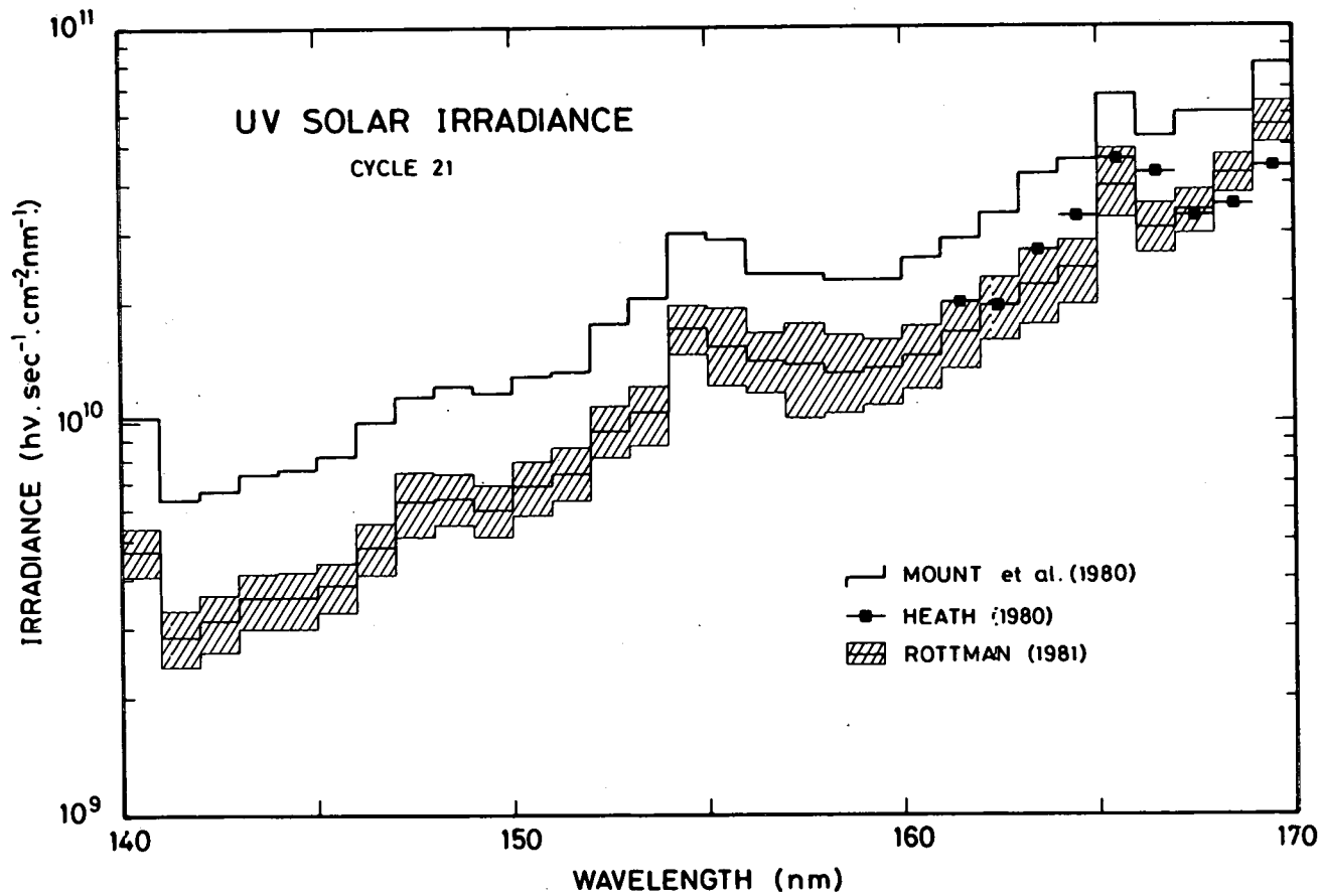
Fig. 3.- Comparison of ultraviolet solar irradiance integrated over 1 nm intervals from 140 to 170 nm, measured during solar cycle 21. The shaded area represent the standard deviation of the five observations of Rottman (1981).
