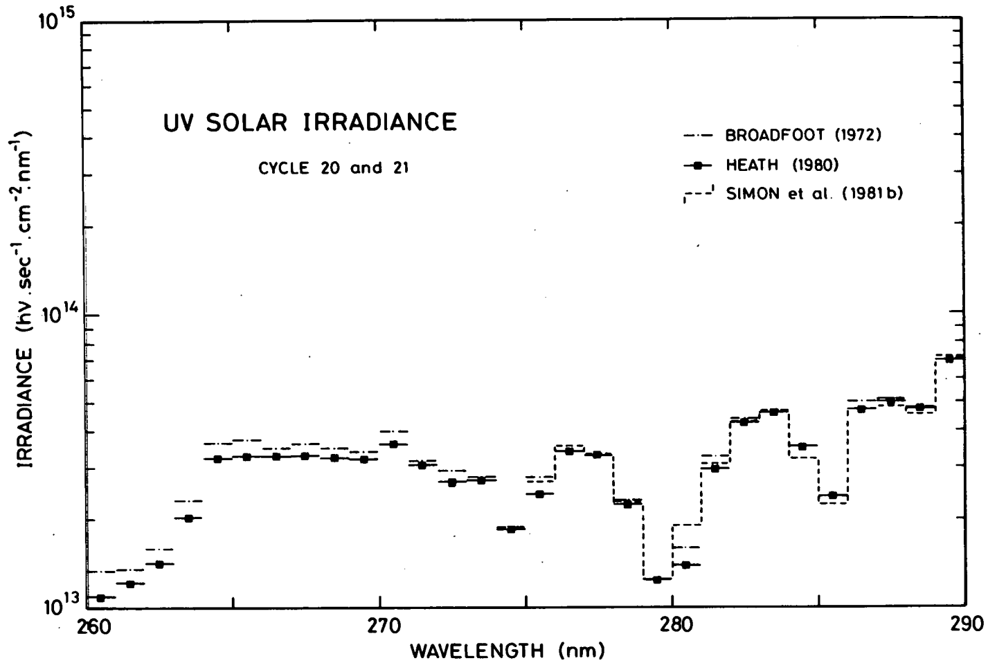
Fig. 10.- Comparison of ultraviolet solar irradiance integrated over 1 nm intervals from 260 to 290 nm. The measurement of Simon (1975) are not represented for the sake of clarity.
