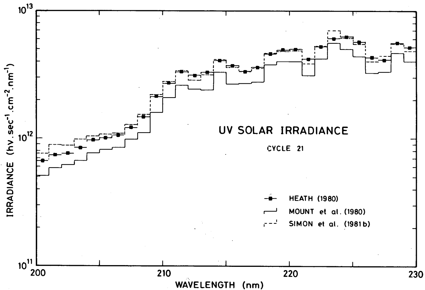
Fig. 7.- Comparison of ultraviolet solar irradiance integrated over 1 nm intervals from 200 to 230 nm, measured during solar cycle 21. The measurements of Simon et al. (1981a) are not represented for the sake of clarity.
