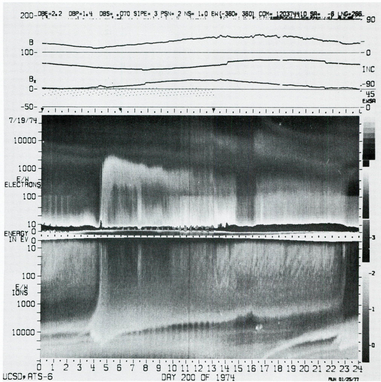
Fig. 3a.- The spectrogram of data from ATS 6 acquired on 19 July 1974. The electron and proton energy spectra have been measured with the plasma spectrometers which are directed nearly perpendicular to the magnetic field direction. The flux intensity is determined by the brightness of the photographic density. Local times and Universal times of the satellite ATS 6 are given respectively by the upper and lower scales. The top panels contain the intensity (B) the B_x component and the Inclination angle of the local magnetic field measured at the position of ATS 6.
