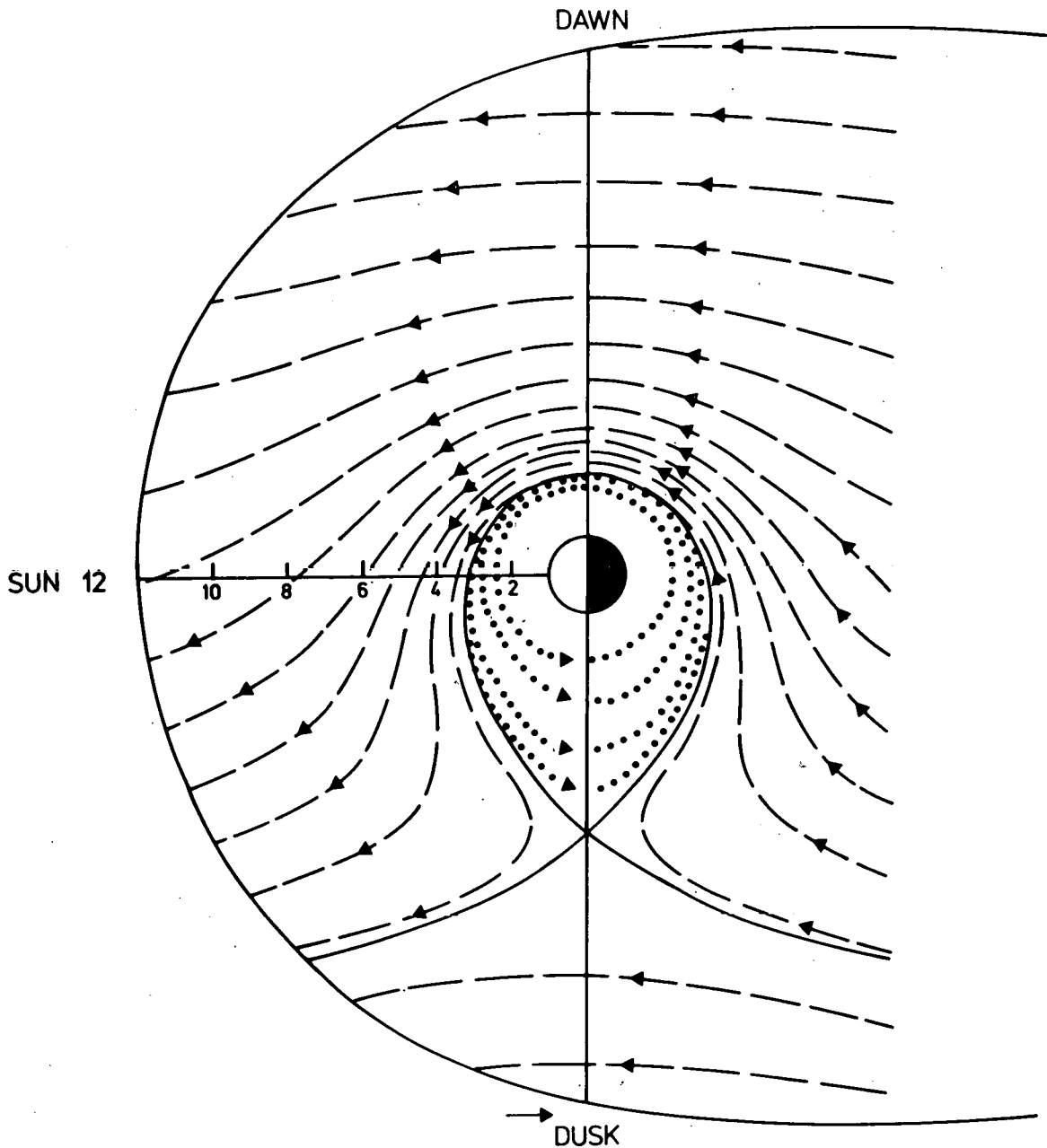
Fig. 2.- A contour plot of the uniform dawn-dusk electric field model by Kavanagh et al. (1968). The last closed equipotential passing through the singular point at 1800 LT, is chosen to fit the equatorial position of the plasmapause. The dotted curves are streamlines of electrons and ions confined within a region which has been identified with the plasma-sphere, according to the MHD-theory for the plasmapause formation.
