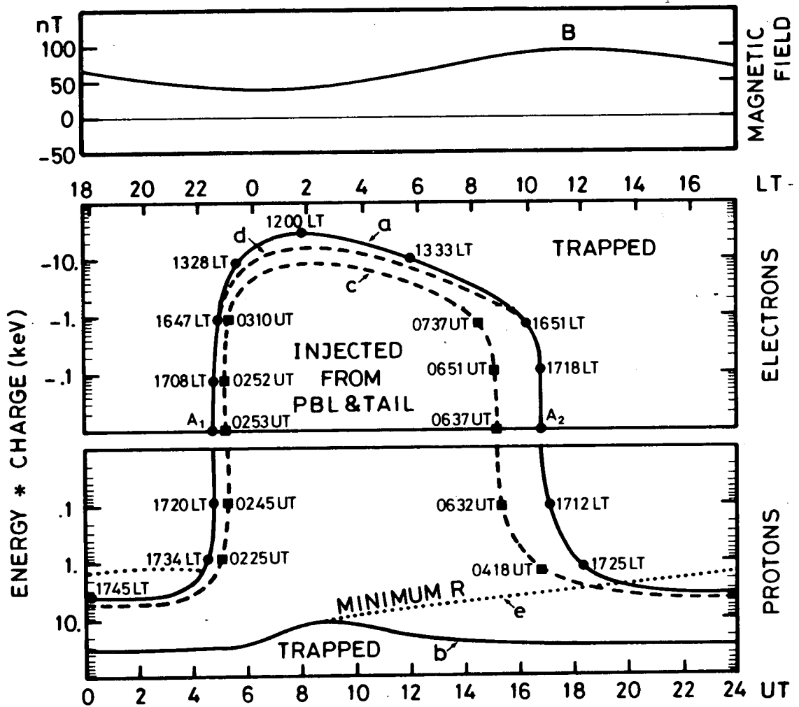
Fig. 3b. A plot showing the type of particle trajectories encountered by the ATS 6 geostationary satellite according to the E3H and M2 electric and magnetic field models. The scales are the same as in Fig. 3a.
