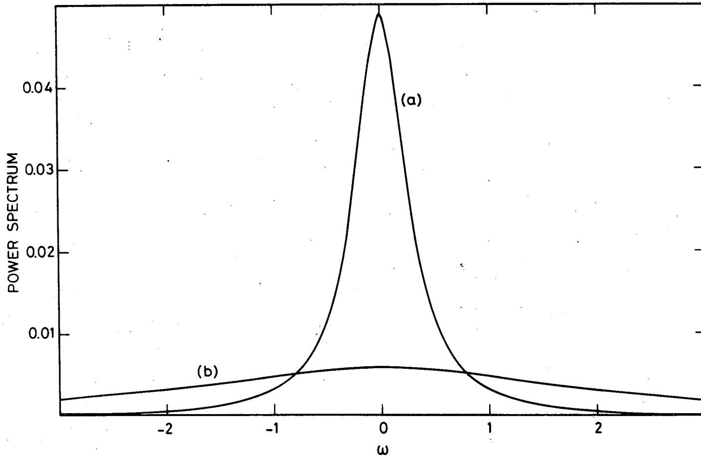
Fig. 1.- Power spectrum associated with the autocorrelation function of the mean surface temperature. Eq. (32) (curve (a)) and an Orstein-Uhlenbeck process (curve (b)), for q_2^2 = 1 \text{ Kcal cm}^{-2} \text{ yr}^{-1} . The parameters of the model described in Eq. (21) are as follows : Q = 252.76 \text{ Kcal cm}^{-2} \text{ yr}^{-1} , A = 159.24 \text{ Kcal cm}^{-2} \text{ yr}^{-1} , B = 1.17 \text{ Kcal cm}^{-2} \text{ yr}^{-1} , D = 0.44 \text{ Kcal cm}^{-2} \text{ yr}^{-1} , S(x) = 1 - 0.477 P_2(x) , a(x) = 0.697 - 0.00779 P_2(x) for x < x_s and a(x) = 0.38 for x > x_s , T_0^* = 14.9^\circ\text{C} , T_2^* = -28.2^\circ\text{C} , x_s^* = 0.96 .
