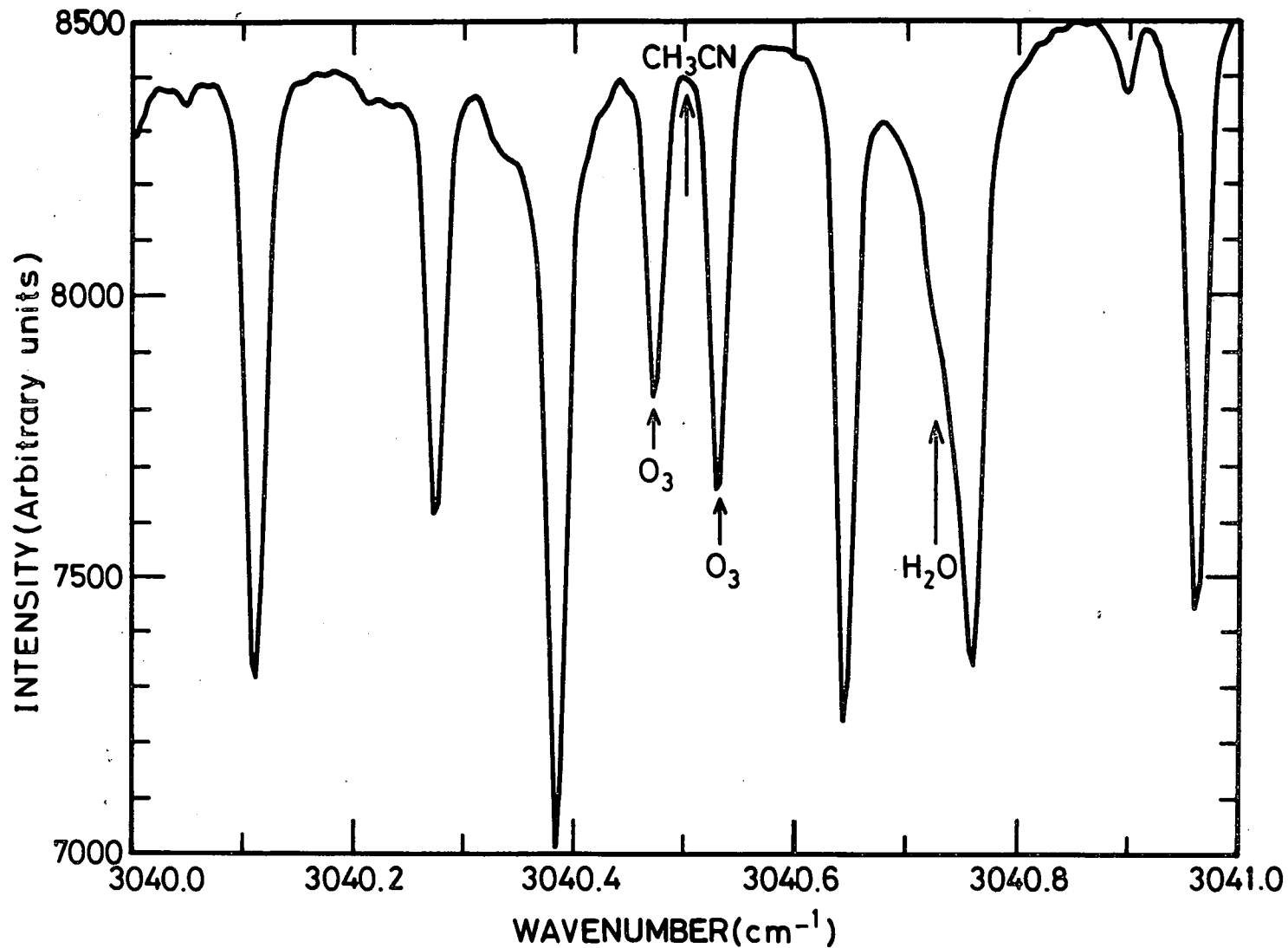
Fig. 1.- Portion of the Delbouille et al. (1981) atlas indicating the region of expected CH 3 CN absorption; the width of the lines except for the shoulder marked H 2 O permits to identify them as stratospheric ozone lines.
