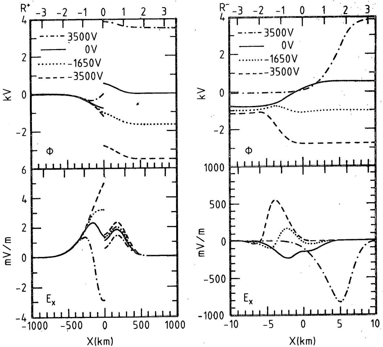
Figure 2 : Electric potential ( \phi ) and electric field ( E ) structures for different values of \phi_2 - \phi_1 (+ 3500 V, 0 V, - 1650 V and - 3500 V). The left-hand side panels characterize the ion-dominated layers, located at both ends of the sheath, while the right-hand side panels pertain to the thin electron-dominated layer near x = 0 . Boundary conditions are given in table II. As in figure 1, the structure of the very thin electron-dominated layer near x = 0 is not displayed on the much larger scale of the ion-dominated layers (left-hand side panels).
