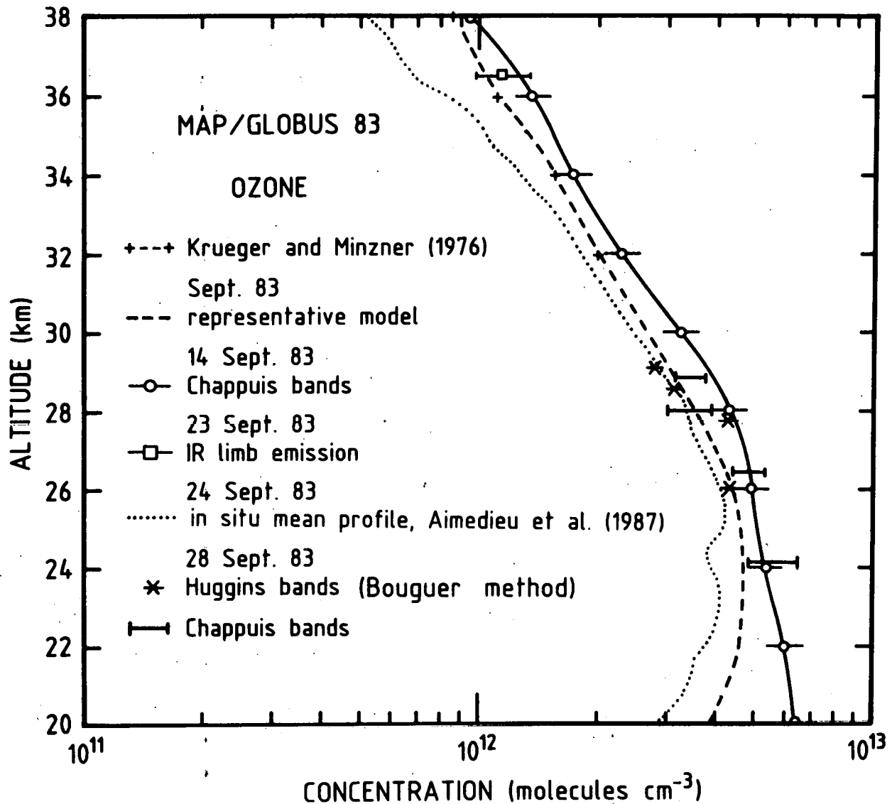
Figure 3. Comparison between ozone profiles deduced from remote sensing measurements performed during the MAP/Globus campaign in September 1983. In situ average profile deduced from measurements performed on 24 September 1983 is also shown for discussion purposes.
