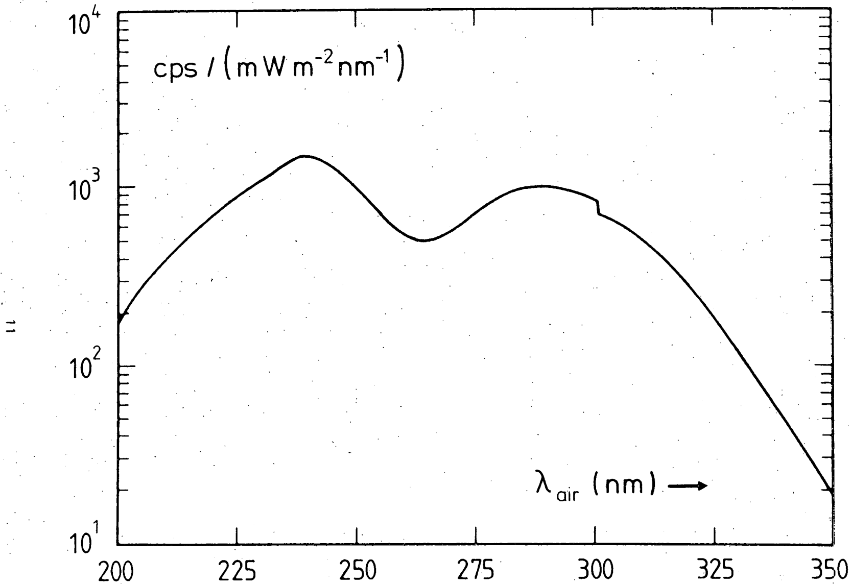
Fig. 4.- The overall responsivity of the UV-spectrometer. The step near 300 nm results from the insertion of a higher order separation filter.
