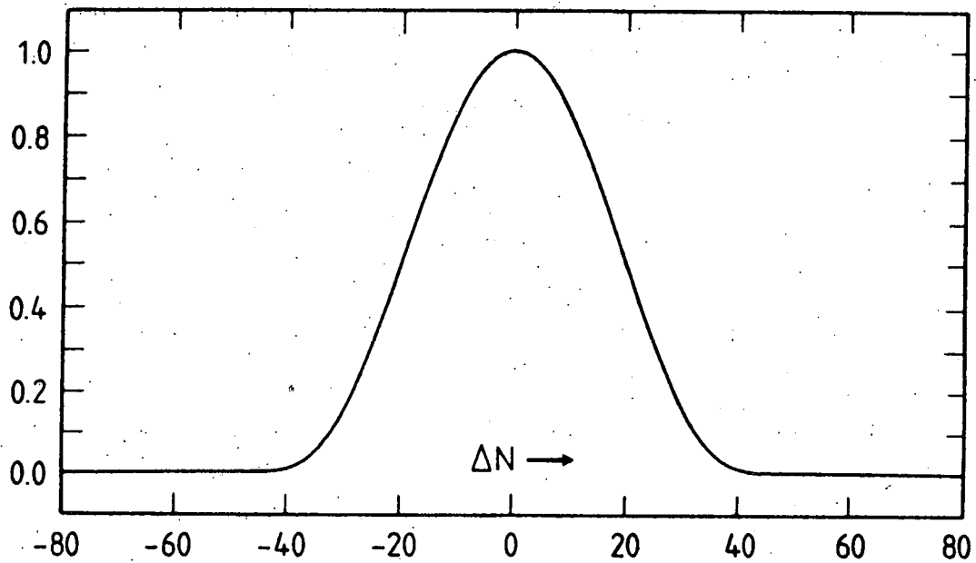
Fig. 5.- The passband-profile of the UV-spectrometer as a function of the difference \Delta N between the grating step number N and the step number at the passband-center. The profile is symmetric and does not depend on the central grating step number.
