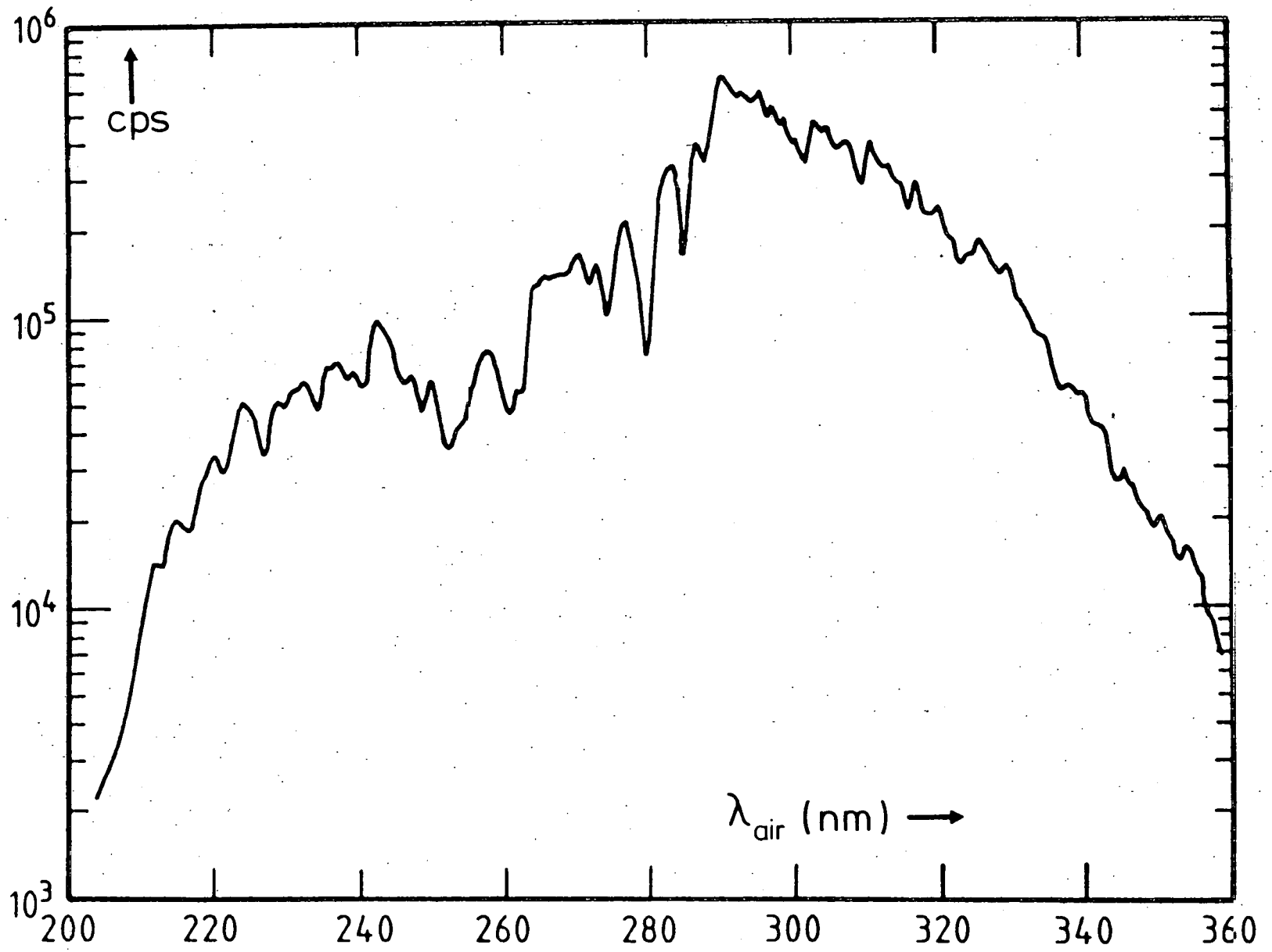
Fig. 6.- The Sun's signals as a function of (air)- wavelength \lambda_{\text{air}} (mean of the 19 undisturbed spectra).
