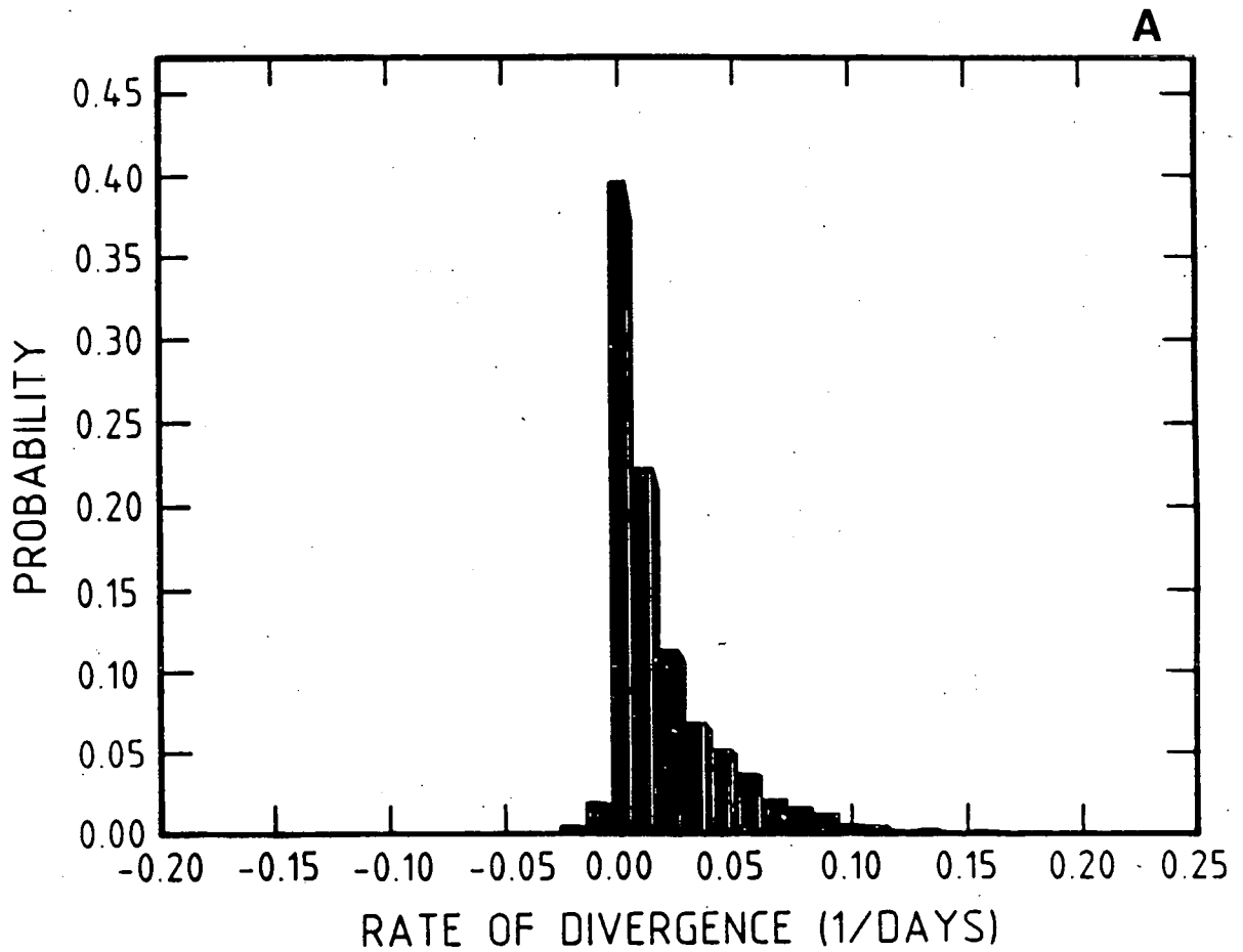
Fig. 9.- Histograms of the probability distribution of the local rates of divergence \beta_i , whose average yield the largest positive Lyapounov exponent, (a); and the most negative exponent, (b).
