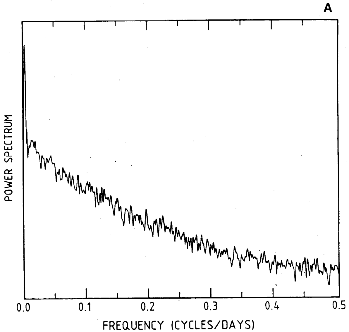
Fig. 2.- (a) Smoothed power spectrum of the daily 500 mb geopotential at Marseille (b) smoothed spectrum obtained from spatial averaging of the signal at nine stations.
