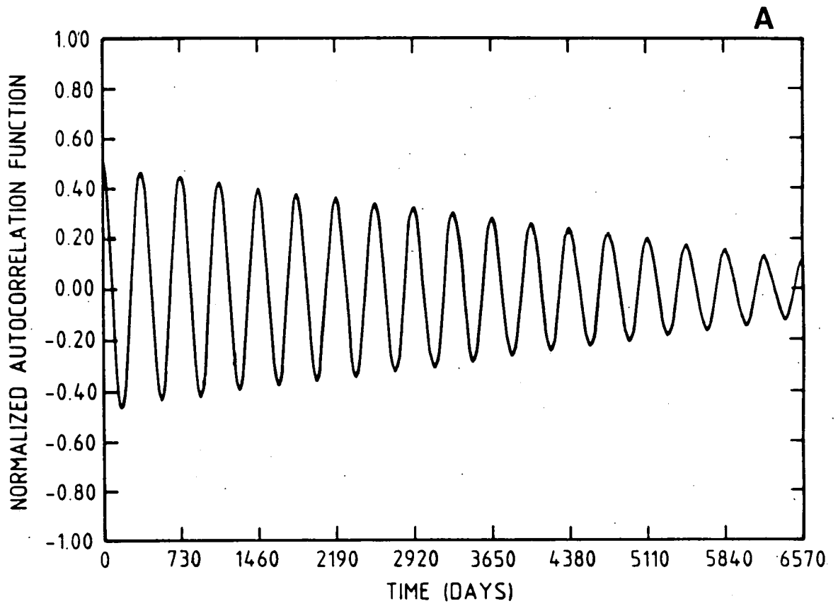
Fig. 3.- Correlation function of the geopotential signal over large time scales : (a) Marseille (b) spatial average of nine signals.
