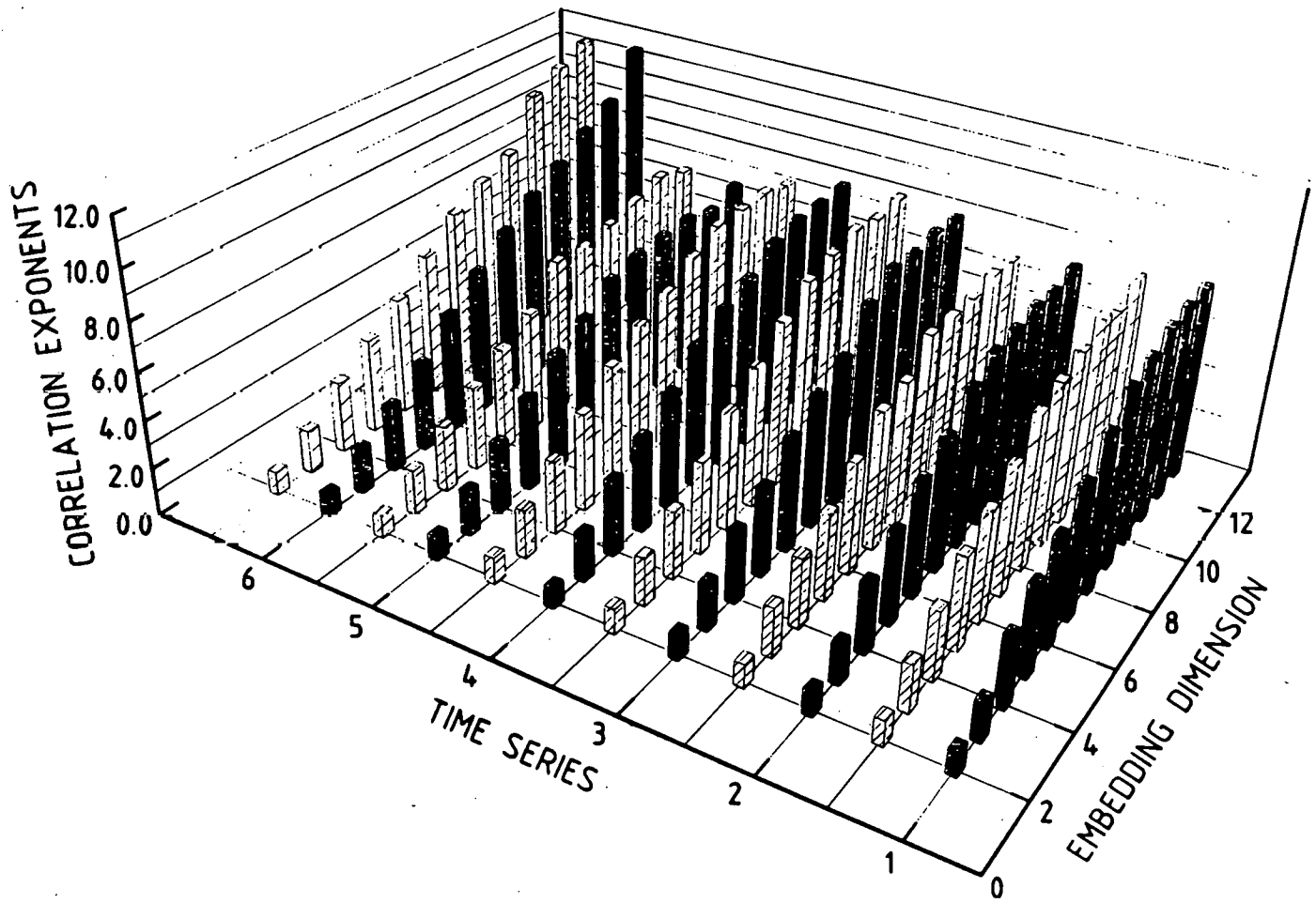
Fig. 8.- Correlation exponents obtained successively by the method of time delays (hatched blocks) and by the singular space construction (black blocks) for 6 signals. From left to right : pseudo-random signal, 500 mb geopotential height at Marseille, Stockholm, Rome, Reykjavik and Lisbon.
