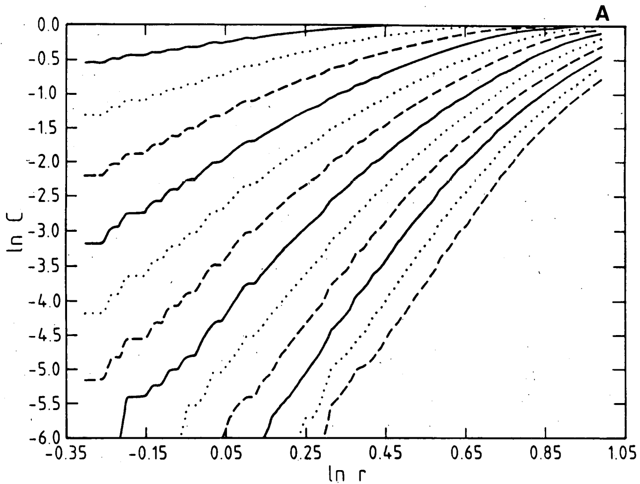
Fig. 7.- Plots of \ln C against \ln r for embedding dimensions n = 1 to n = 12 for Lisbon using method of time delays (a), and singular space (b).
