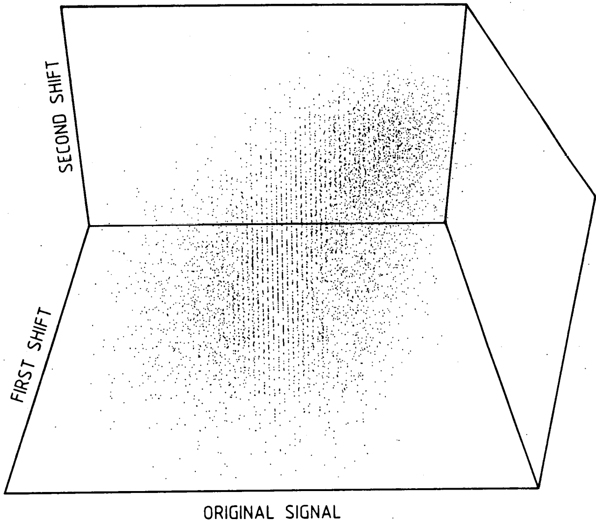
Fig. 4.- Three-dimensional projection of the entire trajectory for Marseilles obtained by the method of time delays, with a shift \tau = 10 days.
