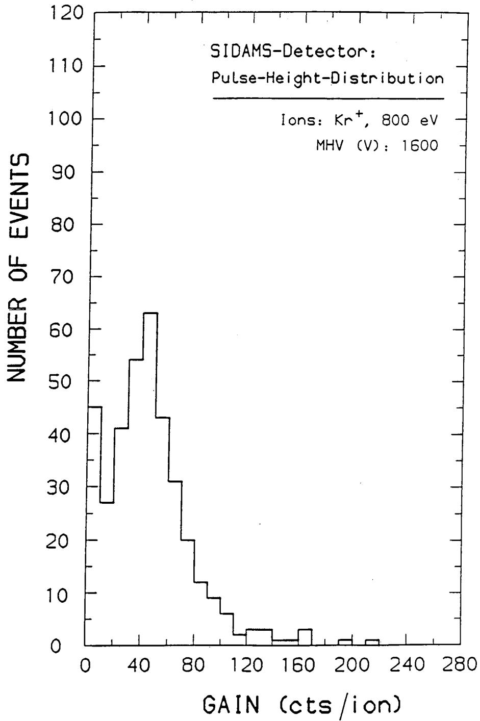
Fig. 6.- Pulse height distribution of Kr^+ ions at 800 eV energy measured with a curved 1-inch C2-type Galileo Optics MCP.
