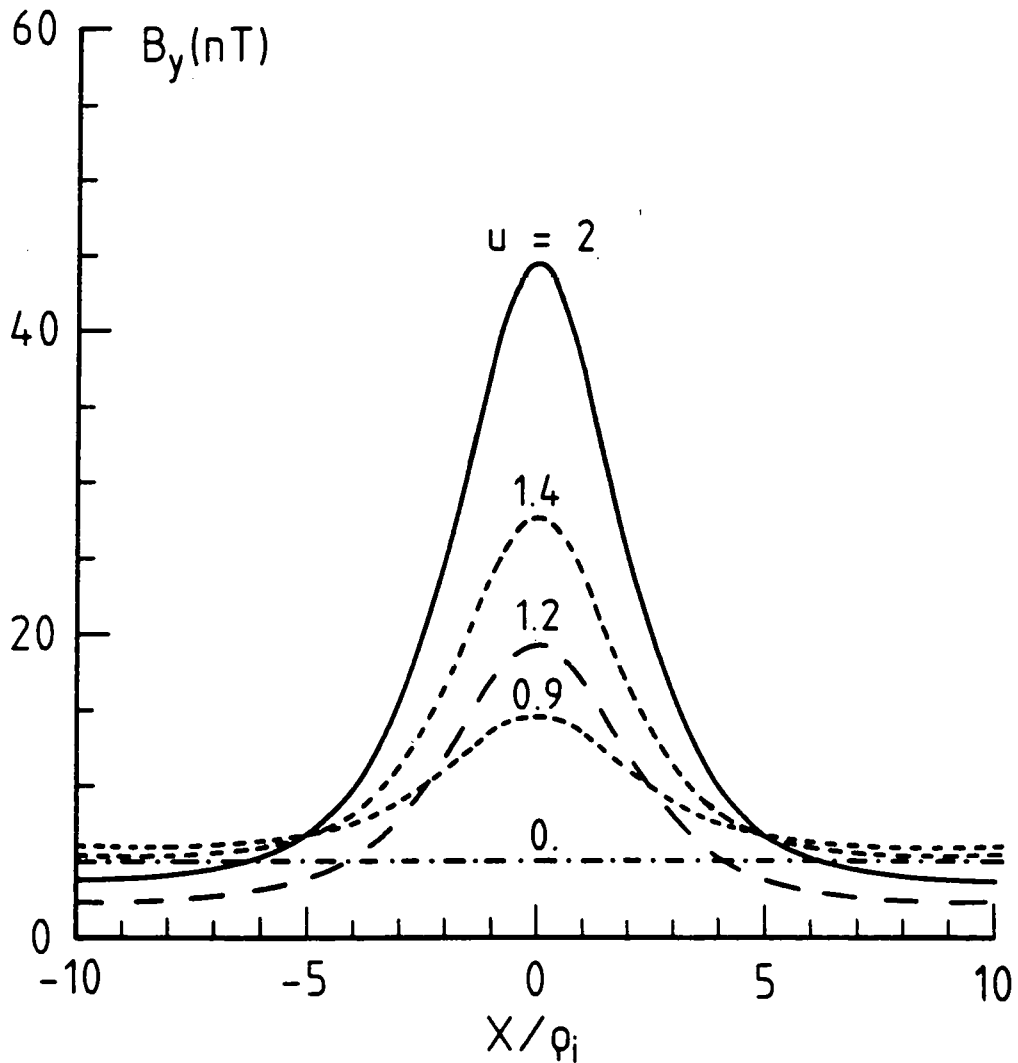
Figure 3: Profiles of the B_y component of the magnetic field for different values of the flow asymmetry factor u . The value of s_0 (the number density of “trapped” particles at x = 0 ) depends on the value of u as indicated in Table 1. For all cases considered in this figure the total angle of rotation of the magnetic field through the magnetopause is \theta_0 \approx 170^\circ . The other plasma and field parameters are the same as those used to compute Figures 1 and 2.
