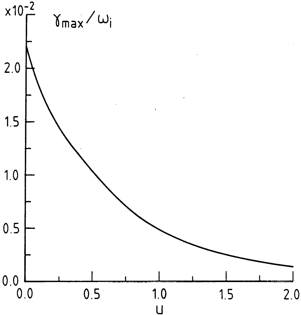
Figure 6: The dependence of the maximum growth rate of the tearing instability (normalized on the ion Larmor frequency \omega_i = eB_1/m_i c ) on the factor of flow asymmetry u .
