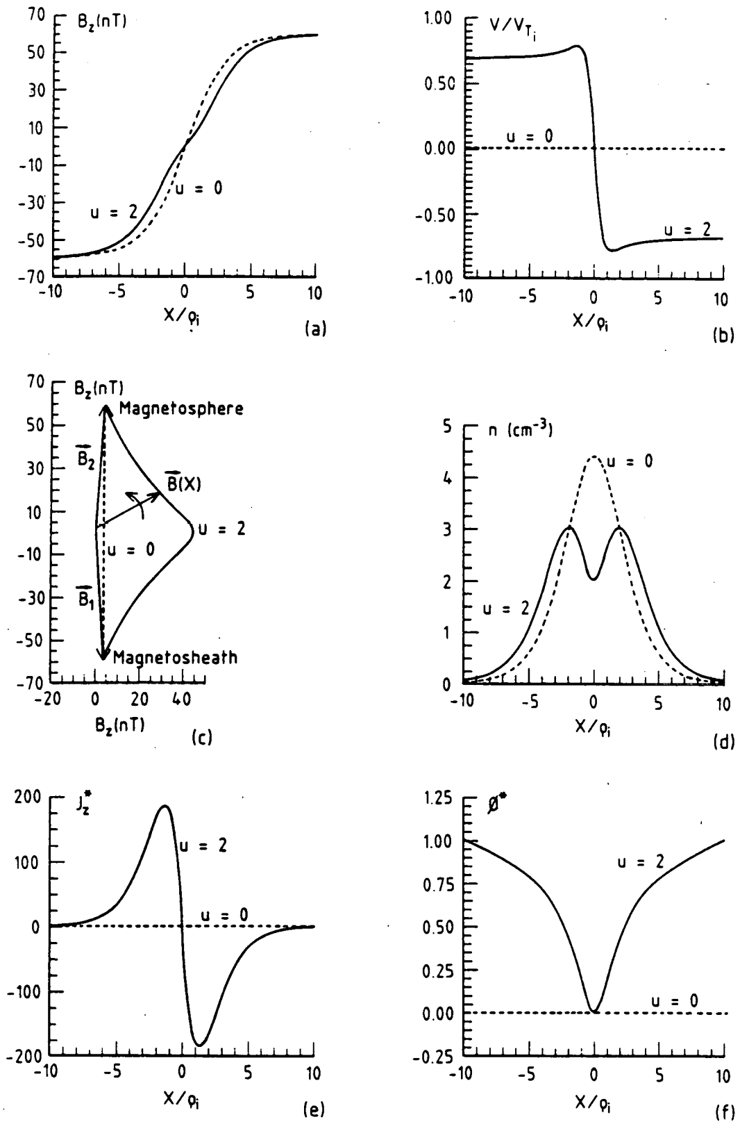
Figure 2: Same as Figure 1, but for the case u = 2 .
