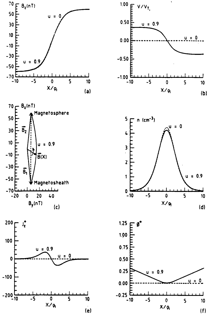
Figure 1: Structure of the magnetopause current layer for |B_1| = |B_2| = 60 nT, T_i = T_e = 1 keV, \theta_0 \approx 170^\circ , u = 0.9 . The ratio u = U/U_d is the factor of flow asymmetry. It represents half the relative flow ( U = |V_1 - V_2|/2 ) normalized to the ion drift velocity U_d = cT_i/eB_1D ( =146 km/s for the plasma and field parameters used here). The total angle of rotation of the magnetic field is \theta_0 . For comparison, the Harris profiles corresponding to u = 0 are also displayed and are represented by the dashed curves. From left to right and from top to bottom the following variables are illustrated. (a) B_z (in nanoteslas); (b) bulk flow velocity V/V_{Ti} ( V_{Ti} = (2T_i/m_i)^{1/2} is the ion thermal velocity; V_{Ti} = 438 km/s); (c) hodogram of the magnetic field (in nanoteslas); (d) number density n (in cubic centimeters); (e) J_z^* = J_{iz}^* + J_{ez}^* is the z component of the total current density normalized to \Lambda_J = s_1 e V_{Ti} (= 7 \times 10^{-10} A/m ^2 ); (f) electric potential \phi^* , normalized to \Lambda_\phi = 2T_i/e (= 2 \times 10^3 V). These plasma and field parameters are illustrated as a function of the distance x/\rho_i from the center of the layer (where \rho_i is the ion Larmor radius in the field B_1 ; \rho_i = 76.2 km). The configuration is also characterized by the following parameters: D = 1.5\rho_i \approx 114 km, s_1 = 0.01 cm ^{-3} . The value of the parameter s_0 depends on the value of u as determined in Table 1.
