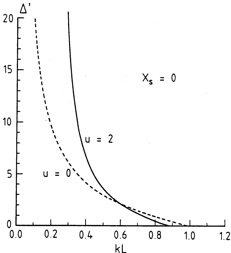
Figure 5: The dependence of the free energy of perturbations \Delta' of the central magnetic surface x = 0 on the wave number kL . The solid curve corresponds to a finite value of the flow asymmetry factor ( u = 2 ). For comparison, the corresponding profile of \Delta' for the symmetrical Harris configuration ( u = 0 ) is illustrated by the dashed curve.
