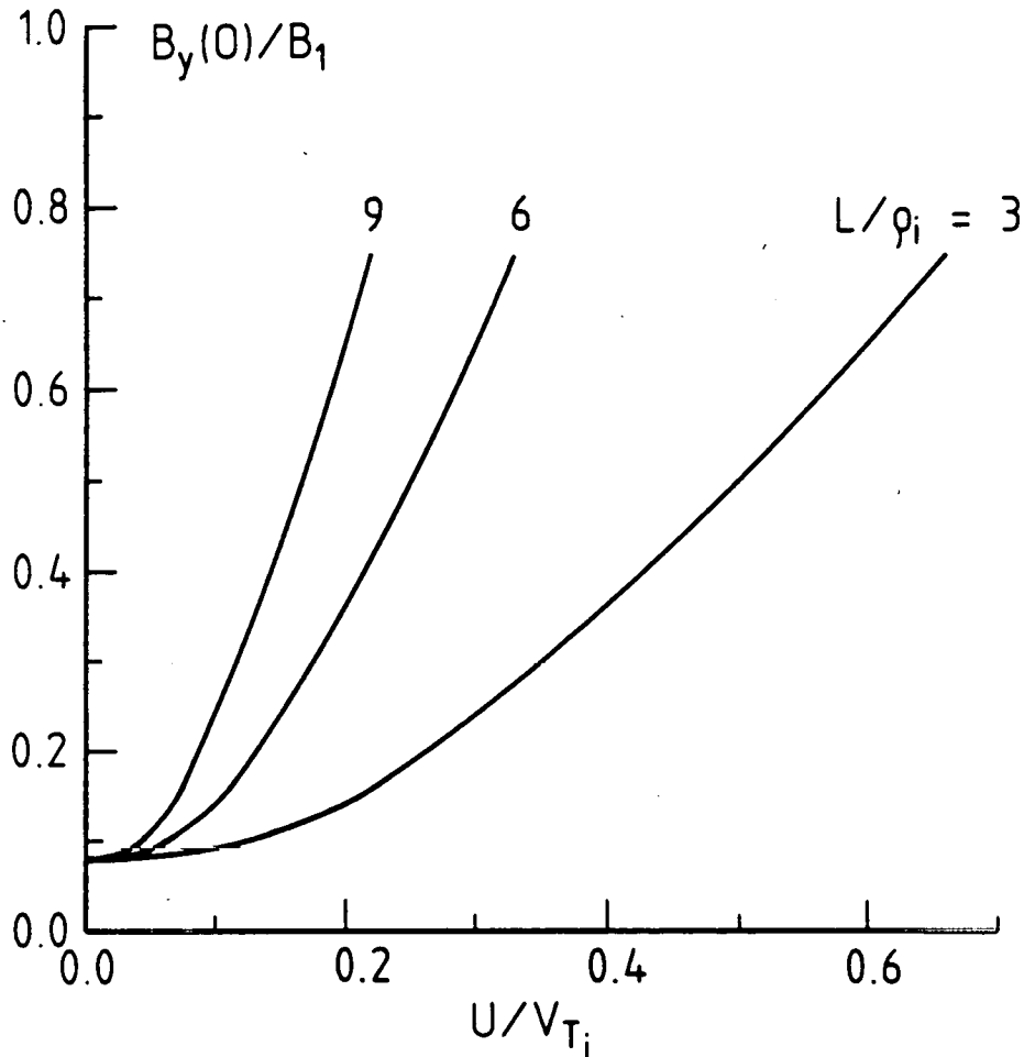
Figure 4: Dependence of the B_y component of the magnetic field at x = 0 (normalized on B_1 ) on the shear flow U (normalized on V_{Ti} ) for different values of the MCL thickness, while keeping the value of \theta_0 \approx 170^\circ . In this figure the thickness is measured in the ion Larmor radius and is expressed in terms of the parameter L of the Harris model by using the relation L/\rho_i \approx 2D/\rho_i (see equation (11) for the case where the asymptotic fields are nearly antiparallel). It can be seen that decreasing the value of the shear flow can lead to the same intensity of the B_y component at x = 0 , provided the thickness is increased.
