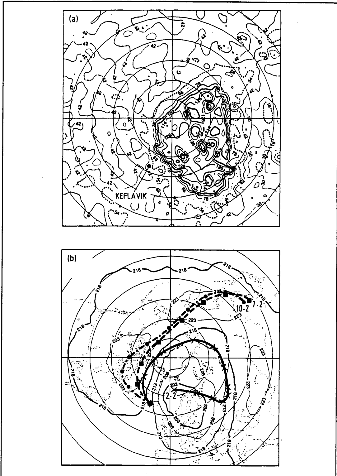
Fig. 3 (a) ECMWF potential vorticity analysis on the 550 K isentropic surface for February 7, 1992. The position of Keflavik is marked by a black point. (b) Temperature analysis on the same level and for the same day, together with trajectories for stratospheric air at 550 K arriving over Iceland on the date shown.
