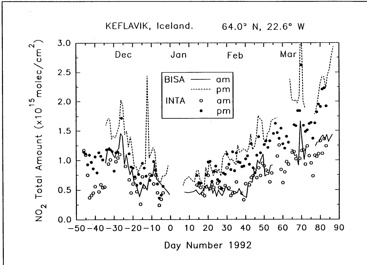
Fig. 1 Sunrise and sunset observations of NO 2 column amounts at Keflavik (Iceland) during EASOE, with INTA and BISA UV-visible ground-based spectrometers.
