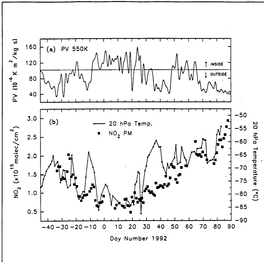
Fig. 2 (a) Potential vorticity evolution at the 550 K isentropic level. The dotted line indicates the boundary of the polar vortex. (b) Sunset \text{NO}_2 column amounts (BISA data) together with temperature at 20 hPa.
