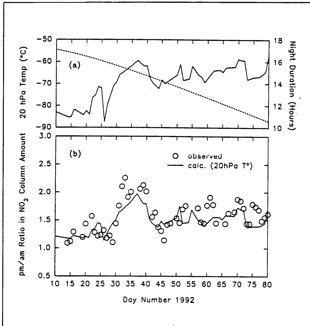
Fig. 4 (a) Temperature at 20 hPa (solid line) together with calculated night duration at the same level. (b) Observed nighttime decays in \text{NO}_2 column amount (3 day-running average, INTA data) compared to calculated values obtained with given temperatures and night durations.
