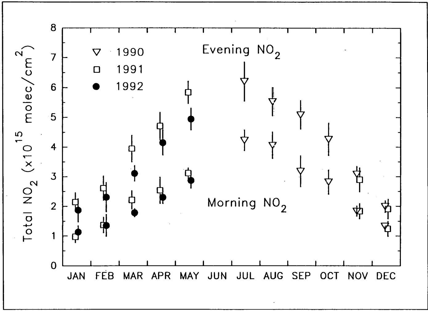
Fig. 2 Comparison of monthly mean NO 2 vertical abundances from measurements obtained at the Jungfraujoch (figure 1). The vertical bar represents the 1 sigma variability of the data during the considered month.
