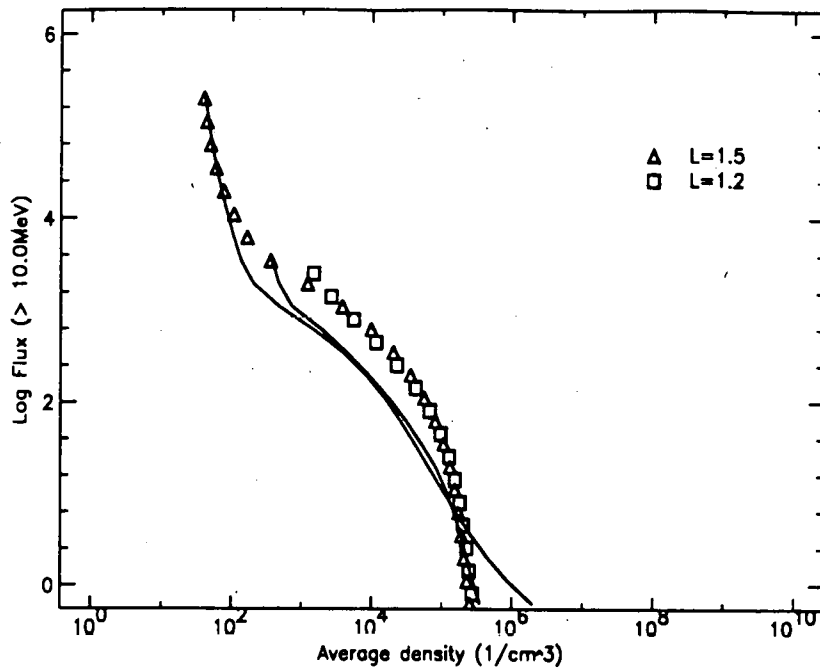
Figure 4. The integral AP-8 MIN/MAX proton flux above 10 MeV as a function of the drift shell average of the atmospheric density for low L -values. The symbols and lines have the same meaning as in Fig. 1.
