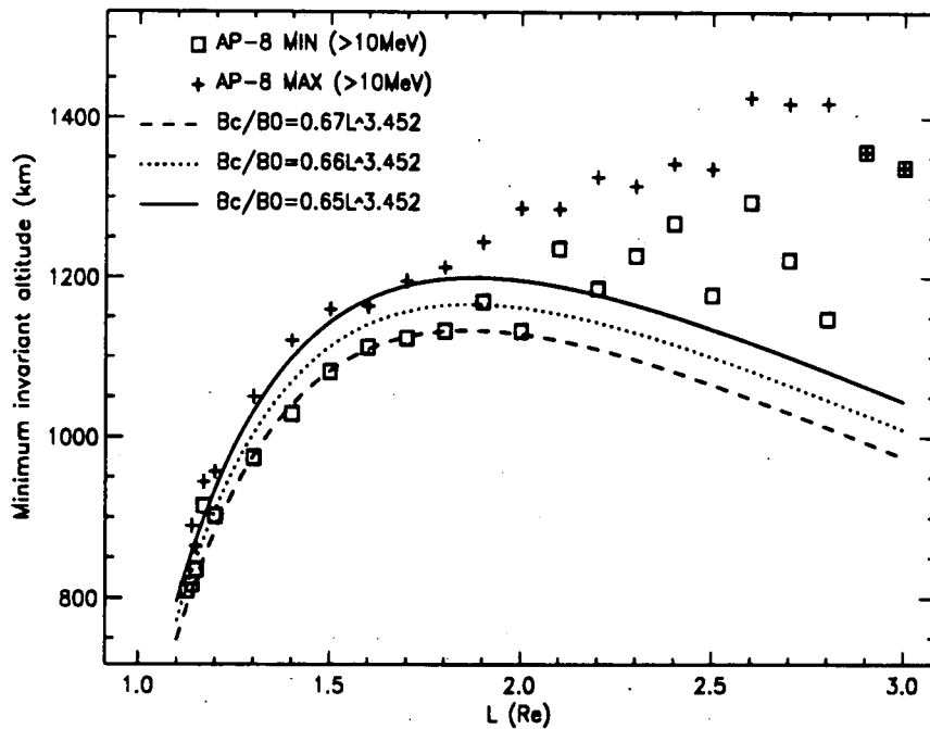
Figure 3. Invariant altitudes corresponding to the last B/B_0 value of the L blocks in AP-8 MAX (+) and AP-8 MIN ( \square ), for E > 10 MeV. The lines show the invariant altitude corresponding to three fits of B_c/B_0 .
