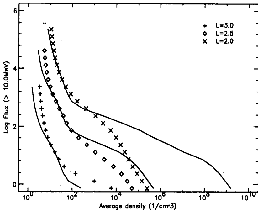
Figure 5. The integral AP-8 MIN/MAX proton flux above 10 MeV as a function of the drift shell average of the atmospheric density for higher L -values. The symbols and lines have the same meaning as in Fig. 1.
