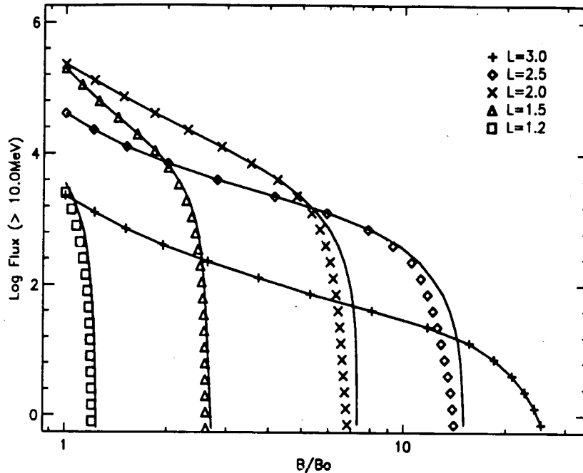
Figure 1. The integral AP-8 MIN/MAX proton flux above 10 MeV as a function of B/B_0 for selected L -values. The symbols denote AP-8 MAX values, the AP-8 MIN values are represented by the solid lines.
