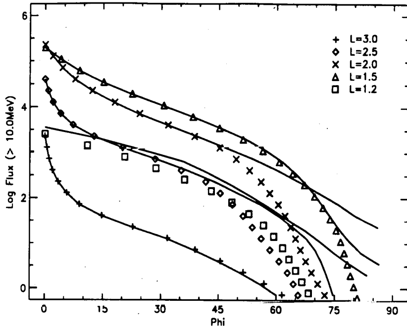
Figure 2. The integral AP-8 MIN/MAX proton flux above 10 MeV as a function of \varphi for selected L -values. The symbols and lines have the same meaning as in Fig. 1.
