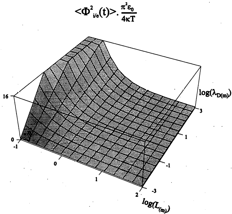
Figure 6. Normalized noise variance due to impacts and/or emissions of plasma particles, as a function of the antenna length and Debye length, for a fixed r_a=1 mm, T being constant.
