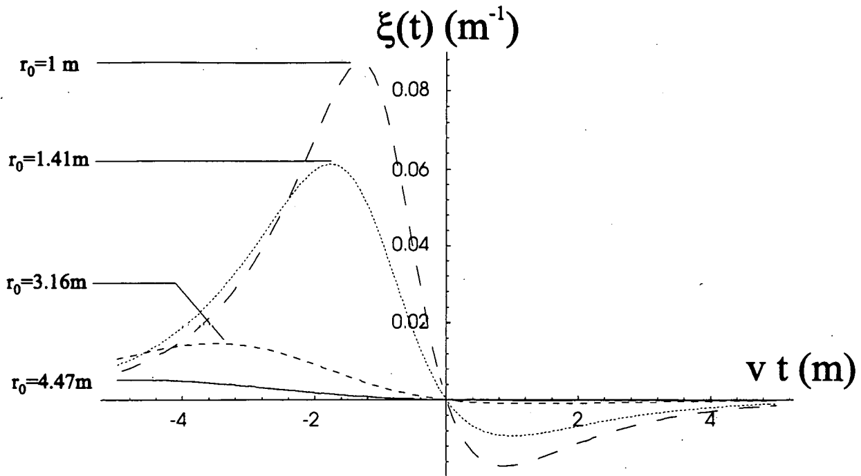
Figure 3e. Antenna response as a function of vt for different r_0 . Here \phi = -\pi/4 , \theta = \pi/4 , L = 10 \text{ m} , \lambda_d = 1 \text{ m} .
