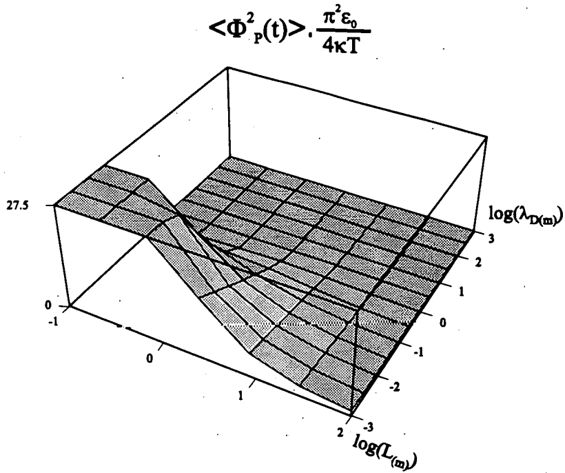
Figure 5. Normalized noise variance due to plasma particles flyby, as a function of the antenna length and Debye length, T being constant.
