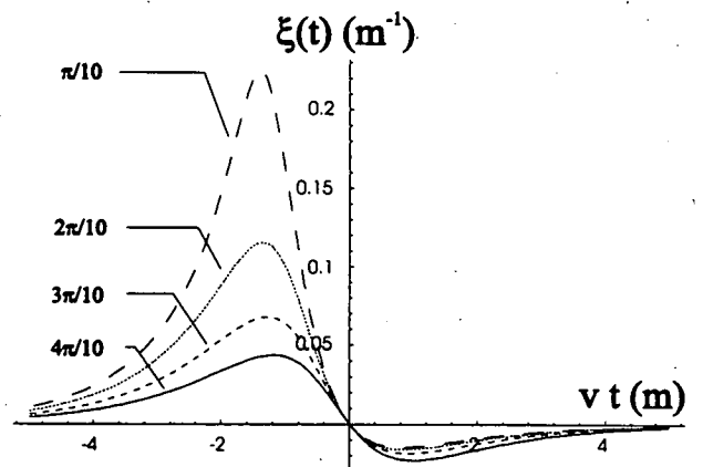
Figure 3d. Antenna response as a function of vt for different \varphi . Here r_0=1\text{m} , \theta=\pi/2 , L=10\text{m} , \lambda_d=1\text{m} .
