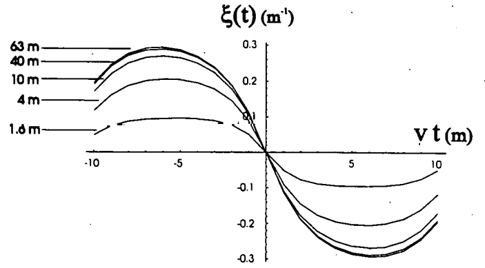
Figure 3b. Antenna response for a grain moving parallel to the antenna as a function of vt for different Debye lengths. Here r_0=1.41\text{m} , L=10\text{m} .
