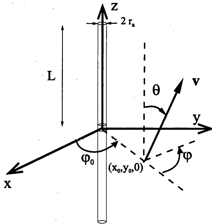
Figure 1. Antenna geometry of a wire dipole antenna and the coordinates used
