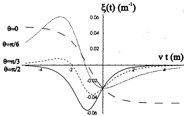
Figure 3c. Antenna response as a function of vt for different \theta . Here r_0=1.41\text{m} , \varphi=-\pi/4 , L=10\text{m} , \lambda_d=1\text{m} .
