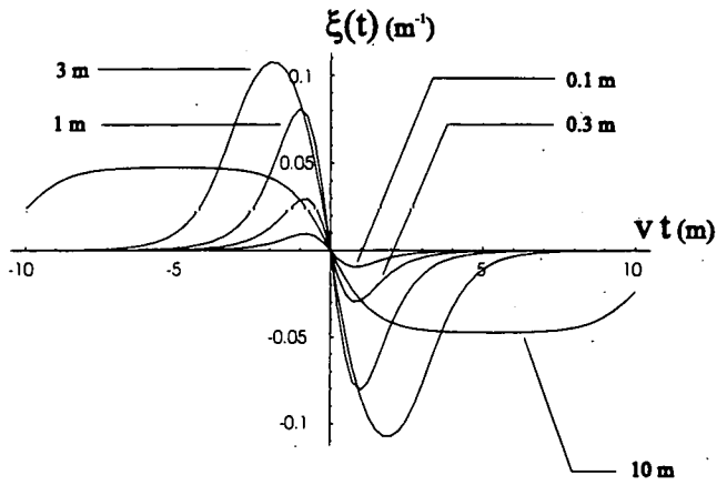
Figure 3a. Antenna response for a grain moving parallel to the antenna as a function of vt for different antenna lengths. Here r_0=1.41\text{m} , \lambda_d=1\text{m} .
