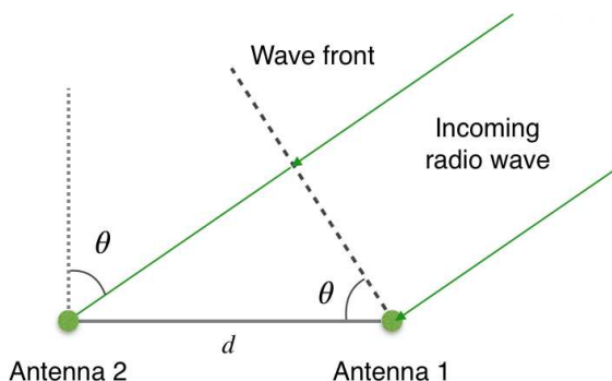
Figure 4 – Principles of two-element interferometer.
