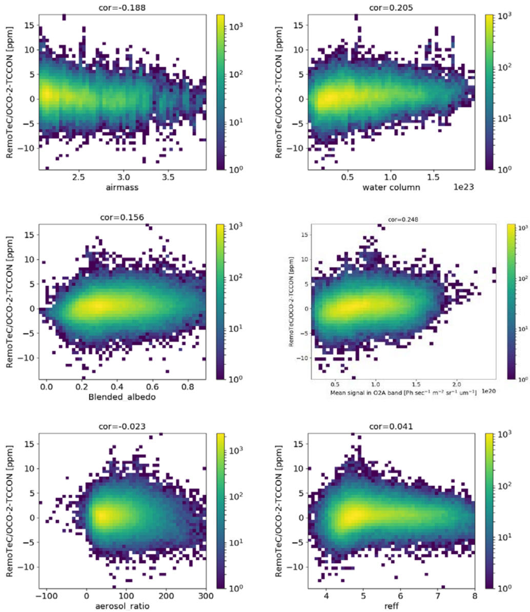
Figure S1. Error on XCO 2 retrievals as a function of six parameters: air mass, water column, blended albedo, mean signal in 5 O 2 A-band, aerosol ratio and aerosol size parameter (reff). Different colors represent the frequency of point occurrence.
