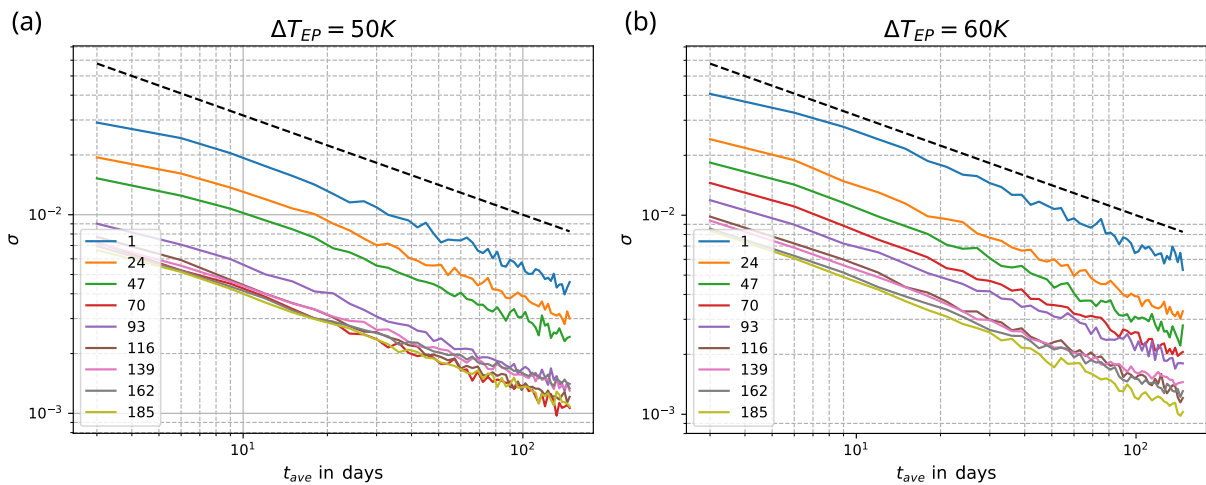
Figure A1. Standard deviation \sigma as a function of the block averaging length t_{ave} for different Lyapunov exponents of the PUMA model. The Lyapunov index is shown in the legend. Panel (a) shows the results for a temperature gradient \Delta T_{EP} of 50 K, panel (b) for 60 K. The black dashed line corresponds to t_{ave}^{-\frac{1}{2}} scaling.
