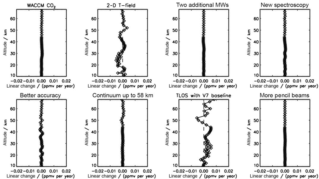
Figure 2. Sensitivity study: how different changes in retrieval setup affect the ozone retrieval. For each change, we show the linear term of differences of ozone retrieved from v7 spectra, using the new retrieval setup and the previous retrieval setup. Each panel corresponds to a retrieval setting for which only one parameter (which is stated in the title of the panel) is changed, and all other parameters remain unchanged.
