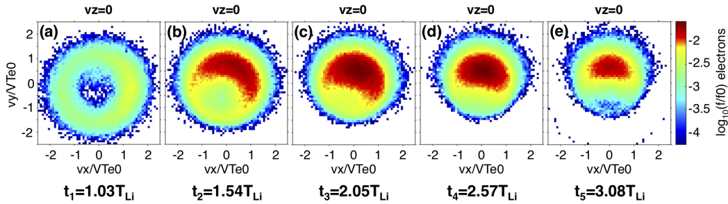
Figure 5. Virtual time series of five electron VDFs “measured” by a virtual satellite launched into the simulation domain. We illustrate the space of perpendicular velocities for v_z = 0 . The colour scale used is logarithmic.
