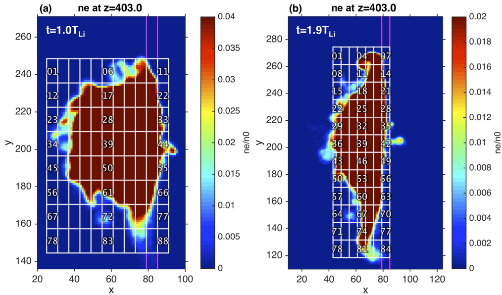
Figure A1. Electron number density for the z = 403 cross section together with the entire spatial grid used to calculate the electron velocity distribution functions, at (a) t = 1T_{Li} and (b) t = 1.9T_{Li} . There are 88 spatial bins in panel (a) and 84 in (b).
