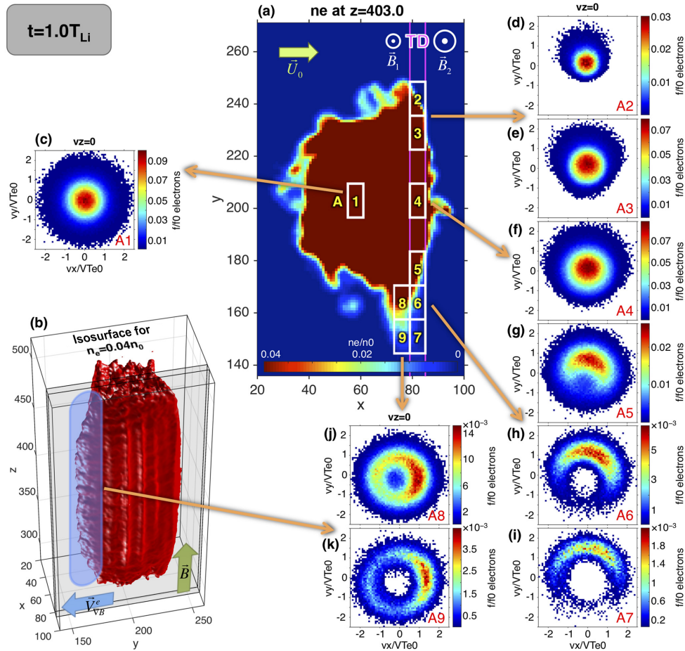
Figure 2. Snapshot of 3-D PIC simulation at t = 1T_{Li} (phase A). (a) Electron number density in the xOy plane for z = 403 . (b) The 3-D density isosurface for n_e = 0.04n_0 . (c–k) Electron VDFs in the space of perpendicular velocities for the spatial bins shown with white rectangles in panel (a). The two magenta lines mark the TD's boundaries.
