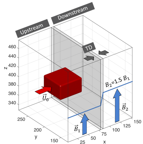
Figure 1. Schematic diagram of the simulation set-up. The high-speed plasma jet (shown by the red 3-D box) moves from the upstream region towards a parallel tangential discontinuity. The spatial profile of the background magnetic field is shown in blue. The tangential discontinuity is located between x_1 = 79 and x_2 = 85 .
