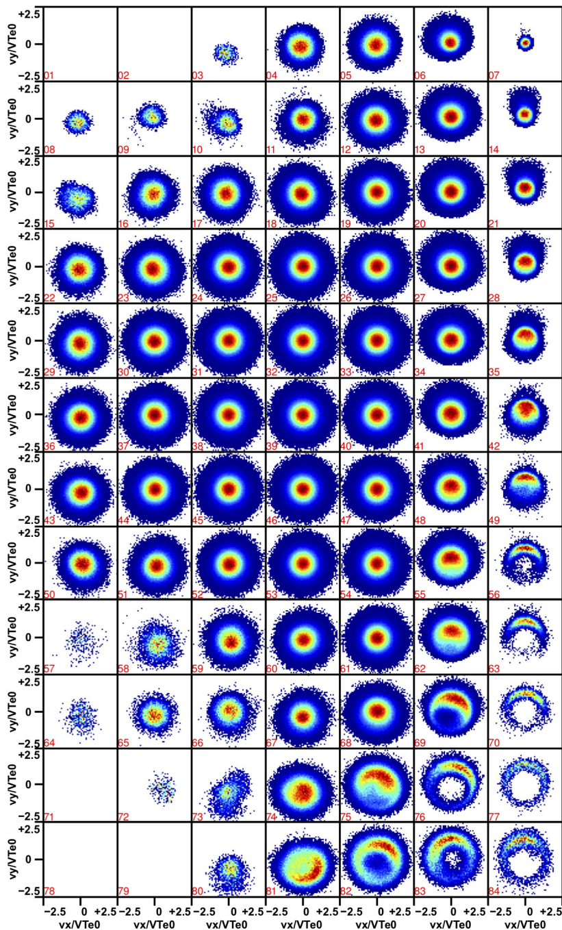
Figure A3. Electron VDFs, at t = 1.9T_{Li} , for each of the 84 spatial bins defined in Fig. A1b. We show v_z = 0 cross sections. The nine VDFs presented in Fig. 3 of the article correspond to bins 39, 6, 13, 41, 69, 76, 83, 75 and 82.
