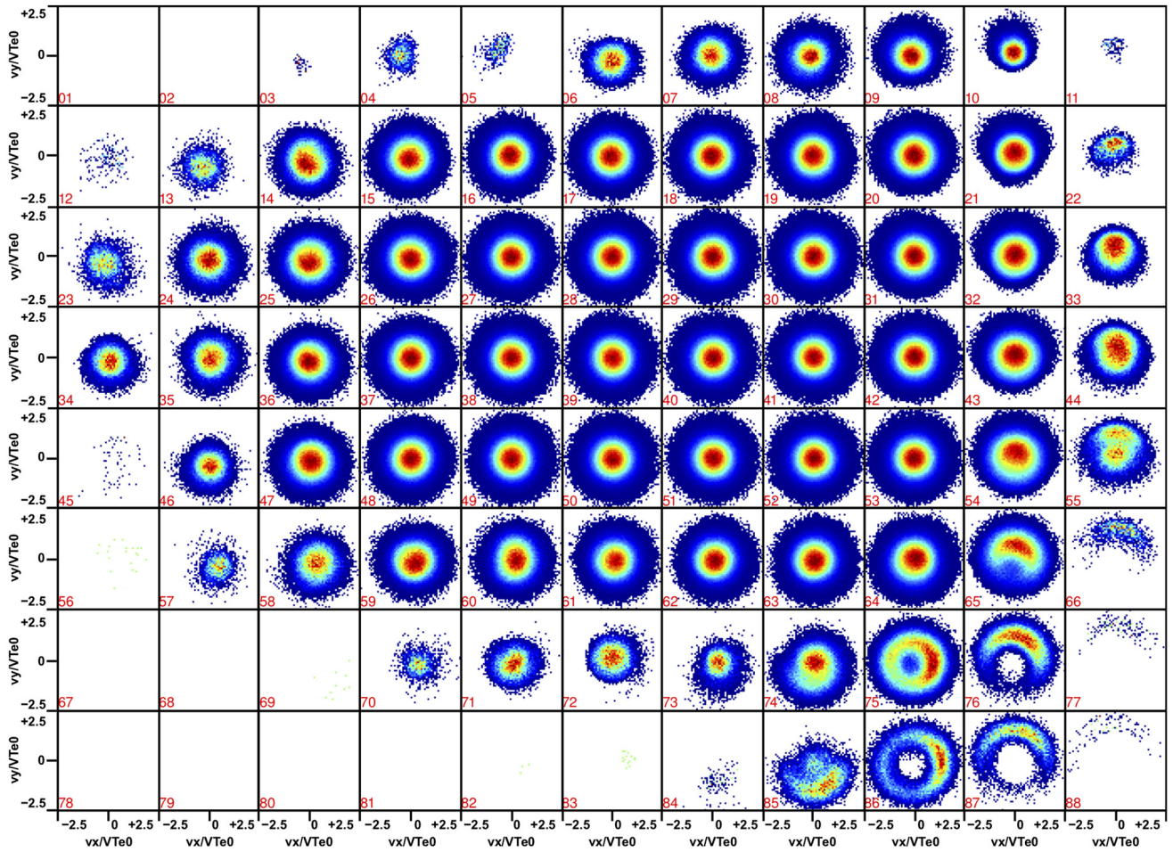
Figure A2. Electron VDFs, at t = 1T_{Li} , for each of the 88 spatial bins defined in Fig. A1a. We show v_z = 0 cross sections. The nine VDFs presented in Fig. 2 of the article correspond to bins 39, 10, 21, 43, 65, 76, 87, 75 and 86.
