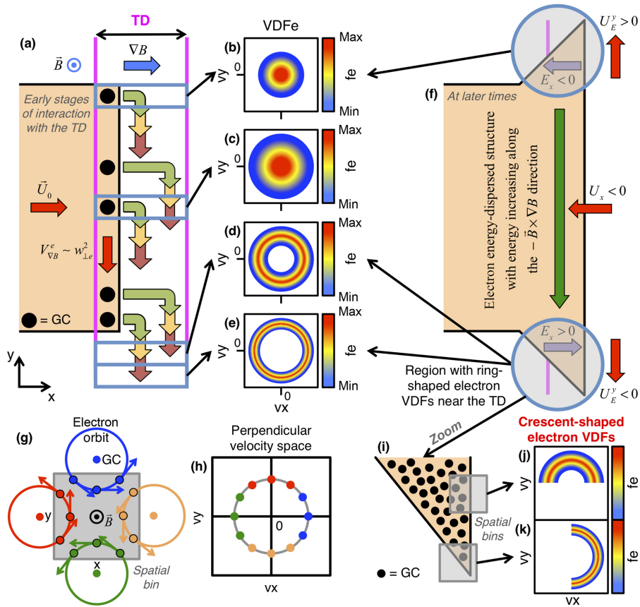
Figure 4. Panel (a) illustrates the phase A of plasma jet’s interaction with the magnetic discontinuity. The black dots indicate the guiding centres (GCs) of electrons localized at the front edge. The multiple groups of green–yellow–red arrows show the gradient-B drift displacement of the GCs proportional to the gyration energy (green corresponds to the lowest energy). The four blue boxes indicate the bins where the VDF is computed. The electron VDFs obtained for the upper edge bins (b, c) are gyrotropic and their phase density vanishes for large velocities; the VDFs obtained for the bottom edge bins (d, e) are ring-shaped. Panels (g) and (h) illustrate how the electrons with GCs outside a spatial bin contribute to different sectors of the VDF collected in the respective bin. The colours of the dots in panel (h) identify which particle shown in panel (g) contributes to that sector of the VDF. This effect corresponds to a remote sensing of the large Larmor radius electrons outside the bin. Panels (f) and (i)–(k) show how the remote sensing effect contributes to the formation of crescent-shaped VDFs in a configuration similar to the PIC simulations.
