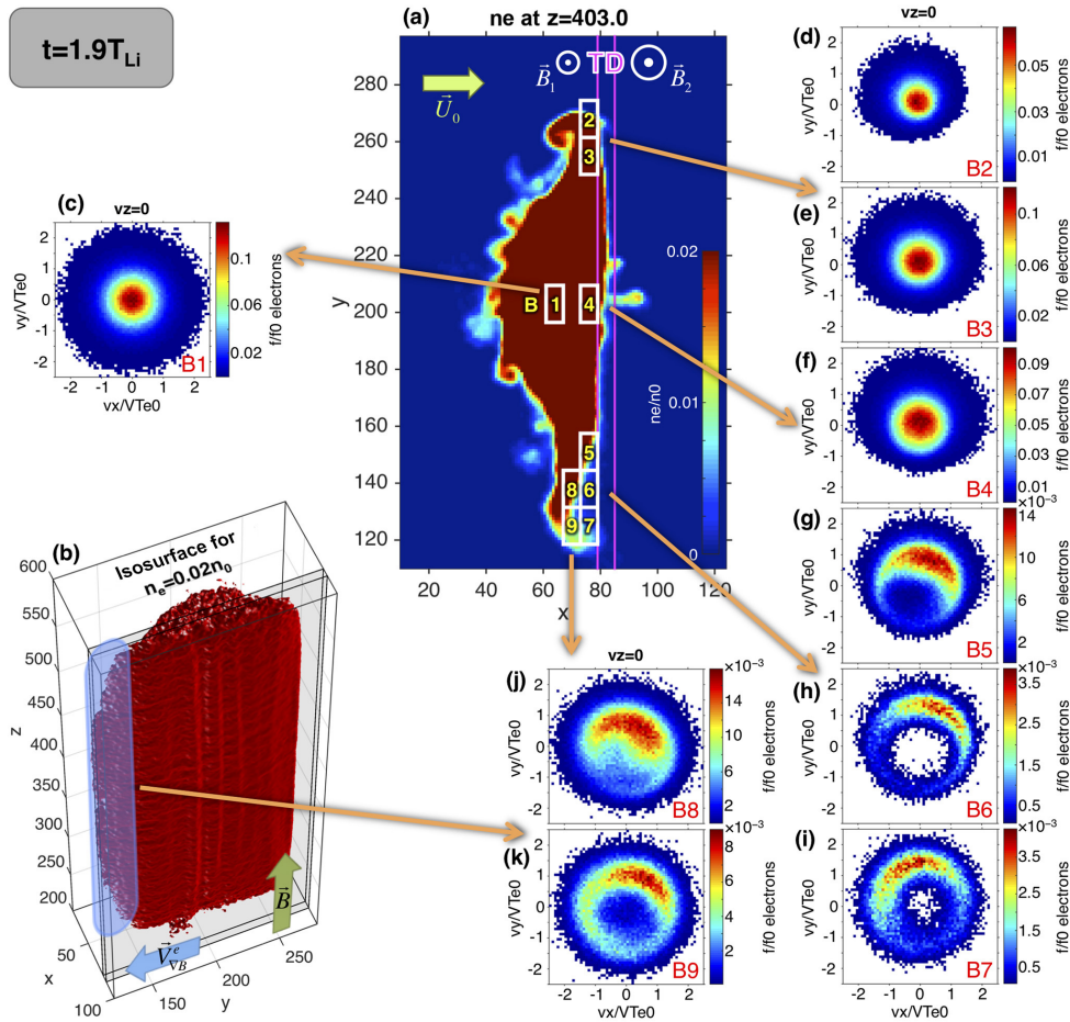
Figure 3. Snapshot of 3-D PIC simulation at t = 1.9T_{Li} (phase B). (a) Electron number density in the xOy plane for z = 403 . (b) The 3-D density isosurface for n_e = 0.02n_0 . (c–k) Electron VDFs in the space of perpendicular velocities for the spatial bins shown with white rectangles in panel (a). The two magenta lines mark the TD’s boundaries.
