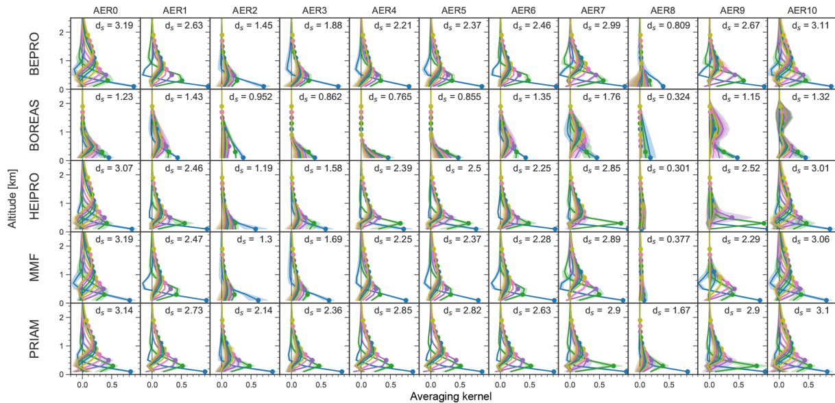
Figure 5. The 360 nm aerosol AVKs. Each subplot shows the mean AVK over all SZAs and RAA for a specific aerosol scenario (columns) and retrieval algorithm (rows). Filled circles indicate the nominal altitude of the corresponding AVK plotted in the same colour. Colour-shaded areas (barely visible in most cases) indicate the standard deviation of the AVKs, i.e. the variation for different SZAs and RAA. Also shown are the DFS. AVKs stem from retrievals with noisy measurements ( \sqrt{1n} ).
