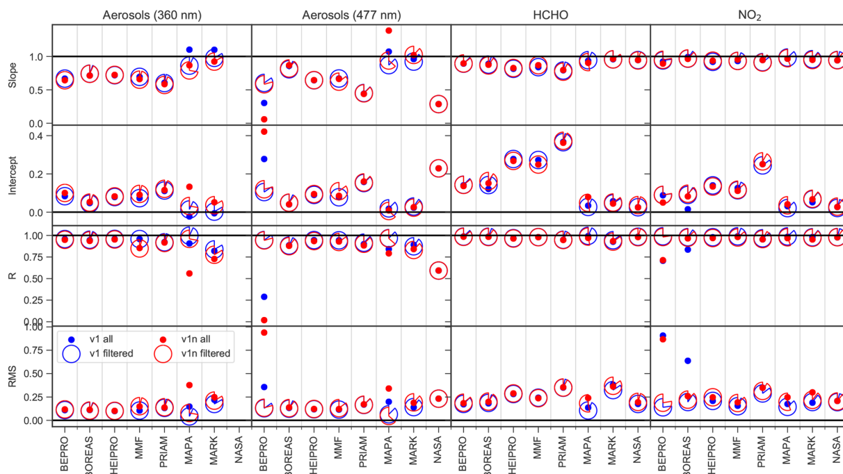
Figure 18. Slope, intercept, regression coefficient, and RMS for the correlation between true and retrieved aerosol as well as HCHO and NO 2 VCD. Intercept and RMS values are in dimensionless units for aerosols and 10^{16} molec cm -2 for HCHO and NO 2 . Cloud and fog scenarios (AER8, AER9, AER10) are excluded from the regression analysis.
