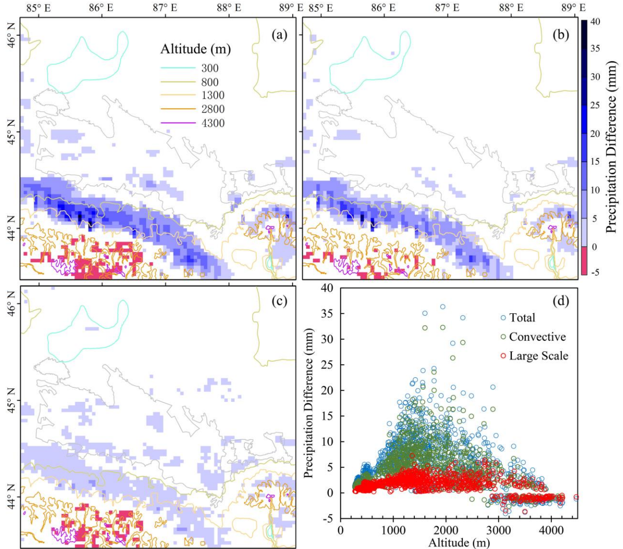
Fig. 3. The averaged summer precipitation during the period 1981-2016 computed from the difference CTL-NO_OASIS (a) total, (b) convective, (c) large scale. (d) The precipitation difference CTL-NO_OASIS as a function of the elevation in each grid point where a statistically significant difference is found. Only grid point with a statistically significant change ( p < 0.001 ) are shown in the (a), (b) and (c) plots.
