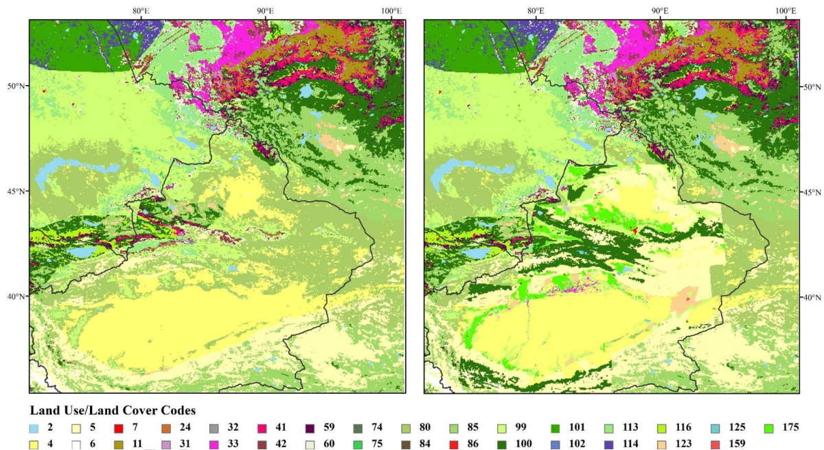
Fig. 2. The default land cover data from ECOCLIMAP (a) and the updated land cover data using the XIEG land cover database (b).
