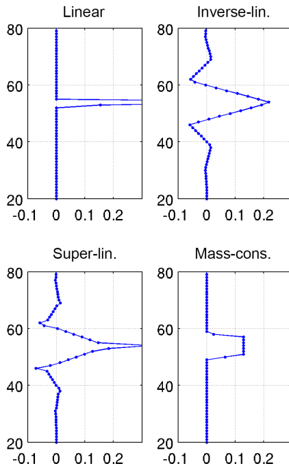
Figure 2. Regridding window functions for the four vertical sampling matching operations discussed in Sect. 4.1.2, going from a fine grid (0 to 100 in steps of one) to a coarse grid (0 to 100 in steps of 100/13) that only overlaps at the vertical edges (a.u.). The seventh row of each regridding matrix with dimension 14 \times 101 is plotted (columns 20 to 80 only). For pseudo-inverse and super-linear regridding these matrix elements are never zero, but of the order of 10^{-6} at the edges.
