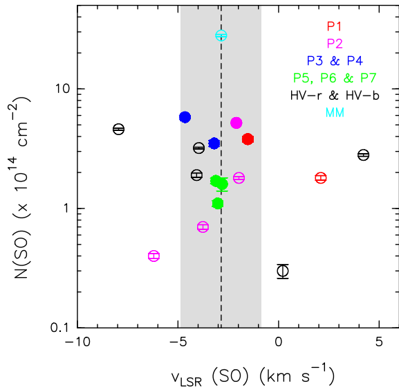
Figure 7. SO column density versus SO velocity towards the different positions in the AFGL 5142 field studied in this work. The filled/empty circles indicate detections/non-detections of PN. The different colours denote different groups of positions, as labelled in the upper right corner. The uncertainties on the column densities are indicated with error bars. The uncertainties on the velocities are within the size of the symbols. The systemic velocity of the central core, -2.85 \text{ km s}^{-1} , is indicated with a vertical dashed line. The grey band indicates a velocity range of \pm 2 \text{ km s}^{-1} with respect to the systemic velocity, which contains all the regions with PN detections.
