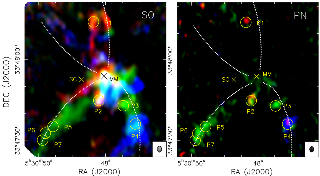
Figure 2. ALMA-integrated maps of SO( 2_3-1_2 ) (left) and PN( 2-1 ) (right) in three velocity ranges: [-6.5, -4.5] \text{km s}^{-1} (blue), [-4.5, -2.0] \text{km s}^{-1} (green), and [-2.0, 0] \text{km s}^{-1} (red). The cavity of the bipolar outflow is indicated with dashed white curves. The positions of the SC and the MM core are indicated with yellow (or black) crosses. The different P-spots (P1–P7) are identified with yellow circles. The beams of the observations are indicated in the lower right corner of each panel.
