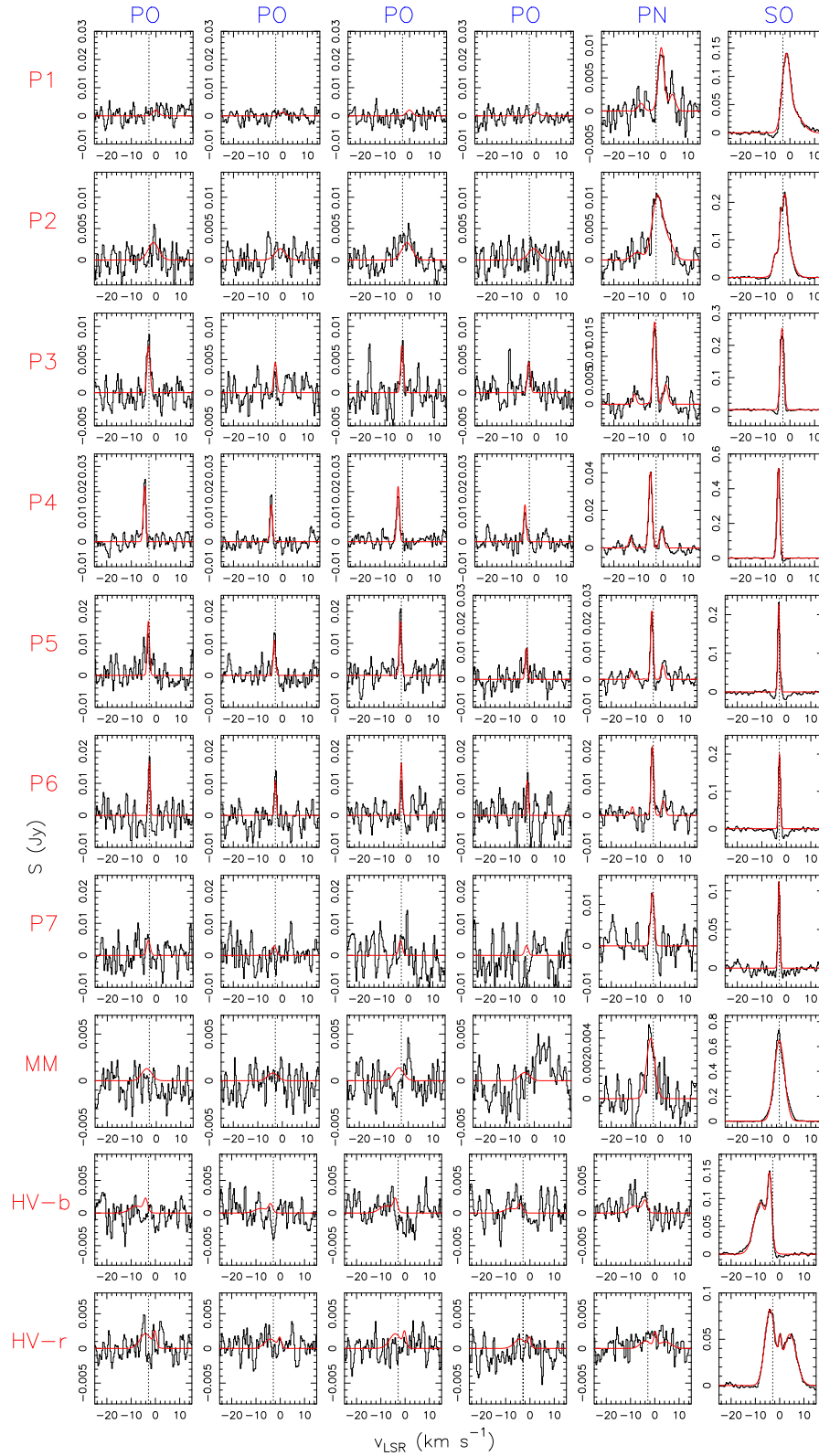
Figure 4. ALMA spectra of PO, PN, and SO (molecular transitions listed in Table 1) towards different positions of the AFGL 5142 star-forming region, indicated to the left of the panels. The dashed vertical lines indicate the systemic velocity of the central core, -2.85 \text{ km s}^{-1} . The red lines are local thermodynamic equilibrium (LTE) fits to the data obtained as explained in the text.
