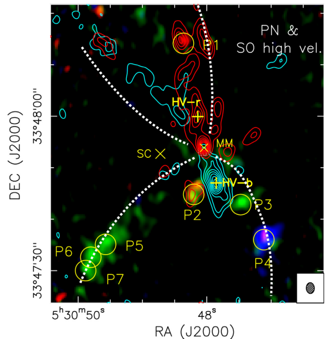
Figure 3. ALMA-integrated PN( 2-1 ) emission map (in colours) as shown in the right-hand panel of Fig. 2, with the high-velocity SO emission (in contours) shown in Fig. 1(b) overlaid. The positions of the SC and the MM core are indicated with yellow crosses. The different P-spots (P1–P7) are identified with yellow circles. The positions of the high-velocity spots HV-r and HV-b are indicated with yellow plus signs. The cavity of the bipolar outflow is indicated with dashed white curves.
