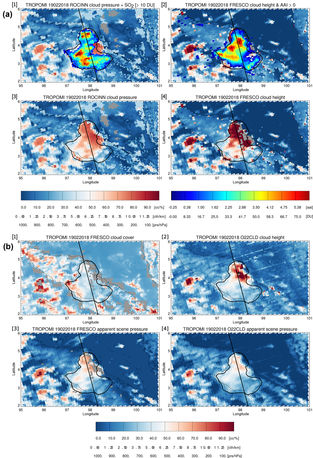
Figure 1. (a) TROPOMI cloud pressure (ROCINN; a1 and 3 ) and TROPOMI FRESKO cloud heights ( a2 and 4 ). TROPOMI SO 2 ( a1 ) and the AAI ( a2 ) for the overpass of the 19 February 2018 Sinabung eruption. The straight line denotes the path of the CALIPSO overpass, the solid-line shape denotes the outline of > 10 DU SO 2 columns, and the dotted-line shape denotes the AAI > 0 value. Note that for FRESKO and ROCINN cloud heights certain pixels are greyed out (“no data”), related to yet-unresolved retrieval artifacts. (b) As in (a) but for TROPOMI FRESKO cloud cover ( b1 ), O22CLD cloud height ( b2 ), FRESKO apparent scene pressure ( b3 ), and O22CLD apparent scene pressure ( b4 ). cc is cloud cover, cth is cloud top height, and prs is cloud pressure and scene pressure.
