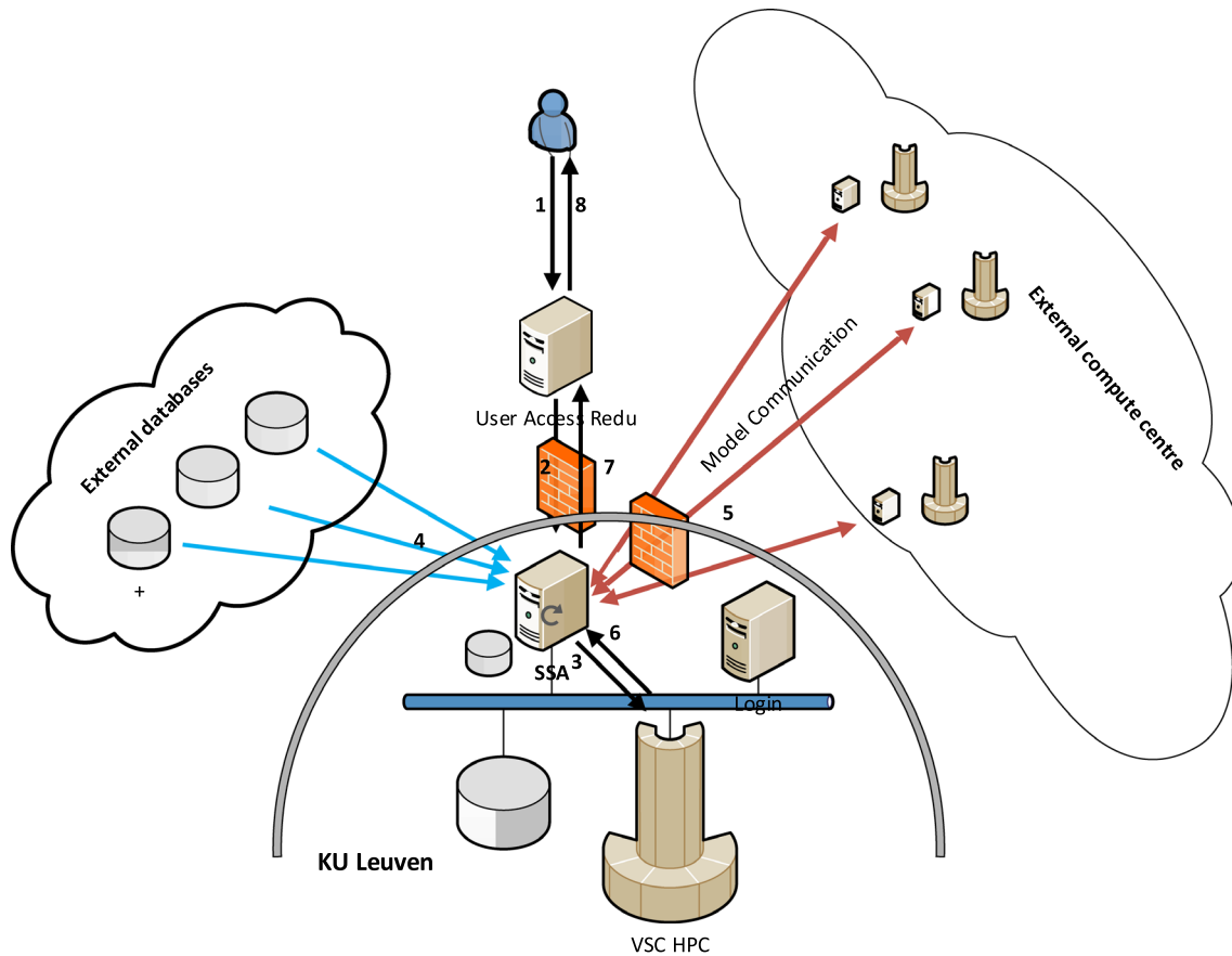
Fig. 1. Basic set-up of the federated VSWMC-P2 service with geographically distributed system elements.
