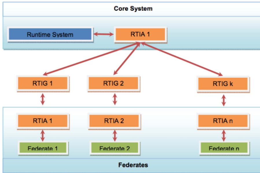
Fig. 4. RTI gateways (RTIGs) manage the simulations and transfers messages between federates. The VSWMC-P2 system supports multiple RTIGs to tackle high communication loads.
