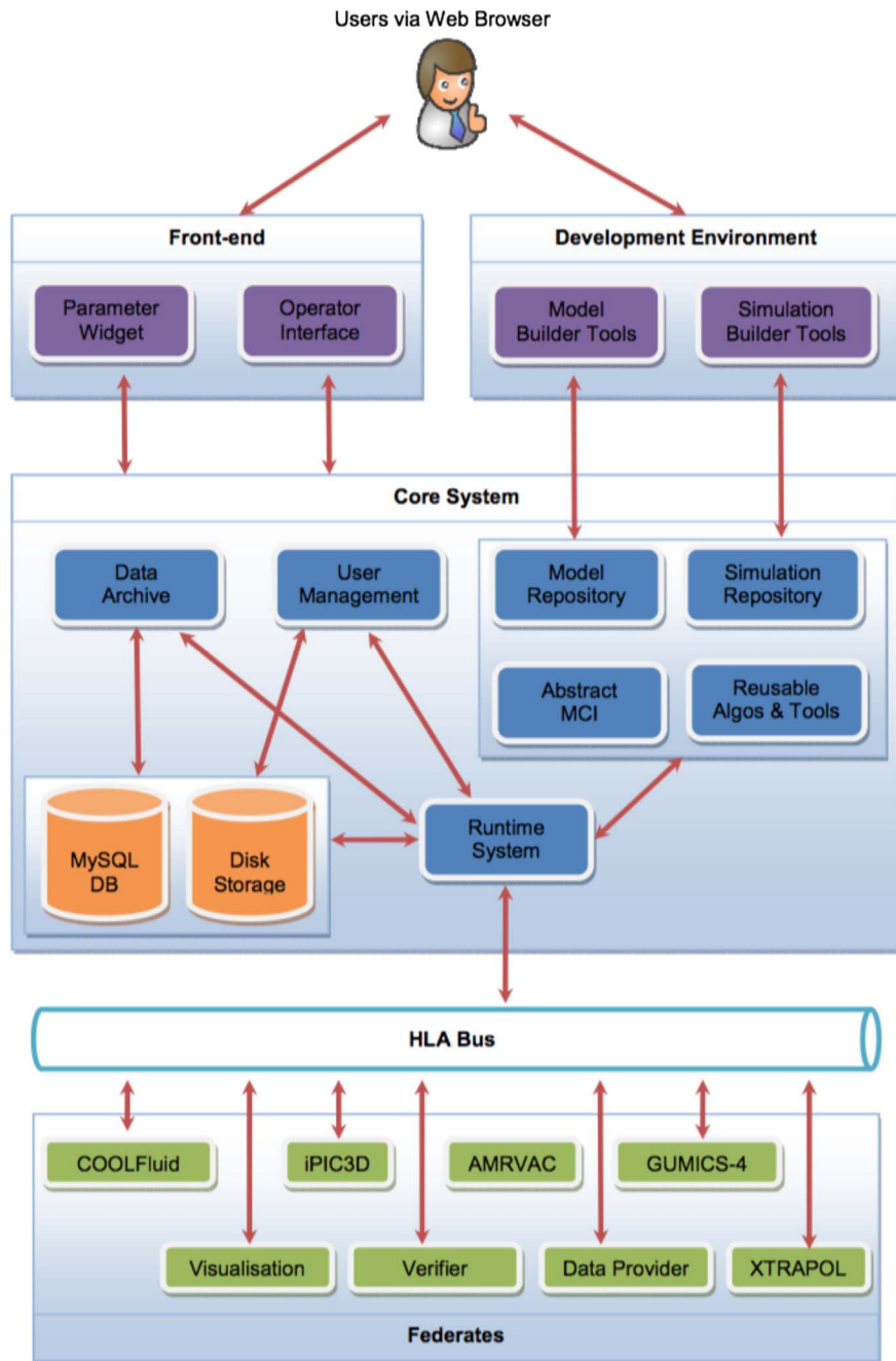
Fig. 2. VSWMC-P2 system requirements overview.
