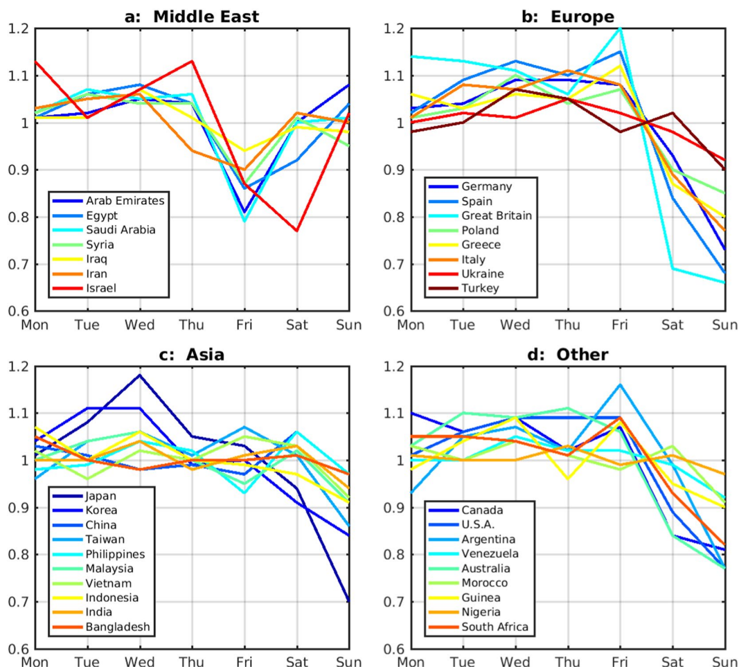
Figure 2. Mean normalised OMI NO 2 weekly profiles averaged over all studied cities in countries of (a) the Middle East, (b) Europe, (c) Asia, and (d) countries in the Americas, Africa and Australia (cf. Supplementary Table S3).
