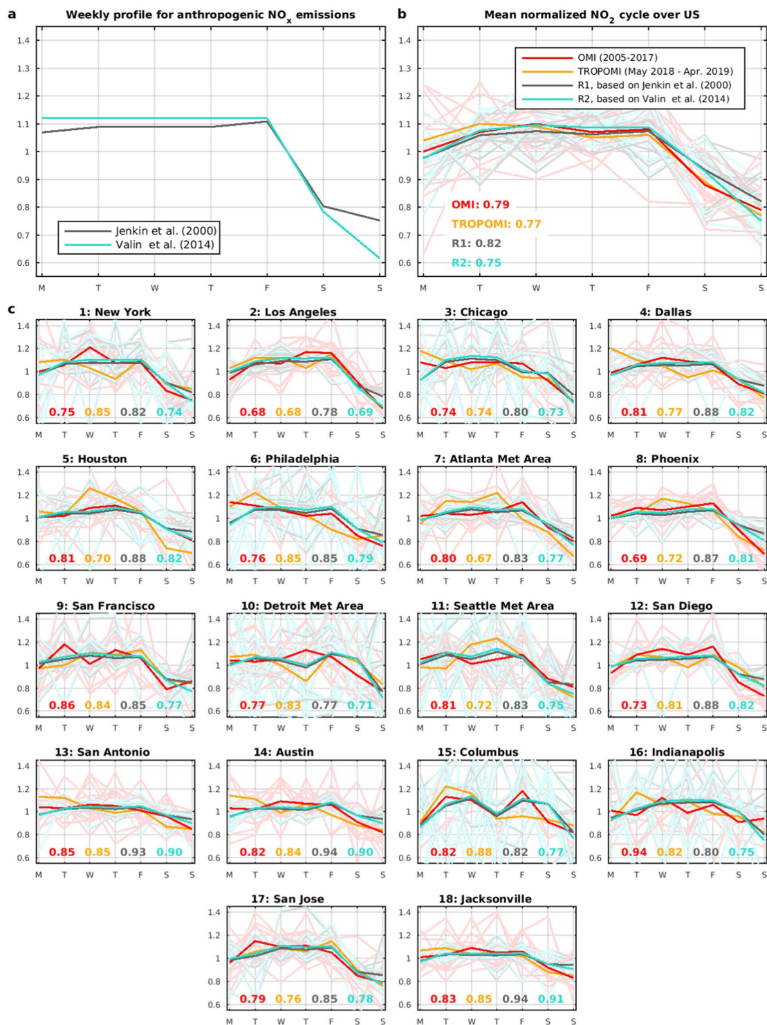
Figure 4. (a) Normalised weekly profiles of anthropogenic NO x emissions over the U.S. used in simulations R1 and R2. (b) Mean normalised weekly NO 2 cycle for all U.S. cities (weighted by population) from OMI (2005–2017, red) and TROPOMI (orange), and from model runs R1 (black) and R2 (light blue). Dark red line: average OMI cycle for 2005–2017; pale lines: individual years. The normalised column on Sunday is given inset. (c) Same as b for individual cities ranked according to the population of their urban areas ( en.wikipedia.org/wiki/List_of_United_States_urban_areas ).
