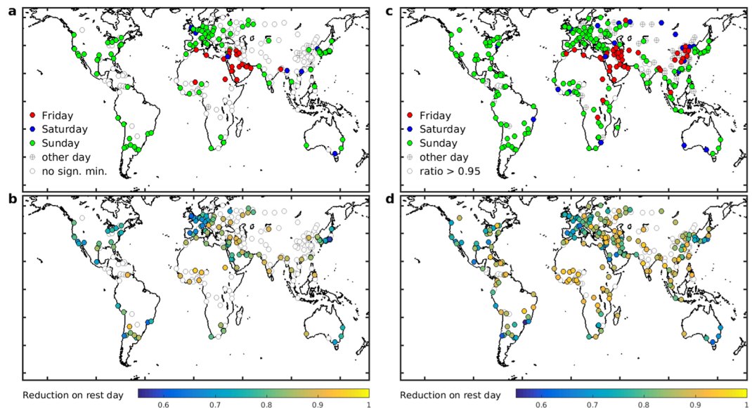
Figure 1. (a) Location of studied cities. The color indicates the day of minimum according to OMI \text{NO}_2 data over 2005–2017. Open circles indicate cities for which the OMI minimum is not significant (see text). (b) Normalised \text{NO}_2 column on the day of the minimum of OMI data. (c,d) Same as a and b for TROPOMI data over May 2018–April 2019. The numerical values of OMI and TROPOMI normalised columns are given in Supplementary Table S1. The map is generated using the shapefile landareas.shp from the mapping toolbox of MATLAB version R2013a (8.1.0.604), Natick, Massachusetts, The MathWorks Inc.
