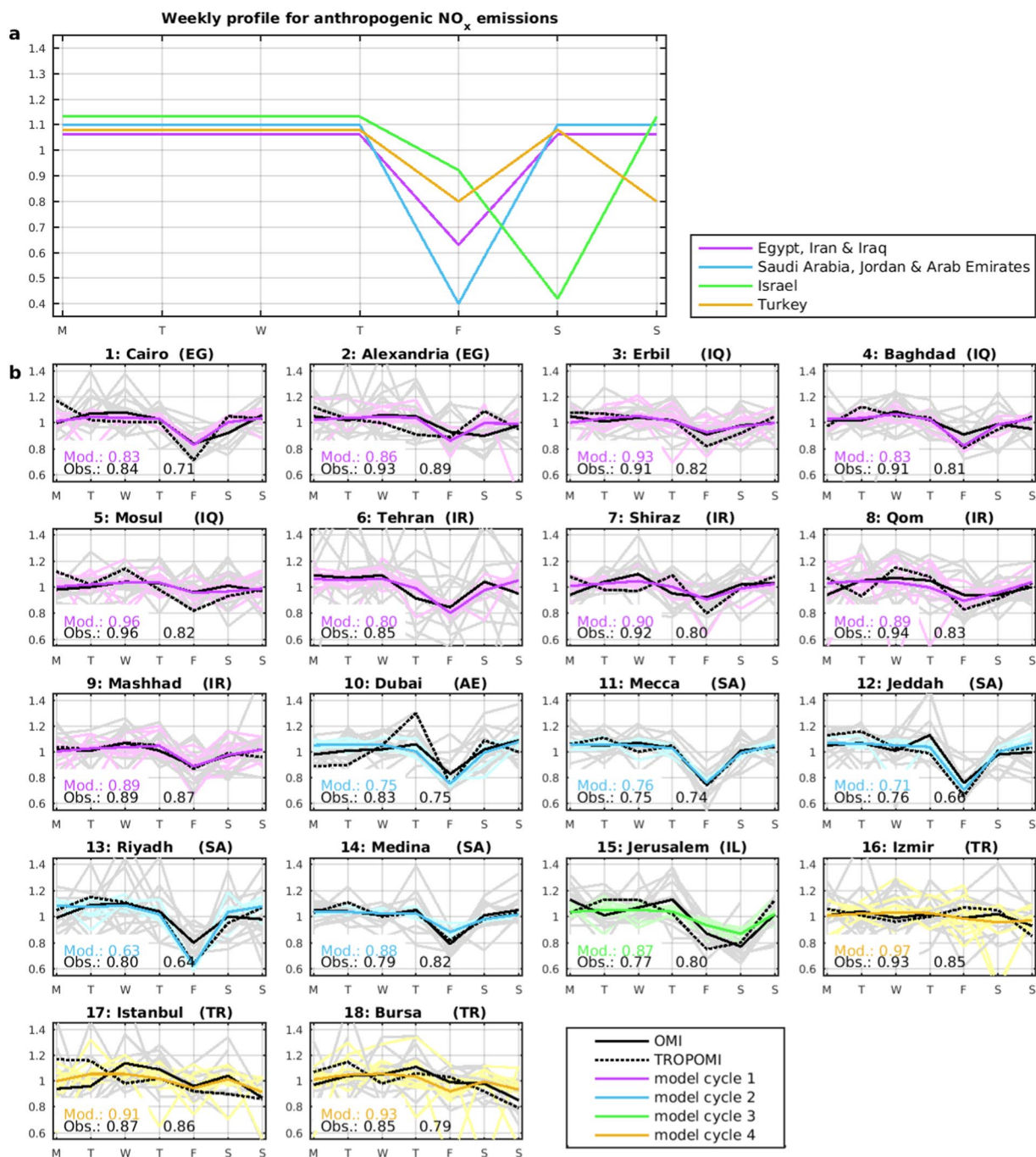
Figure 6. (a) Normalised weekly profiles of anthropogenic NO x emissions for Middle East countries used in the simulations (see main text). (b) Mean normalised weekly NO 2 cycle in Middle East cities observed by OMI (black), TROPOMI (dashed black) and predicted by the model (coloured lines). The model uses distinct weekly emission profiles for Egypt, Iran and Iraq (magenta), Arab Emirates, Jordan, and Saudi Arabia (blue), Israel (green), and Turkey (yellow). Thick black line: average OMI 2005–2017; thin grey lines: individual years. The day-of-minimum normalised column is given inset for the model, OMI, and TROPOMI.
