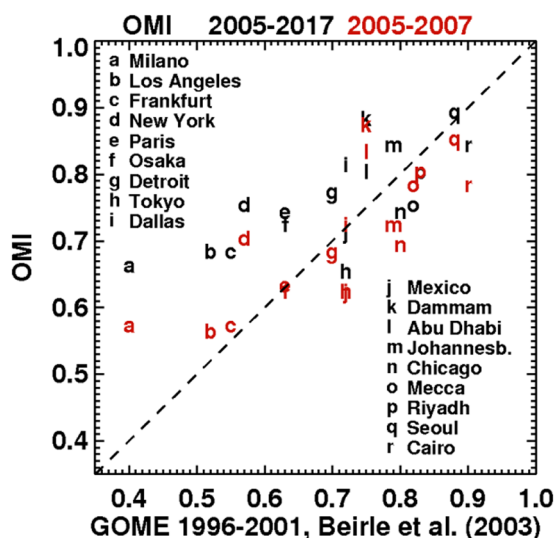
Figure 3. Column reduction during the rest day (Sunday or Friday) over 18 large cities reported in 6 based on GOME 1996–2001 data, and based on OMI data from either 2005–2017 (black) or 2005–2007 (red).
