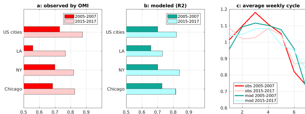
Figure 5. (a) Sunday-to-week column ratios averaged over 2005–2007 and over 2015–2017 for U.S. cities (average of 18 cities weighted by population), and for New York, Los Angeles and Chicago as observed by OMI. (b) Same for ratios calculated with the MAGRITTE model simulation R2. (c) Average observed and modelled weekly cycle for U.S. cities over 2005–2007 and 2015–2017.
