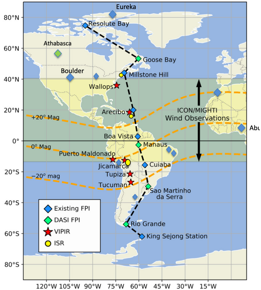
Figure 24: A proposed expansion plan for the Fabry-Perot Interferometer network in the American sector called Distributed Array of Small Instruments (DASI). If the IMCP can provide infrastructures at locations like Goose Bay, Rio Grande, and others, a complete chain can be implemented shortly. The geographical coverage of the ICON/MIGHTI wind observations is also indicated.
