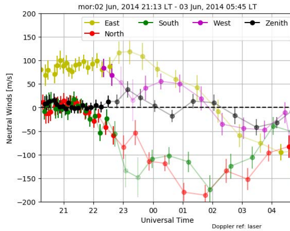
Figure 26: Wind components of the FPI look measurements; north, south, east, west and zenith during 02 June 2014
