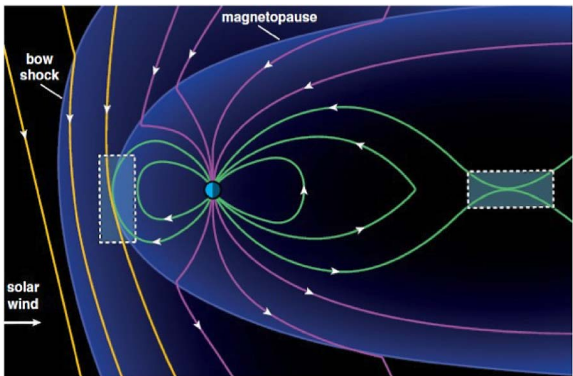
Figure 4: Illustration of the two main regions of magnetic reconnection in the Earth magnetosphere (magnetospheric "nose" on the dayside and tail plasmasheet center) by means of which energy coming from the solar wind is channelled into the inner magnetosphere and IMUA after temporary storage in the tail magnetic field configuration.
