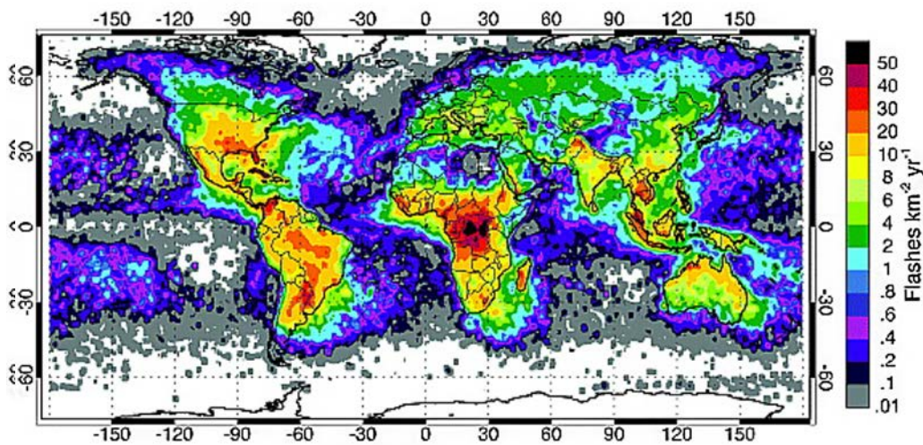
Figure 8: Annualized global distribution of lightning strokes over the globe, expressed in units of number of flashes per square km and per year, showing a pronounced maximum in equatorial Africa over Rwanda and the Democratic Republic of Congo, maximizing over the Rwandan city of Kamembe, and a strong land-to-oceans contrast. From Christian et al. (2003).
