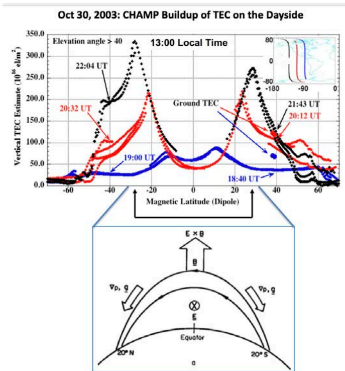
Figure 6: An example of an ionospheric Total Electron Content (TEC) perturbation produced on the equatorial ionospheric anomaly by the penetration of an eastward electric field from higher latitudes. Under the effect of the enhanced eastward electric field and upward drift applied to equatorial magnetic flux tubes, plasma is depleted at the equator and diffuses along magnetic field lines away from the equator (equatorial fountain effect), enhancing the TEC at latitudes of 15 to 40 degrees, as shown by CHAMP TEC data in the south-Atlantic anomaly region on three successive passes (blue, red and black).
