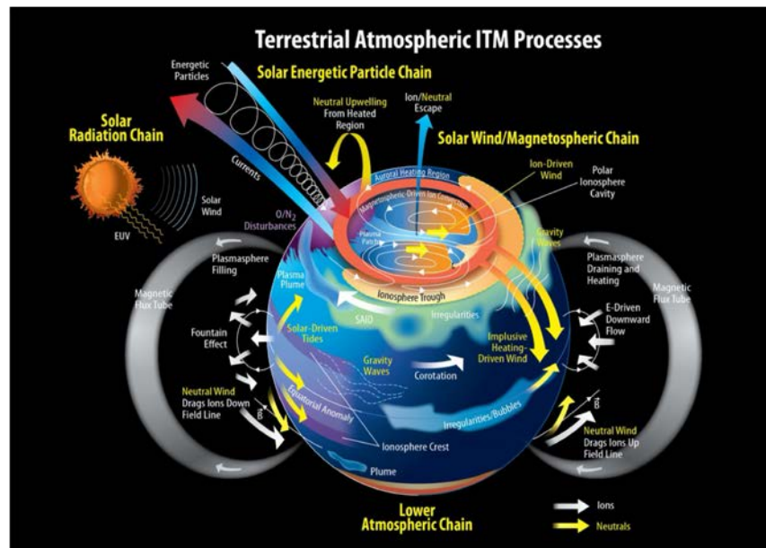
Figure 33: Cartoon illustrating the main processes that take place and are modeled in the coupled ionosphere-thermosphere-atmosphere system. Credits: NASA's Scientific Visualization Studio https://svs.gsfc.nasa.gov/4641 .
