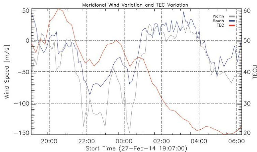
Figure 27: Total electron content (TEC) measured over Rabat (33.998°N, 6.854°W) and thermospheric meridional wind north- and south facing components, measured by the Fabry-Perotinterferometer (FPI) over Oukaimeden Observatory (31.206°N, 7.866°W; 22.84°N magnetic).
