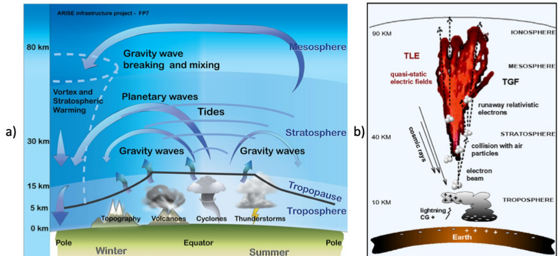
Figure 9: A schematic of the atmospheric dynamic processes encountered in the Earth's lower and middle atmosphere which lead to different types of wave emissions responsible for transfer of energy and momentum between atmospheric layers and between latitude regions: a) planetary waves, tides, gravity waves and infrasound waves (not shown in the figure) generated by topography, weather events and volcanoes transfer momentum and deposit energy by reflection, absorption and/or breaking (from E. Blanc et al. (2018), ARISE FP7 Infrastructure project of the European Union); b) thunderstorm clouds are responsible for the generation of different types of emissions into the IMUA: Transient Luminous Events (TLE), Transient Gamma Ray Flashes (TGFs) possibly triggered by upward-accelerated electron beams, ELF radio emissions penetrating into the ionosphere and interacting with radiation belts (not shown) (from Blanc E. et al., 2007)
