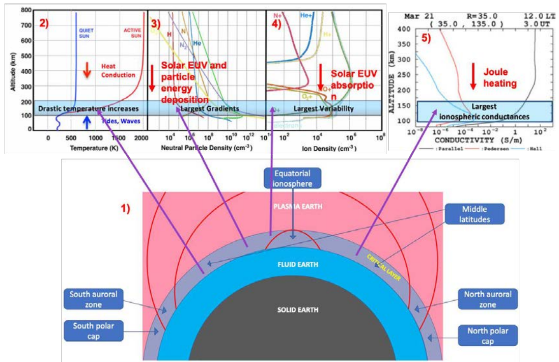
Figure 1: Distinguishing three “phase domains” in our geospace (1), e.g. Solid Earth (black), Fluid Earth (blue) and Plasma Earth (pink) shows that fluid Earth and Plasma Earth overlap over a thin shell extending approximately from 50 to 500 km surrounding our planet, which we call the Ionosphere-Middle-Upper-Atmosphere (IMUA), a critical transport layer within which hydrodynamics and electrodynamics are coupled. The unique transport properties of the IMUA make it an efficient “screen” on which to project and detect disturbances coming from above (the coupled Sun-Earth system) and from below (fluid and solid Earth) in our geospace: the IMUA is a region of heat conduction from above related to the strong upward exospheric temperature gradient (2), energy deposition by solar EUV and X-ray radiation and by precipitating particles (3,4) and maximum Joule heating by ionospheric electric currents (5).
