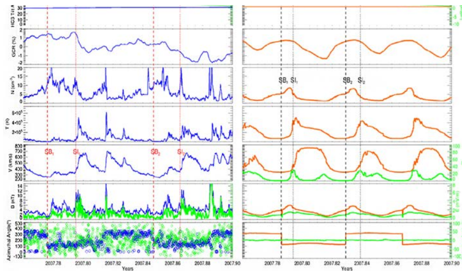
Figure 30: The 27-day periodic variations of 2 GV proton intensity and solar wind plasma properties (left: observations, right: simulations).
