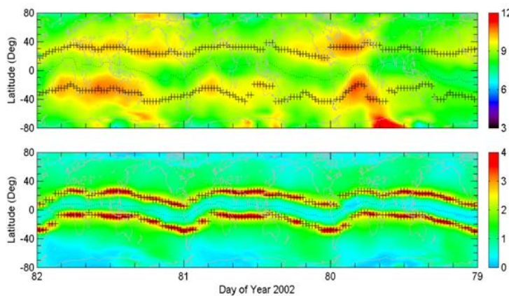
Figure 34: Simultaneous neutral mass density (top, 10^{12} \text{ kg/m}^3 ) and electron density (bottom, 10^{12} /\text{m}^3 ) measured by the CHAMP satellite at around 19 LT in Equinox (day 79-81 in 2002). The UT day runs from right to left. This plot demonstrates the coupling and decoupling features between the ionosphere and the thermosphere at low and middle latitudes and the modulation association with the lower atmosphere forcing (modified by Lei et al., 2010)
