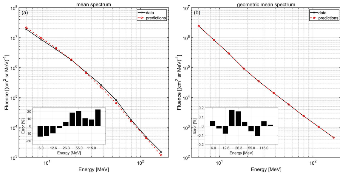
Fig. 11. Comparison of (a) mean spectra and (b) geometric mean spectra of Fluences from all Events in the SEPEM REL and all predicted Fluences in this work. Insets show percentage error at all energy bins.
