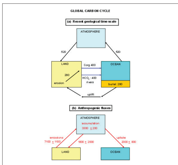
Figure 3.1 - The carbon cycle in recent geological time and its perturbation by human activities. All fluxes in Mt C/yr.
