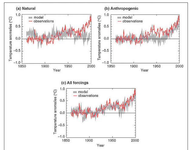
Figure 2.25 – Comparison between modelled and observed temperature rise since 1860. Simulating the earth's temperature variations (°C) and comparing the results with measured changes can provide insight to the underlying causes of major changes. A climate model can be used to simulate temperature changes due to both natural and anthropogenic causes. The simulations represented by the band in (a) were done with only natural forcings: solar variation and volcanic activity. Those encompassed by the band in (b) were done with anthropogenic forcings: greenhouse gases and an estimate of sulphate aerosols. Those encompassed by the band in (c) were done with both natural and anthropogenic forcings included. From (b), it can be seen that inclusion of anthropogenic forcings provides a plausible explanation for a substantial part of the observed temperature changes over the past century, but the best match with observations is obtained in (c), where both natural and anthropogenic factors are included. These results show that the forcings included are sufficient to explain observed changes, but they do not exclude the possibility that other forcings might also have contributed. (IPCC TAR - Climate Change 2001: The Scientific Basis).
