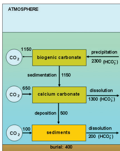
Figure 3.10 - Tentative global cycle of calcium carbonate in the marine system (all fluxes are given in Mt C/yr). The production of calcium carbonate in the euphotic zone and its dissolution in deeper water result in a downward transfer of bicarbonate ( \text{HCO}_3^- ) and an upward transfer of \text{CO}_2 . In order to maintain a steady state, the annual burial of 400 Mt C as \text{CaCO}_3 must be compensated by an equal release of C as \text{CO}_2 into the atmosphere. (R. Wollast, ULB-OCEAN).
