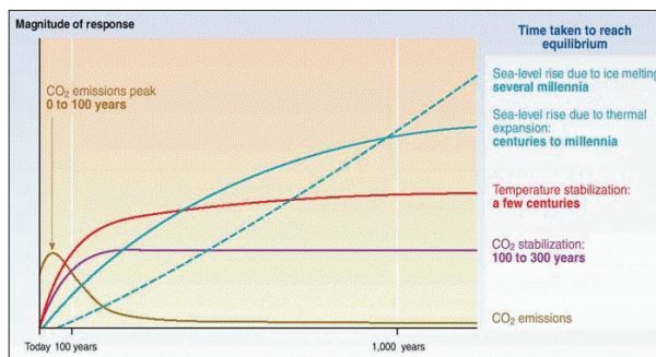
Figure 2.43 – \text{CO}_2 -concentration, temperature, and sea level continue to rise long after emissions are reduced. After \text{CO}_2 emissions are reduced and atmospheric concentrations stabilise, surface air temperature continues to rise slowly for a century or more. Thermal expansion of the ocean continues long after \text{CO}_2 emissions have been reduced, and melting of ice sheets continues to contribute to sea level rise for many centuries. This figure is a generic illustration for stabilisation at any level between 450 and 1,000 ppm, and therefore has no units on the response axis. Responses to stabilisation trajectories in this range show broadly similar time courses, but the impacts become progressively larger at higher concentrations of \text{CO}_2 . (IPCC TAR - Climate Change 2001: The Scientific Basis).
