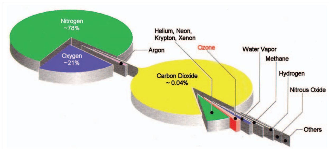
Figure 1.1 - Representation of the relative volume contributions of a series of gases present in the moderately dry earth's atmosphere. The major constituents, nitrogen (N 2 ) and oxygen (O 2 ), account together for about 99% of the total volume. The remaining 1% includes a number of rare, neutral gases and all other minor and trace constituents. Carbon dioxide (CO 2 ) accounts for slightly less than 0.04% by volume and ozone in the stratosphere is another 100 times less abundant. The main environmental preoccupations that have arisen over the past decades (e.g., the ozone layer thinning and climate alterations) thus result from anthropogenic perturbations of a very small fraction of the total atmosphere. (R. Zander, ULg-GIRPAS).
