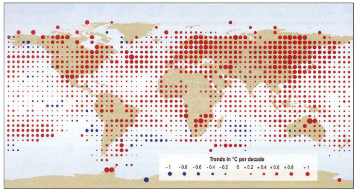
Figure 2.4 – Annual temperature trends: 1976-2000. Consistent, large-scale warming of both the land and ocean surfaces occurred over the last quarter of the 20 th century. (IPCC TAR - Climate Change 2001: Synthesis Report).
