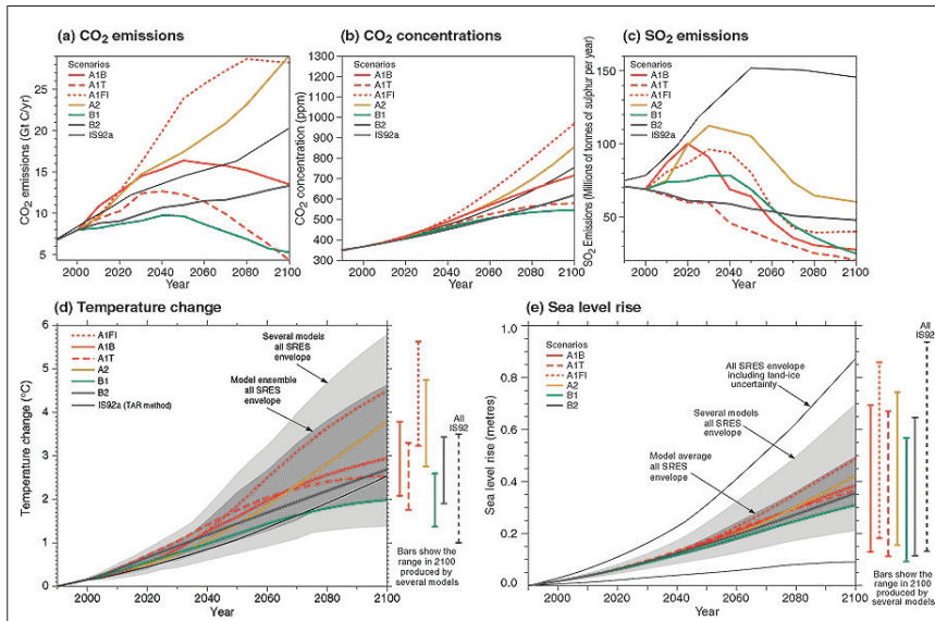
Figure 2.30 - The global climate of the 21 st century. The global climate will depend on natural changes and the response of the climate system to human activities. Climate models project the response of many climate variables – such as increases in global surface temperature and sea level – to various scenarios of greenhouse gas and other human-related emissions. (a) shows the CO 2 emissions of six illustrative scenarios. (b) shows projected CO 2 concentrations. (c) shows anthropogenic SO 2 emissions. Emissions of other gases and other aerosols were included in the model but are not shown in the figure. (d) and (e) show the projected temperature and sea level responses, respectively. Note that the warming and sea level rise from these emissions would continue well beyond 2100. (IPCC TAR - Climate Change 2001: The Scientific Basis).
