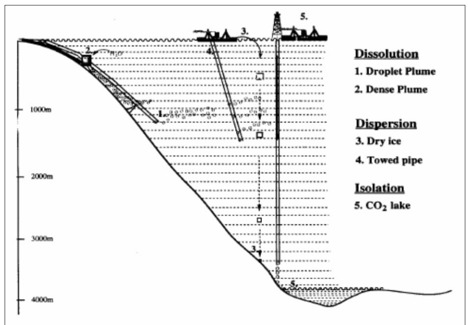
Figure 3.21 - Five suggested methods for injecting \text{CO}_2 into the deep ocean. (Herzog et al., 2001).
