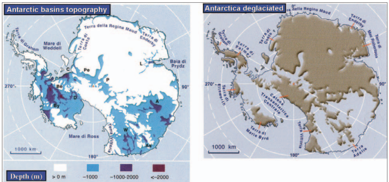
Figure 2.36 - Potential instability of the West Antarctic Ice Sheet (WAIS): The ice shelves fringing the coastal zones of Antarctica (not shown in the figure) are natural 'taps' of the Antarctic ice sheet system. They regulate the flow of continental ice towards the ocean and, correlatively, the amount of fresh water added to the ocean, eventually contributing to sea level rise. This in turn would result in reduced back stresses on the few 'pinning points' where the ice shelves are in contact with bedrock (see Figure 2.28), thus increasing continental ice flow rates and moving the grounding line further inland. The WAIS is mostly grounded below sea level. The figures (adapted from Manzani, 2001) show the depth of the ice-buried Antarctic basins (left) and what would result if all the area below present-day sea level was deglaciata (right). Although this is an oversimplified view that does not take into account the glacio-isostatic rebound (bedrock uplift as the ice burden disappears), it clearly illustrates how the processes described above could potentially destabilise the western part of the Antarctic ice sheet. (ULB-GLACIOL).
