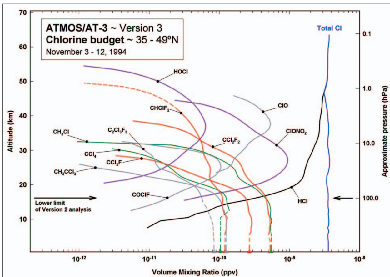
Figure 1.27 - The chlorine budget of the upper troposphere and stratosphere as derived for northern mid-latitudes. It includes all important chlorinated source, sink, and reservoir gases observed by ATMOS during NASA's shuttle mission ATLAS-3 (November 1994) and a few complementary constituents (grey traces) measured by other techniques. Notice the strong similarity (except for \text{CCl}_4 ) between the lowermost volume mixing ratios derived from ATMOS spectra and the corresponding in situ concentrations measured at ground level (triangle symbols) by the NOAA/CMDL network (National Oceanic and Atmospheric Administration / Climate Monitoring and Diagnostics Laboratory). (E. Mahieu, ULg-GIRPAS).
