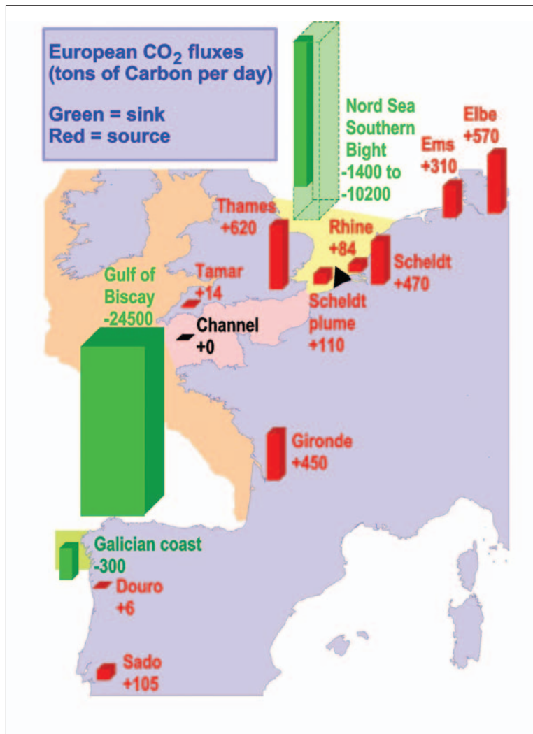
Figure 3.4 - CO 2 fluxes at the air-sea interface for various European estuaries and at the continental shelf. (ULg-OCEANCHEM).
