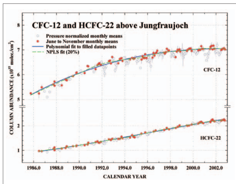
Figure 1.30 - Temporal evolutions of the total column abundances of CFC-12 (regulated) and HCFC-22 (unregulated), as observed above the Jungfraujoch (Switzerland) over the past 17 years. Note the discontinuity in the vertical scale. Continuous and dashed lines (distinguishable for CFC-12 only) represent least square fits to the June-to-November monthly mean columns (filled symbols) only, to avoid significant variability frequently caused by atmospheric transport during winter and spring. (R. Zander, ULg-GIRPAS).
