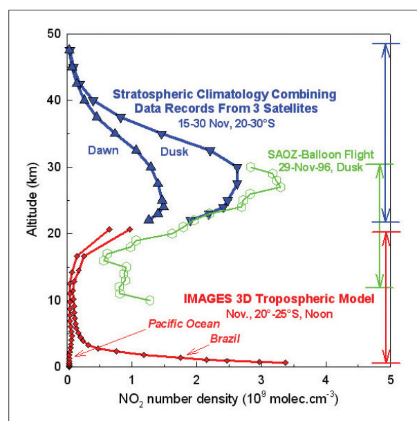
Figure 1.26 - Construction of a composite climatology of NO 2 profiles above Bauru (Brazil, 22°S) using complementary measurement records from satellites and balloons and from modelling results (dawn = sunrise; dusk = sunset). (J.-C. Lambert, BIRA / IASB).
