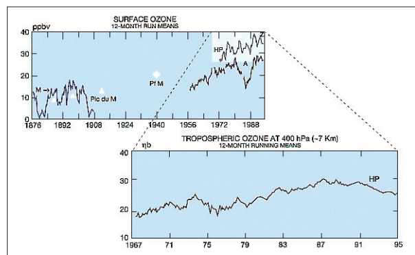
Figure 1.10 - Ozone concentrations in Western Europe since the 19 th century. As demonstrated by the measurements shown in the upper frame, surface ozone concentrations have more than doubled in Western Europe since the 19 th century. Century-old ozone observations in Montsouris (M), near Paris, and at Pic du Midi, in the French Pyrenees, are contrasted here with more recent measurements performed at several Western European sites (HP: Hohenpeissenberg; A: Arkona, both in Germany). Evidence of recent large ozone increases in the middle troposphere (at about 7 km altitude) is shown from ozone soundings at Hohenpeissenberg, in the lower panel of the figure. (WMO report nr. 44, 1999; C. Mensink, VITO-TAP).
