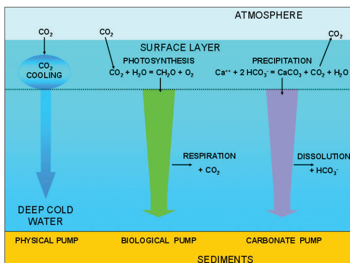
Figure 3.2 - Schematic representation of the major downward carbon fluxes within the ocean
