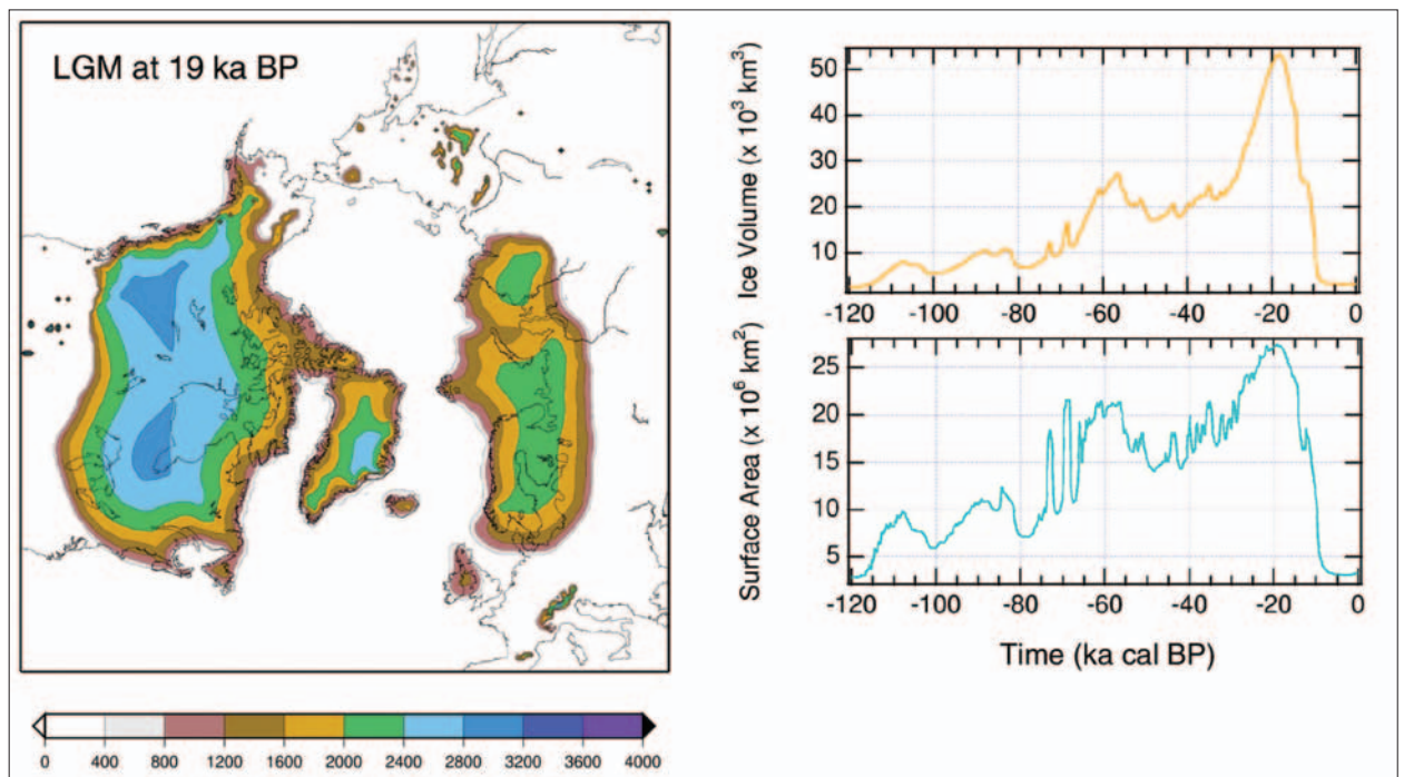
Figure 2.19 - Model simulation over the last glacial cycle showing the evolution of ice volume and surface area and the resulting ice sheet geometry at the Last Glacial Maximum 19 thousand years ago. The major characteristic of the Quaternary ice age was the growth and decay of large ice sheets on the continents of the northern hemisphere. The colour coding in the left panel refers to altitude above sea level. For comparison, an ice volume of 1 million km 3 corresponds to about 2.5 m of global sea level change. (VUB, 2003).
