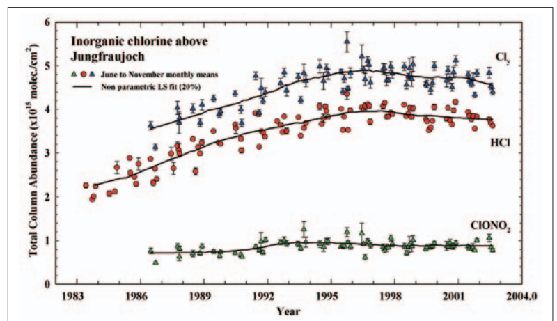
Figure 1.7 - Time series of monthly mean total vertical column abundances of HCl (hydrogen chloride) and \text{ClONO}_2 (chlorine nitrate) derived from infrared solar observations at the Jungfraujoch (Switzerland) from 1983 to 2002. Only June-to-November data have been used here, to avoid significant variability during the winter-spring period. Total inorganic chlorine ( \text{Cl}_y ), which is the sum of the HCl and \text{ClONO}_2 columns, is an excellent surrogate of the total inorganic chlorine loading in the stratosphere. The continuous lines represent the mean temporal trends of the various data sets. These evolutions provide robust evidence that total inorganic chlorine in the unperturbed stratosphere has stabilised recently, in response to the production regulations on chlorine-bearing substances with large ODPs (Ozone Depletion Potentials) outlined in the amended Montreal Protocol. (E. Mahieu, ULg-GIRPAS).
