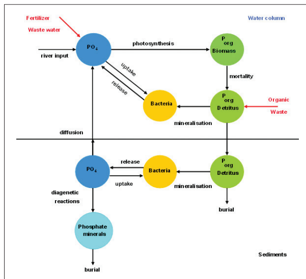
Figure 3.18 – Schematic representation of the phosphorus cycle in aquatic systems. The main anthropogenic perturbations are represented by red arrows.
