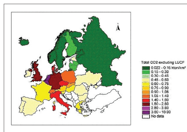
Figure 4.14 - UNFCC C emissions for Europe in 1997, excluding Land Use Cover Change (LUCF) effects. (F. Veroustraete, VITO-TAP).
