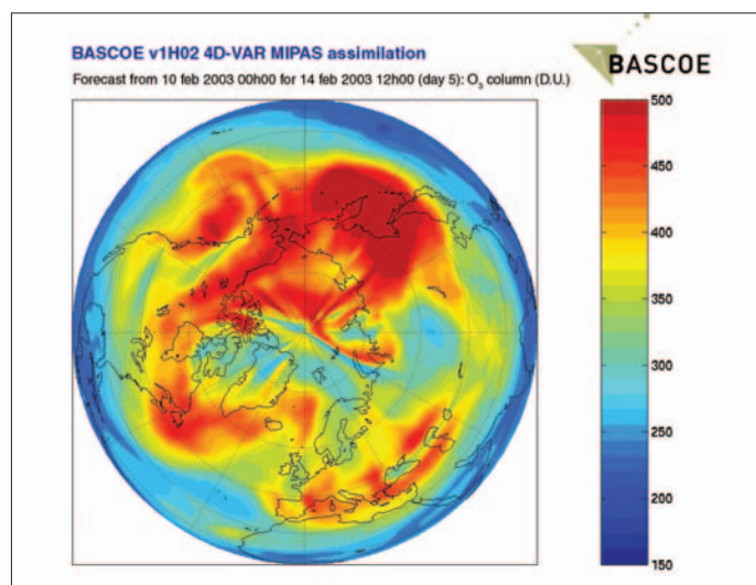
Figure 1.28 - Example of a model prediction of the northern hemisphere total ozone column (in Dobson units, DU) five days ahead, based on ENVISAT satellite observations using BASCOE (Belgian Assimilation System of Chemical Observations from ENVISAT). Subsequent observations have successfully confirmed the predictive approach. (D. Fonteyn, BIRA / IASB).
