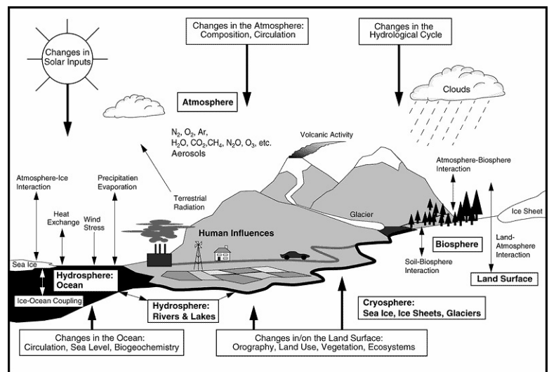
Figure 2.1 - Schematic view of the components of the global climate system (bold text in boxes), their processes and interactions (thin arrows), and some aspects that may change (bold arrows). (IPCC TAR - Climate Change 2001: The Scientific Basis).
