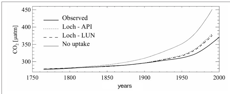
Figure 3.11 - Evolution of the observed atmospheric CO 2 between 1765 and 2000 as compared with (1) the evolution that would have resulted in the absence of uptake by the ocean and (2) computed changes in atmospheric CO 2 due to anthropogenic fluxes, using the ocean carbon cycle model LOCH coupled with the API or LUN ocean circulation model. (ULg-LPAP).
