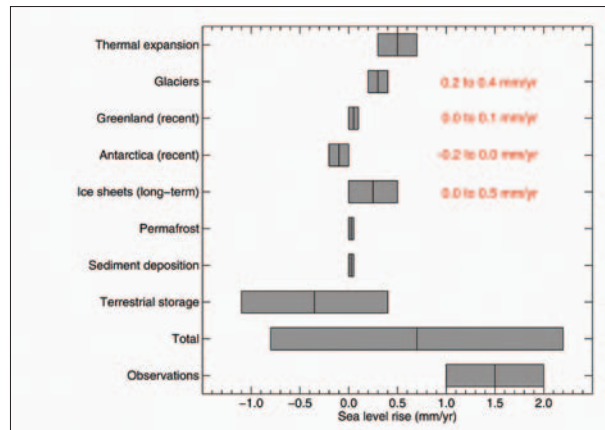
Figure 2.27 - Ranges of uncertainty for the average rate of sea level rise in the 20 th century, and estimated contributions of different processes. (IPCC TAR - Climate Change 2001: The Scientific Basis).
