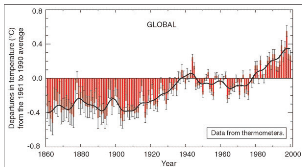
Figure 2.3 - Combined annual land-surface, air, and sea-surface temperature anomalies (°C) from 1861 to 2000, relative to 1961 to 1990. Two standard error uncertainties are shown as bars on the annual number. (IPCC TAR - Climate Change 2001: The Scientific Basis).
