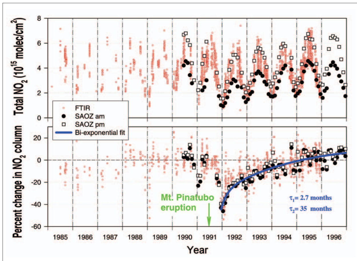
Figure 1.5 - Total \text{NO}_2 reduction at the Jungfraujoch (Switzerland) after the Mt. Pinatubo (Philippines) eruption of June 1991. The top frame shows a superposition of infrared (FTIR, Fourier Transform Infrared; small red circles) and UV-Visible (filled circles and open squares) time series of \text{NO}_2 columns above the Jungfraujoch. The bottom frame shows the percentage monthly mean vertical \text{NO}_2 column reductions observed at the Jungfraujoch by both instruments. The UV-Visible data are monthly means for morning (am) and evening (pm) vertical column amounts; the infrared data are daily mean values. (M. De Mazière, BIRA / IASB).
