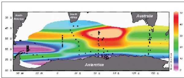
Figure 3.7 - Synoptic view of the mineralisation of organic carbon exported to the deep sea via the biological pump in the Southern Ocean. The data were calculated using the barite proxy of organic carbon mineralisation along vertical profiles at the stations indicated on the map. This flux reflects the importance of the biological pump in the area. The \text{CO}_2 released by bacterial activity in the deep sea remains sequestered on a time scale ranging from decades to a few centuries. (KMMA / MRAC, VUB-ECOL).
