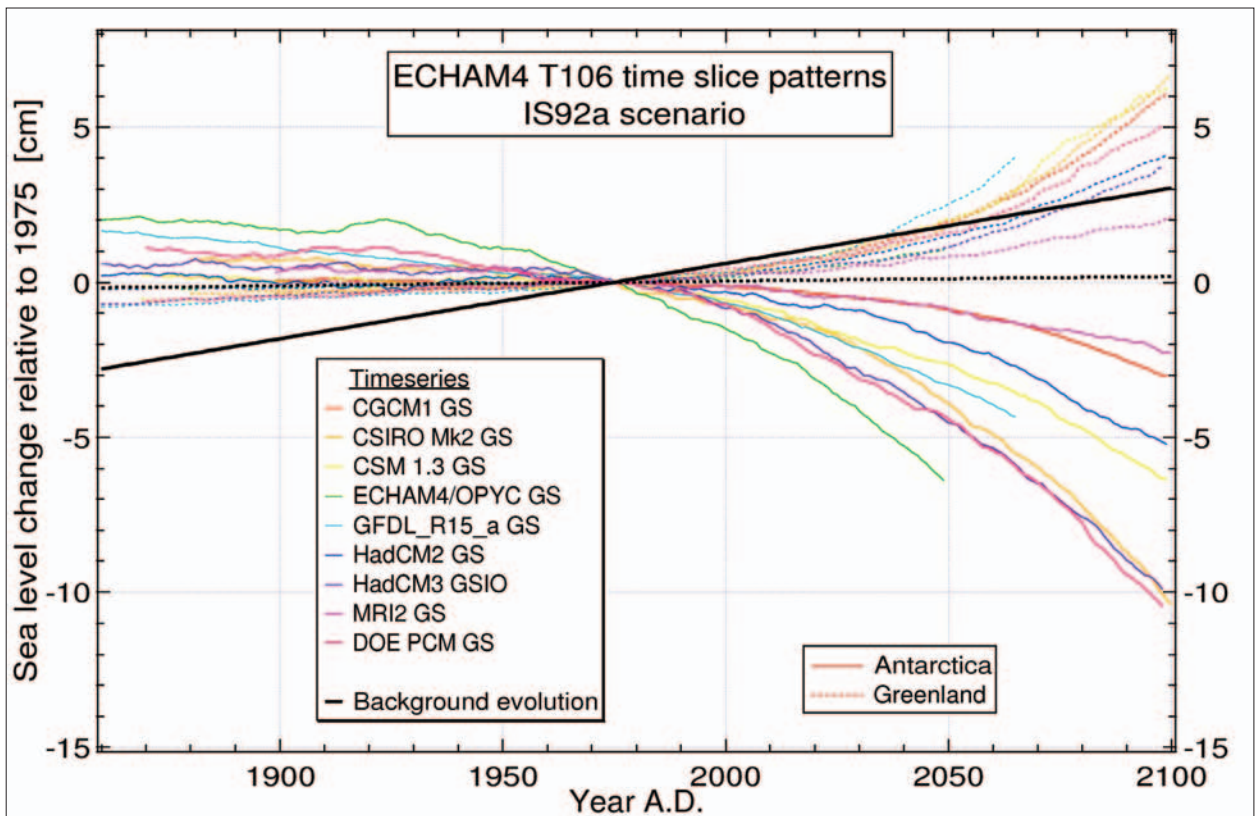
Figure 2.32 - Projected mass changes over the Antarctic and Greenland ice sheets obtained from 3-D ice sheet models. The background evolution resulting from the ongoing response to past climate changes is shown by the thick black lines. These simulations formed the basis of the sea level projections of the IPCC TAR - Climate Change 2001: The Scientific Basis. (VUB-DG).
