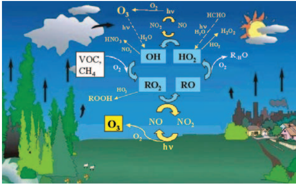
Figure 1.9 - General scheme of ozone formation and oxidation of volatile organic compounds (VOCs) in the troposphere. (J.-F. Muller, BIRA / IASB and J. Peeters, KULeuven-PAC).
