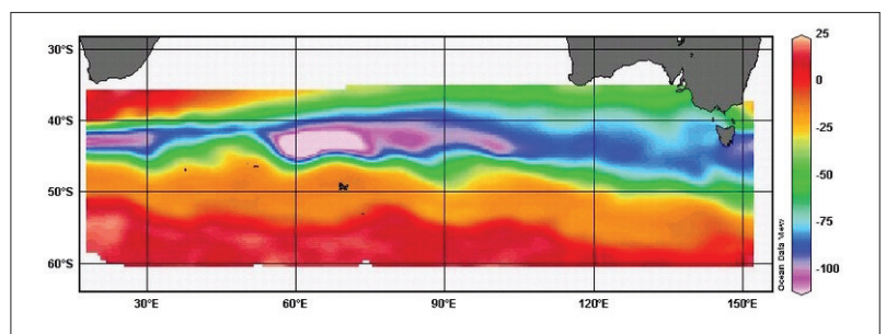
Figure 3.8 - Spring and summer mean air-sea fluxes of \text{CO}_2 for the Indian sector of the Southern Ocean (between 35 and 60^\circ\text{S} ). The fluxes are in \text{mg carbon/m}^2/\text{day} . The map has been reconstructed from the results of five campaigns of \text{CO}_2 measurement and extrapolated using remote sensing of sea surface temperature and wind speed. (ULg-OCEANCHEM).
