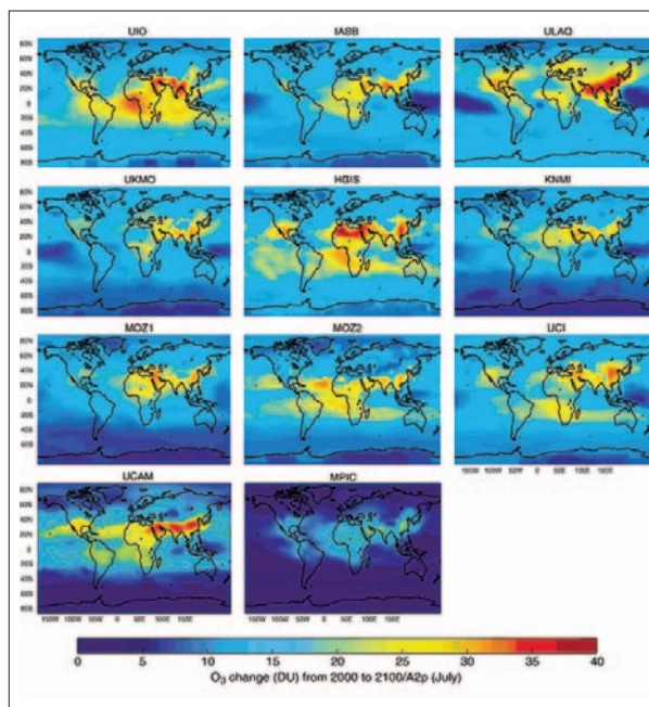
Figure 1.13 - Predicted change in the tropospheric ozone total column amount (in Dobson units) in July due to man-made emissions in 2100 relative to year 2000, according to 11 models of the global tropospheric composition, including IMAGES (Intermediate Model for the Annual and Global Evolution of Species) from BIRA / IASB. The IPCC projections for CH 4 , CO, VOCs, and NO x were used in these simulations (see IPCC Special Report on Emission Scenarios, IPCC SRES). The emission scenario accounts for the projected evolution in population number, GNP (Gross National Product) per capita, technology and pollution control measures in different parts of the world. The global tropospheric ozone is predicted to increase by up to 60% according to the different IPCC scenarios, but with a considerable uncertainty. Note that the possible impacts of climate change on the composition are not taken into account in these simulations, although they were shown to be potentially significant. (J.-F. Muller, BIRA / IASB).
