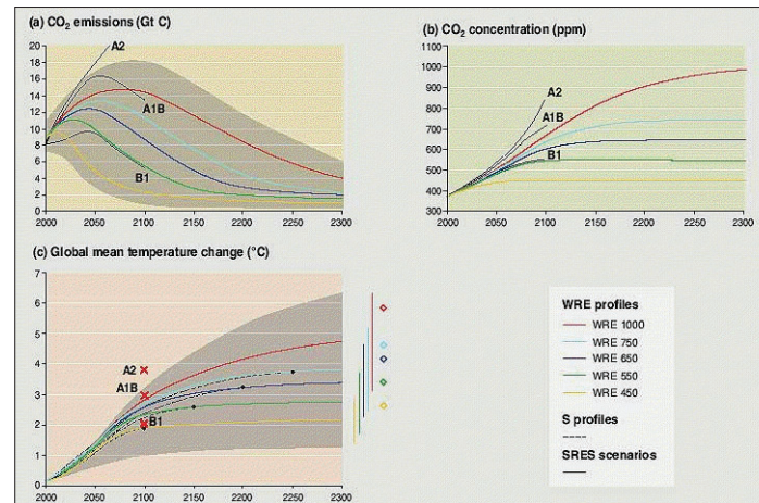
Figure 2.44 – Emissions, concentrations and temperature changes corresponding to different stabilisation levels for \text{CO}_2 concentrations. Stabilising \text{CO}_2 concentrations would require substantial reduction of emissions below current levels and would slow the rate of warming.
