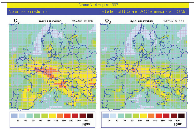
Figure 1.16 - Visualisation of episodic peak ozone concentrations over Europe on August 6, 1997 at 12.00h, as computed by the EUROS model, using emissions of 1997 without emission reductions (left) and with 50% reduction of NO_x and VOC emissions in Europe compared to 1997 (right). The O_3 peak concentration is indicated according to the bottom colour scale ( 1 \mu g/m^3 O_3 = 0.70 \text{ ppbv } O_3 ). According to these model simulations, reductions of NO_x and VOCs clearly have a positive impact on the tropospheric O_3 peak concentrations. The effect is confirmed by present observations. (C. Mensink, VITO-TAP and CELINE / IRCEL).
