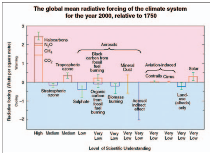
Figure 1.20 - Current estimates of the radiative forcing due to increased concentrations of atmospheric constituents and other mechanisms. Note that certain aerosol types (sulphate, biomass-burning aerosols) lead to cooling, whereas others (black carbon) lead to warming. Also, note the very large uncertainty as to the indirect aerosol forcing. (IPCC TAR, 2001).
