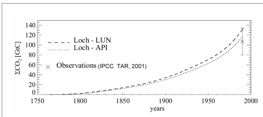
Figure 3.12 - Amount of carbon stored in the ocean since 1765. The ocean inventories correspond to the model results when the observed atmospheric CO 2 concentrations are imposed. (ULg-LPAP).
