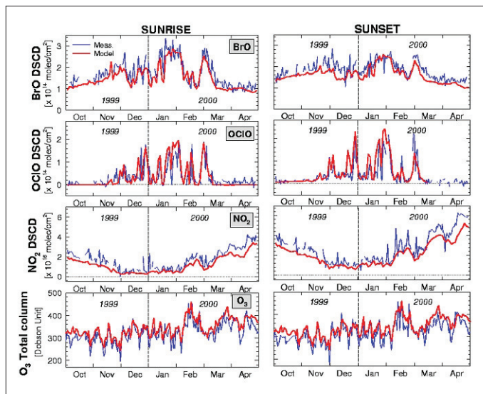
Figure 1.2 - Observed and calculated BrO ( 80-90^\circ solar zenith angle, sza ), OCIO ( 80-92^\circ sza ), and NO_2 ( 80-90^\circ sza ) differential slant column densities (DSCD), and O_3 total columns in Dobson units, for sunrise (left) and sunset (right) at Harestua (Norway, 60^\circ N ) for the winter 1999/2000. These comparisons show that model calculations reproduce quite well most observed features, thus indicating that the important activation processes involved in ozone depletion at northern latitudes (both inside and outside the vortex) are well implemented in the model algorithms used here. The Dobson unit, DU, is defined in Annex 9. (F. Hendrick, BIRA / IASB).
