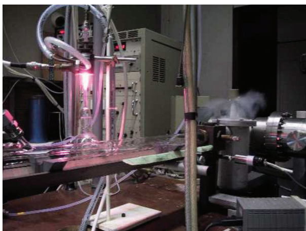
Figure 1.17 - Fast-flow reactor in operation at KULeuven-PAC. This instrument, in combination with on-line mass spectrometric detection, has been built for determining the products of monoterpene reactions. This approach represents a smaller-scale alternative to the more expensive and less accessible research facilities in Europe. Hydroxyl radicals (OH) are produced in the afterglow of microwave-induced plasma. A methodology has been developed for the analysis of degradation products. (C. Vinckier, KULeuven-PAC).
