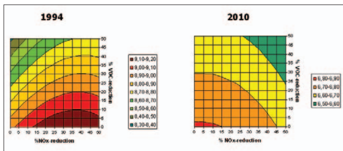
Figure 1.15 - Accumulated ozone concentrations in excess of 40 ppbv ( AOT_{40} ), as a function of NO_x and VOC reductions in 1994 (left) and 2010 (right). The diagrams show that in 1994 a moderate reduction of NO_x emissions in Belgium would have resulted in an increase in AOT_{40} , whereas any reduction in VOC emissions would have resulted in a decrease in AOT_{40} . In 2010, both NO_x and VOC reductions would result in a decrease in the AOT_{40} . (C. Mensink, VITO-TAP).
