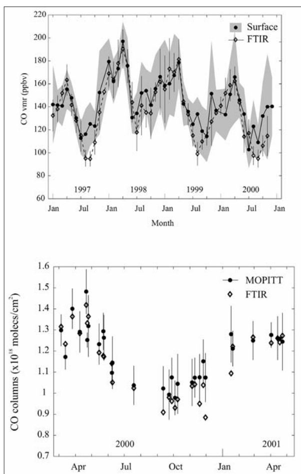
Figure 1.25 - Example of the synergistic use of multiplatform measurements of carbon monoxide (CO) abundances at the Jungfraujoch (Switzerland), for the assessment of their respective qualities. Top panel: comparison between monthly means of CO surface volume mixing ratios as measured in situ by the Swiss Federal Laboratories for Materials Testing and Research (EMPA) and remotely by Fourier Transform Infrared (FTIR) spectrometers operated by ULg-GIRPAS. Bottom panel: comparison between daily means of CO column amounts above the station's altitude measured by FTIR and by Monitoring of Pollution In The Troposphere (MOPITT). The very strong similarity between the ground-based remote sensing FTIR measurements and the in situ and space-borne infrared measurements helps scientists to gain confidence in the ability of a ground-based FTIR to monitor the vertical distribution of CO in the lower atmosphere. (B. Barret, BIRA / IASB and E. Mahieu, ULg-GIRPAS).
