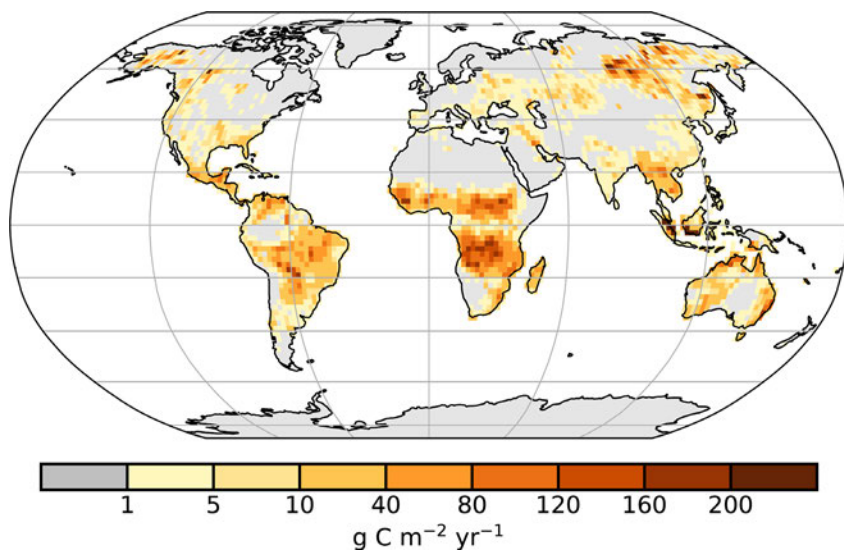
Fig. 2.67. Global map of fire activity ( \text{g C m}^{-2} \text{ yr}^{-1} ) in 2019 in terms of carbon consumption. (Source: GFASv1.4.)
