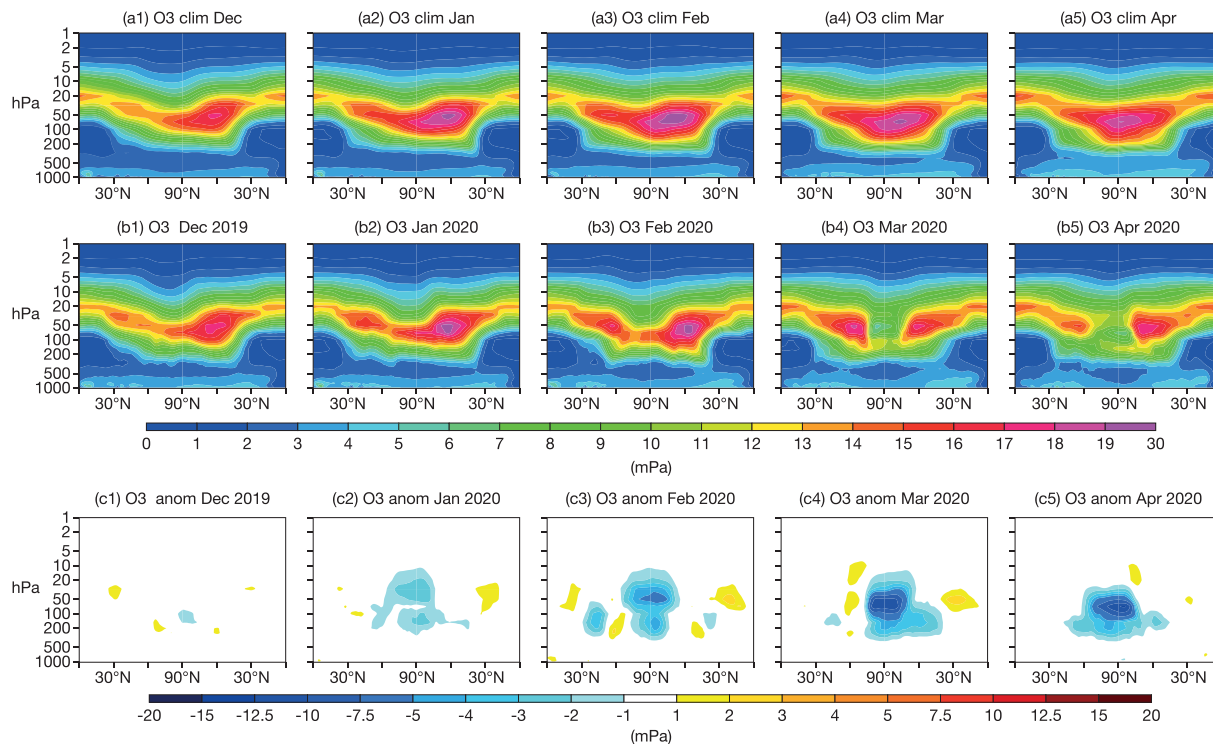
Figure 6. (a) Cross sections of monthly mean climatologically averaged ozone partial pressure (in mPa) from the CAMS reanalysis (2003–2019) along one meridian ( 0^\circ\text{E}/180^\circ\text{E} ) from the equator north via the North Pole and back to the equator, (b) corresponding cross sections for 2019/2020, and (c) cross sections of anomalies for 2019/2020 for December (Column 1), January (Column 2), February (Column 3), March (Column 4), and April (Column 5).
