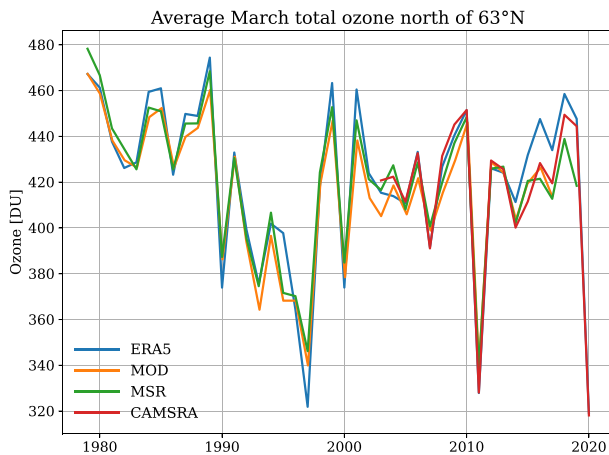
Figure 1. Time series of monthly mean March TCO 3 in Dobson units (DU) averaged over the area north of 63°N from NASA's merged ozone data set (MOD, orange), ERA5 (blue), Multi Sensor Reanalysis (MSR, green), and CAMS reanalysis (CAMSRA, red).
