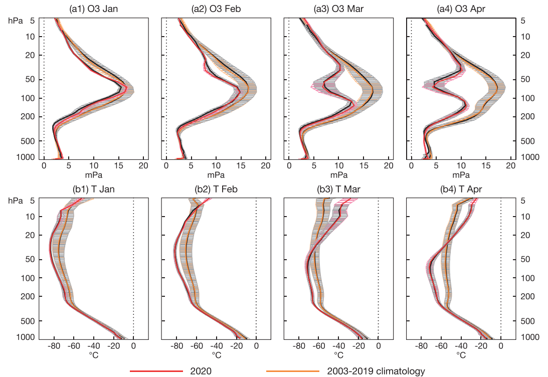
Figure 7. Comparisons of (a) ozone (in mPa) and (b) temperature (in °C) profiles from the CAMS reanalysis and ozonesondes at Ny-Ålesund for January (Column 1), February (Column 2), March (Column 3), and April (Column 4). The red profiles show monthly mean CAMS reanalysis values for 2020, and the orange profiles the climatological mean from the CAMS reanalysis (2003–2019). Black lines show the corresponding means from the ozonesondes. The hatched area depicts \pm one standard deviation. The number of ozone profiles that went into the averages were January 2020: 6; February 2020: 8; March 2020: 16; April 2020: 13; January climatology: 187; February climatology: 178; March climatology: 177; and April climatology: 98.
