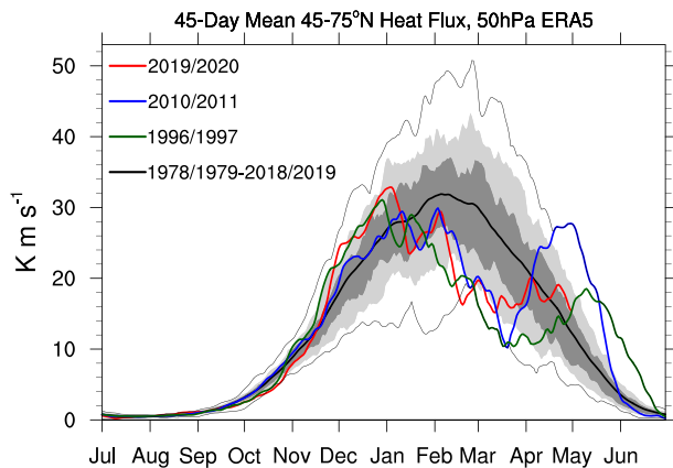
Figure 5. Eddy heat flux in \text{km s}^{-1} at 50 hPa averaged between 45^\circ\text{N} and 75^\circ\text{N} for the 45-day period prior to the date indicated, calculated from ERA5 data. The light shading is the 10th to 90th percentile and the darker shading the 75th–25th percentile. The thin black lines are maximum and minimum values, the thick black line the mean, the red line the values for winter/spring 2019/2020, the blue line for 2010/2011, and the green one for 1996/1997.
