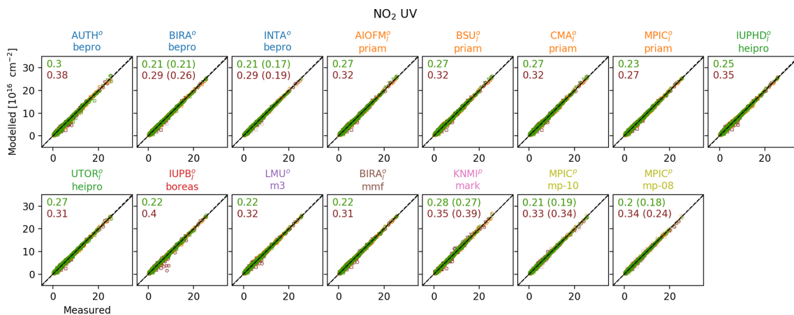
Figure 11. \text{NO}_2 UV dSCD correlation. RMSD between measured and modelled dSCDs is in units of 10^{16} molec. \text{cm}^{-2} . Legends and description of Fig. 8 apply.
