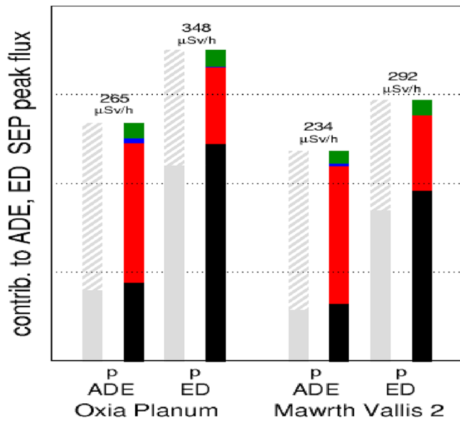
Figure 7. Contributions of the ADE and ED hourly rates for the peak flux of the October 28, 2003 SEP event. ADE, Ambient Dose Equivalent.
