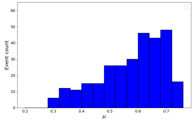
Fig. 7. Distribution of the shape change coefficient \mu derived in this work.
