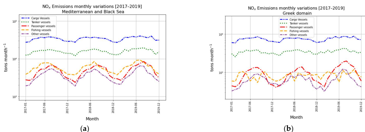
Figure 7. CAMS-GLOB-SHIP \text{NO}_x emissions time series from 2017 to 2019 (in tons per month) classified according to the EMODnet vessel density data of all the available years: Cargo vessels in blue, tanker vessels in green, fishing vessels in orange, passenger vessels in red and other vessels in purple; (a) Mediterranean and Black Sea; (b) Greek domain.
