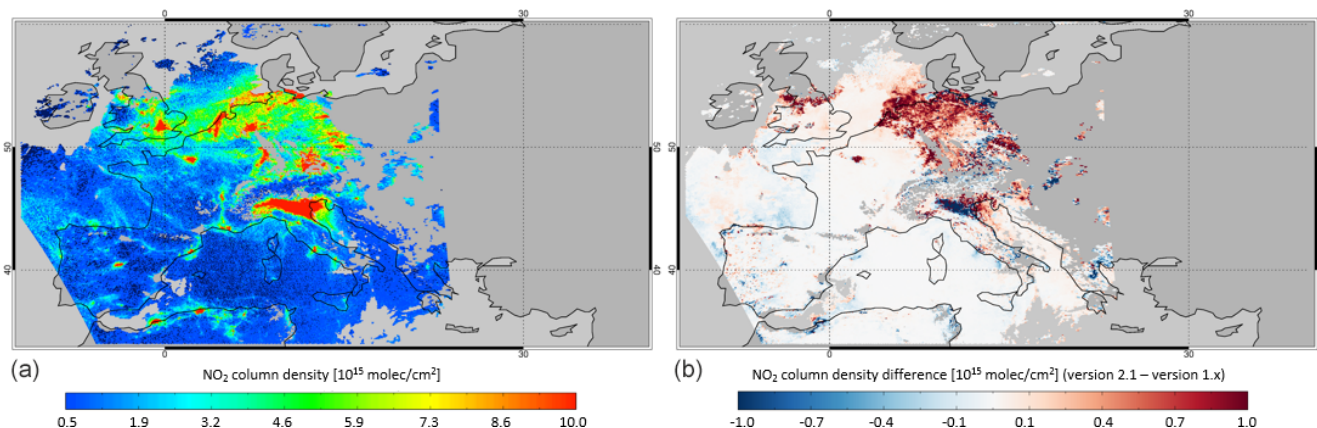
Figure 15. Tropospheric NO 2 columns retrieved using the OCRA/ROCINN cloud parameters from the version 2.1 processor (a) and differences with version 1.x (b) over Europe for orbit 6939 on 14 February 2019. Only measurements with a cloud radiance fraction less than 0.5 are included.
