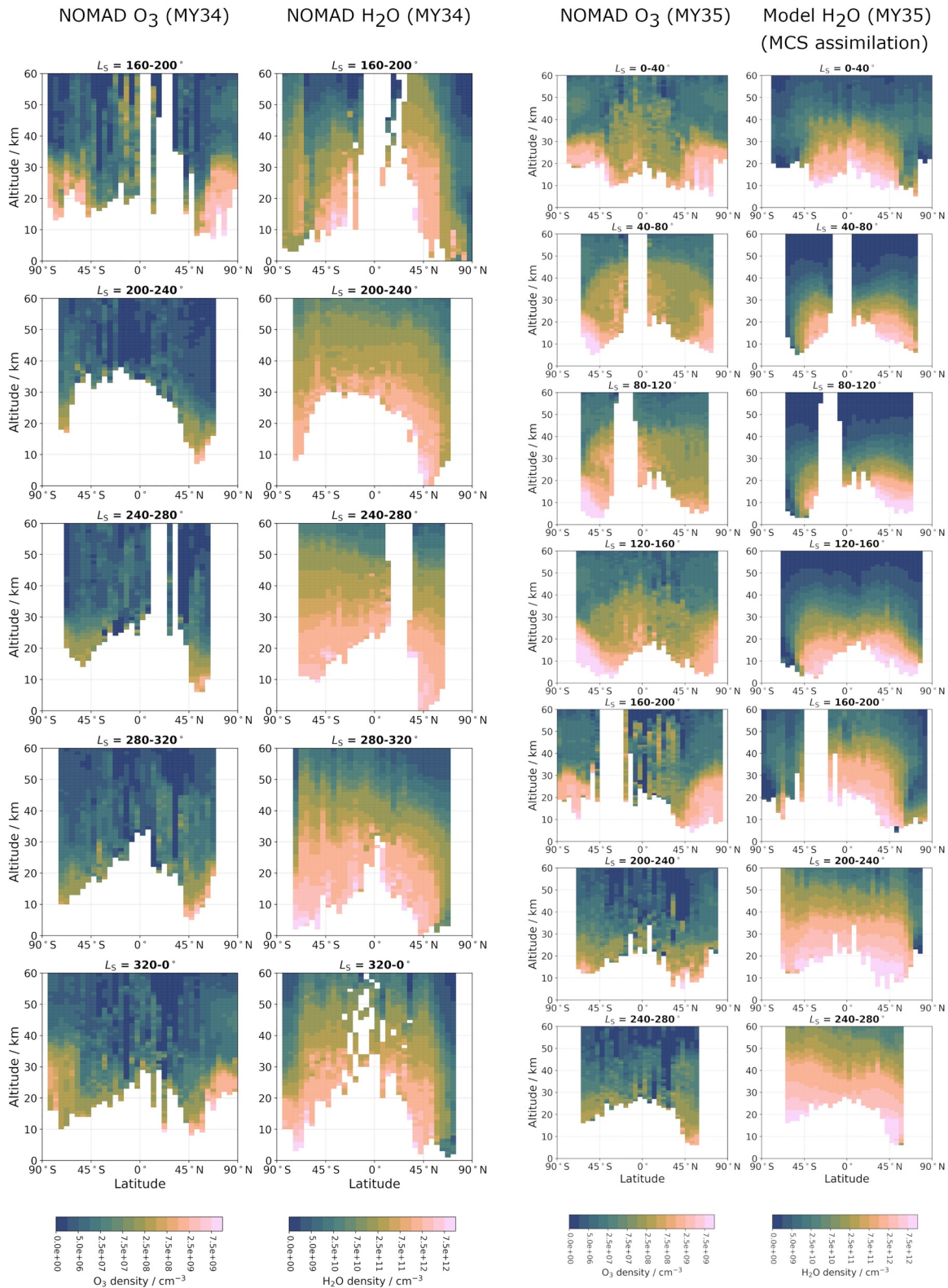
Figure 10. Latitudinal distribution comparison of (left column pair) NOMAD O_3 retrievals and (right column) NOMAD H_2O retrievals (Aoki et al., 2019), in L_S intervals of 40^\circ during MY34, and (right column pair) as left pair but for MY35, and with assimilated model output for H_2O . Retrievals are binned every 5^\circ latitude and 1 km altitude for clarity. The same color scale is used for both species, with different absolute scales.
