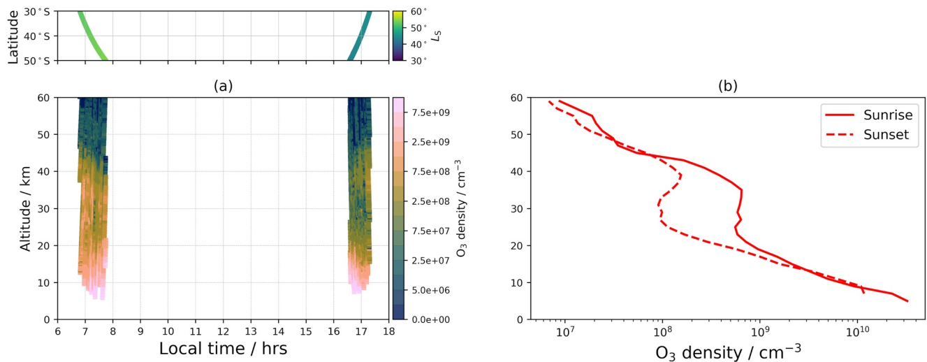
Figure 12. Sunrise and sunset occultations showing the O_3 vertical profile number density for (a) individual profiles over the period L_s = 42^\circ – 54^\circ and the latitude range 30^\circ – 50^\circ S, and (b) the average of these profiles split by sunrise and sunset observation geometry. The exact latitude and L_s for each profile is shown above the plot.
