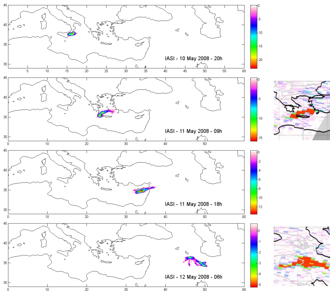
Figure 5: Maps of an SO 2 concentration index from IASI data, in terms of a temperature-brightness difference, after an eruption of Etna (Sicily) in the afternoon of 10 May 2008, showing the motion of the SO 2 cloud to the east. The times given are the times in UTC of the measurement of the SO 2 patch. Note that the colour scale changes between the successive maps. The small pictures on the right are cuts from GOME-2 SO 2 maps at the times corresponding to the IASI maps on the left; the colour bar of these maps is that of Figure 3.
