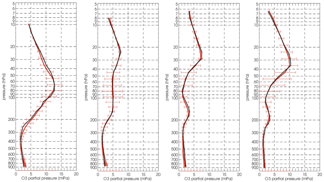
Fig. 8.1.8: Ozone in August, September, October and November 2015 over the Antarctic.
