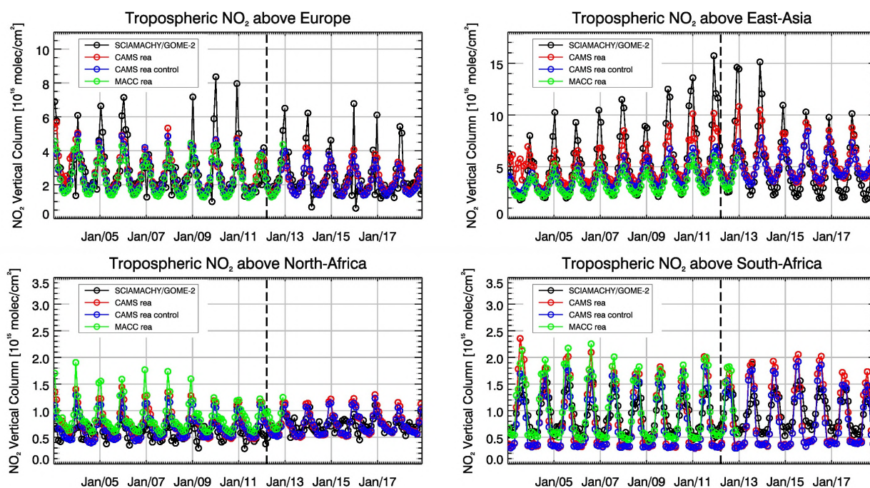
Figure S.9. Comparison of time series of tropospheric NO 2 columns from SCIAMACHY (up to April 2012) and GOME-2 (from April 2012 onwards) to model results over selected regions. The switch from SCIAMACHY to GOME-2 is indicated by the vertical black dashed lines. Upper panels represent regions dominated by anthropogenic emissions; lower panels represent those dominated by biomass burning.
