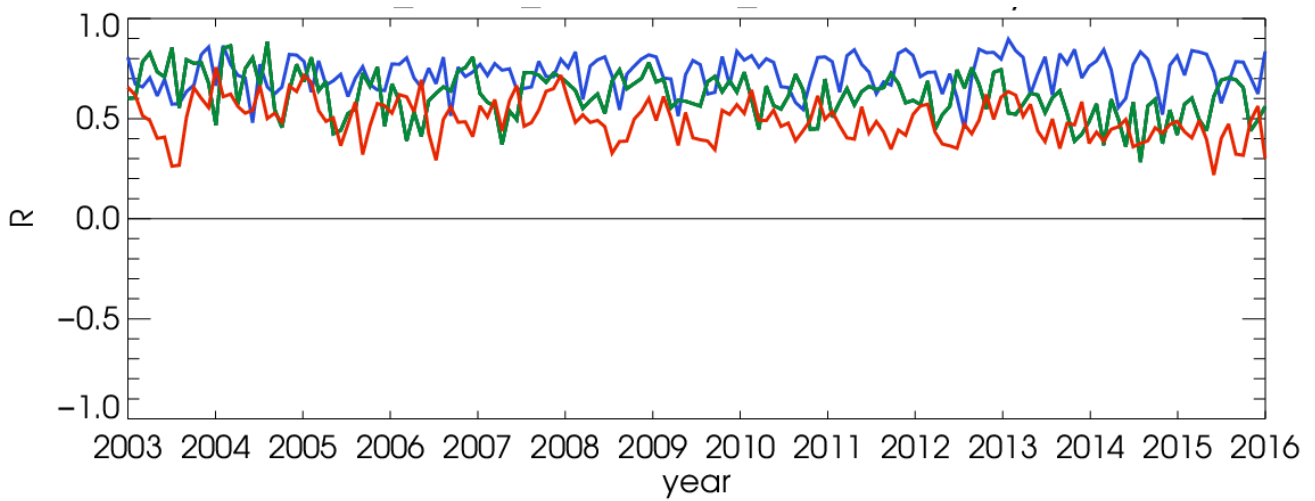
Figure 5.1.2a: Monthly correlation coefficients (R) for GAW stations calculated for the years 2003-2015 for the CAMS reanalysis, averaged over different regions (North America: green, Northern midlatitudes: red, Asia/Japan: blue). After 2015, there are not enough observations for reliable the calculation of average Rs.
