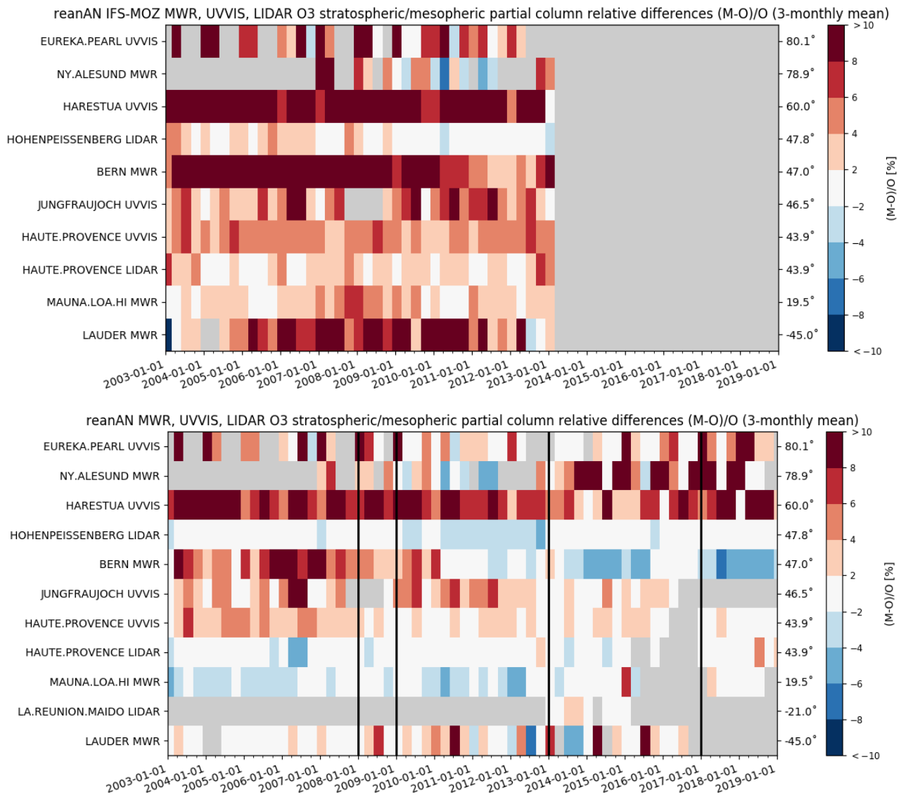
Figure 8.2.2: Time series of seasonal-mean relative partial column differences for stratospheric (LIDAR, UUVIS) and mesospheric (MWR) data products from the NDACC MWR, UUVIS, LIDAR instruments. At some sites a trend can be observed in the seasonal biases for the both models. The MACC reanalysis is shown at the top, the CAMS reanalysis at the bottom.
