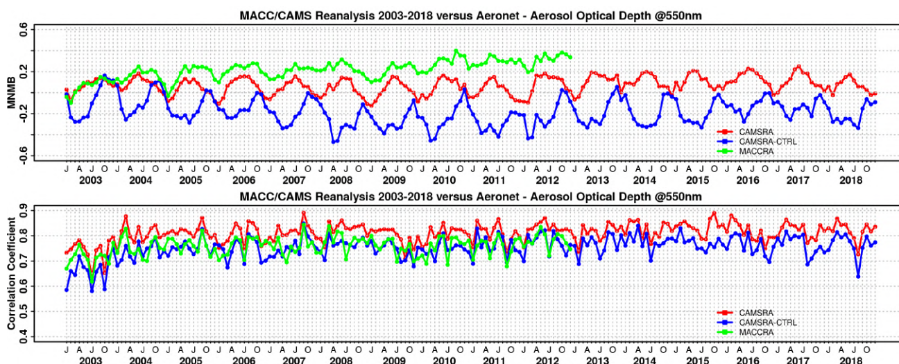
Figure S.1: Aerosol optical depth at 550nm in IFS 00Z model simulations for 2003 – 2018 against daily matching Aeronet Version3 level 1.5; (top) Modified normalized mean bias (MNMB); CAMS reanalysis (red) and control run (blue); MACC reanalysis (green); (bottom) Corresponding correlation coefficient.
