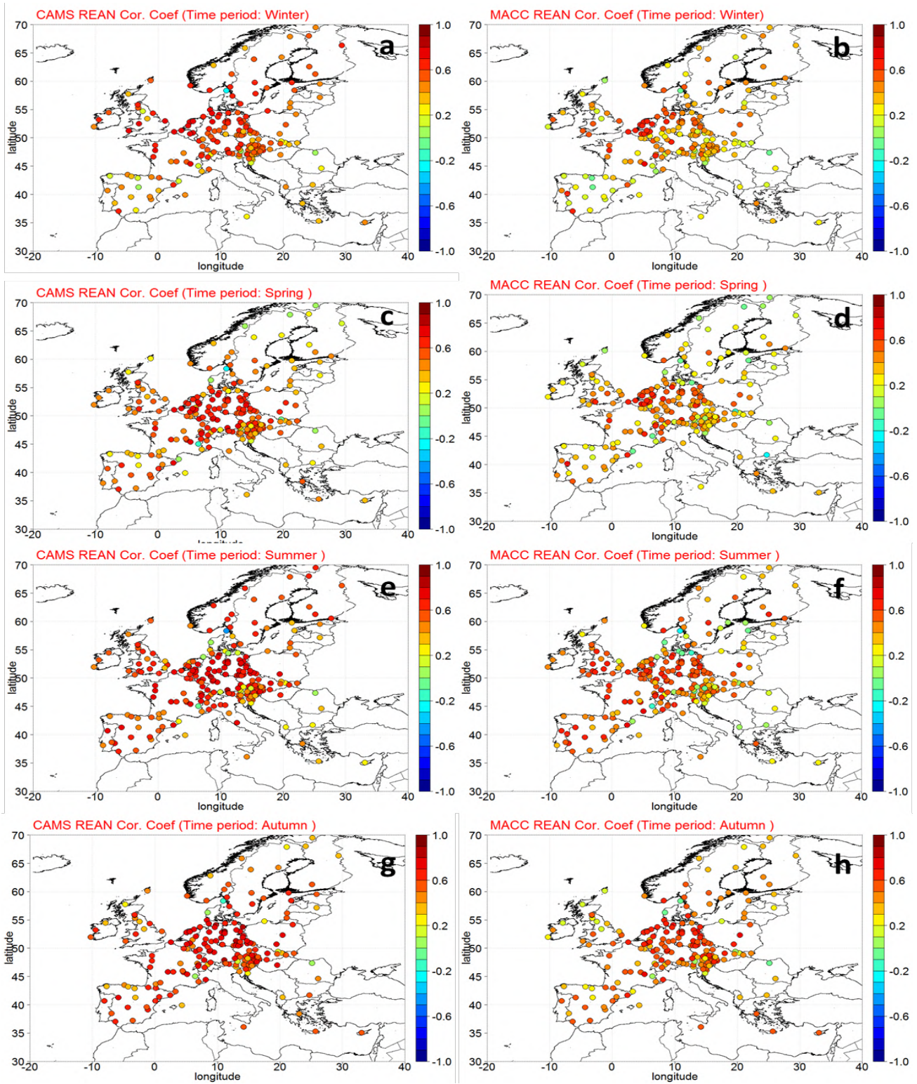
Figure 4.3.6. Correlation Coefficients ( r ) for EMEP data during Winter 1st row, a and b), Spring (2nd row, c and d), Summer (3rd row, e and f) and Autumn (4rd row, g and h) for the CAMS reanalysis (left) and the MACC reanalysis (right).
