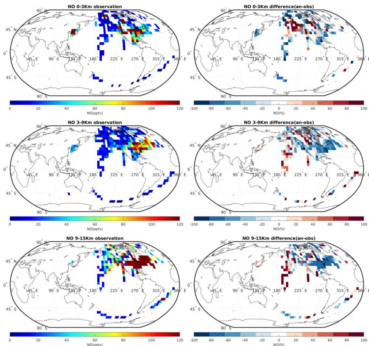
Figure 7.2.6: The campaign observation of NO in pptv (left, see table 7.1.1 and 7.1.2), the difference between the reanalysis and the observation (difference = reanalysis – observation; right). The data are averaged to 5x5 (latitude x longitude) and to three altitude bins: 0-3 Km (top), 3-9 Km (middle), and 9-15Km (bottom).
