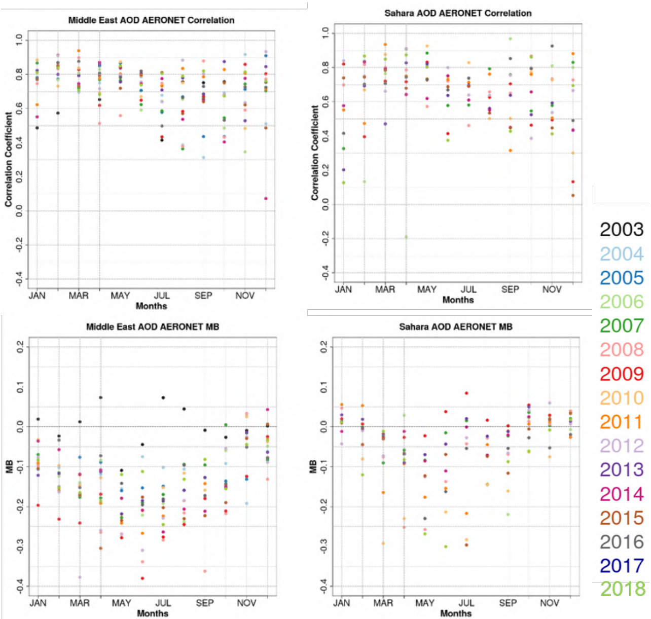
Figure 3.2.3a: Monthly correlation coefficient ( r , upper panels) and Mean Bias (MB, bottom panels) of CAMS reanalysis (on 3-hourly basis) for the years 2003-2018 in the Middle East and Sahara regions. Dust-filtered DOD from AERONET Version 3 cloud-screened is the reference.
