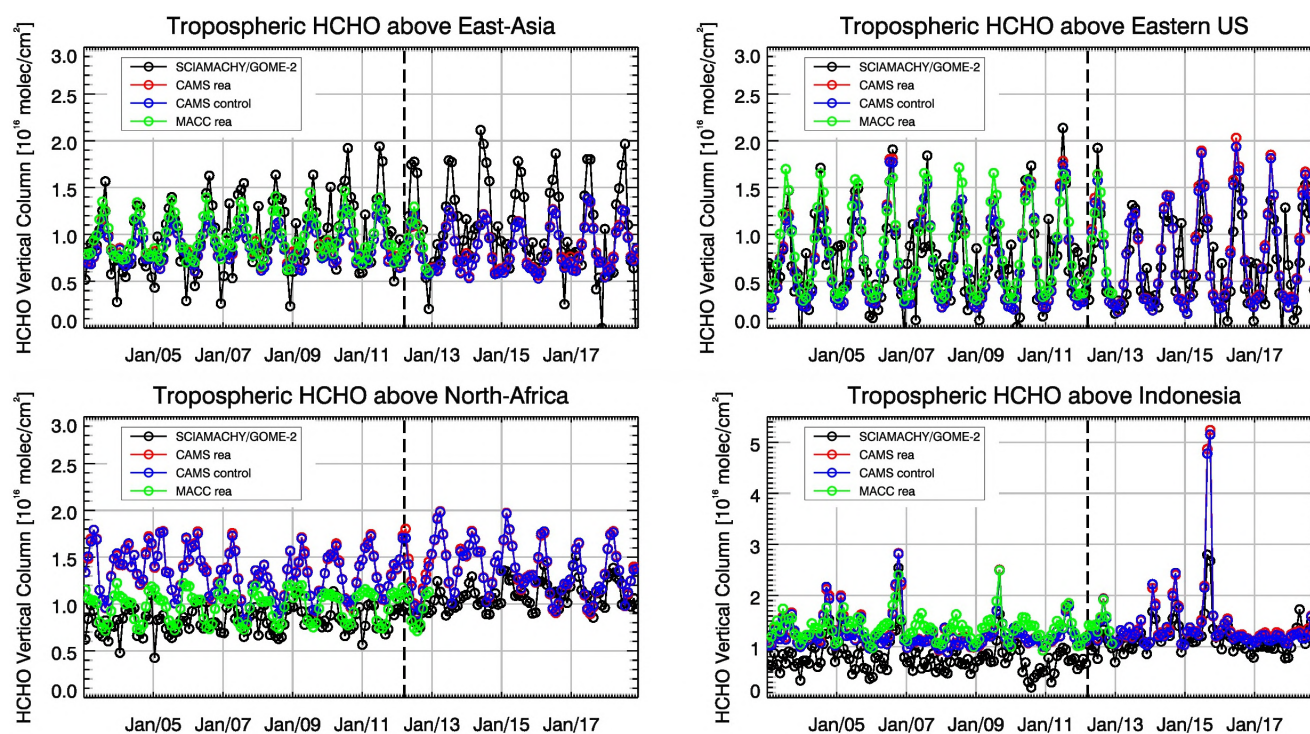
Figure 6.2.1: Comparison of time series of tropospheric HCHO columns from SCIAMACHY (up to April 2012) and GOME-2 (from April 2012 onwards) to model results over selected regions. The switch from SCIAMACHY to GOME-2 is indicated by the vertical black dashed lines. The regions differ from those used for NO 2 to better focus on HCHO hotspots: East Asia (25–40°N, 110–125°E), Eastern US (30–40°N, 75–90°W), Northern Africa (0–15°N, 15°W–25°E) and Indonesia (5°S–5°N, 100–120°E). Negative satellite retrieved values over Eastern US and East-Asia are due to the limited amount of data during Northern Hemisphere winter months for these regions.
