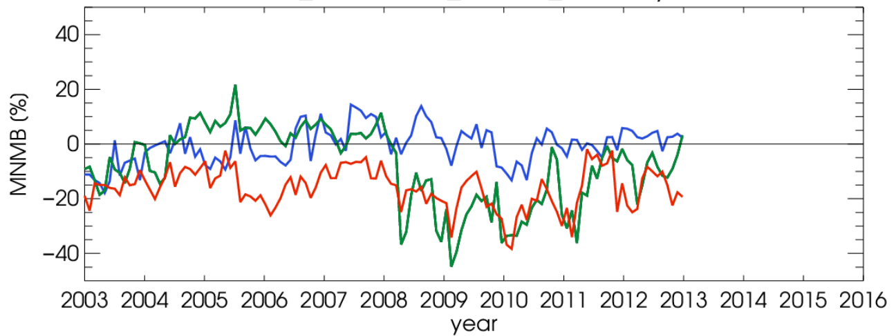
Figure 5.1.1b: Same as Fig. 5.1.4a, but for the MACC reanalysis.
