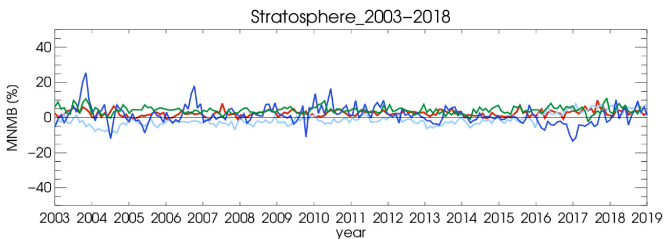
Fig. 8.1.1: Normalised bias of the reanalysis versus ozone sondes, for 4 regions in the stratosphere (dark blue: Antarctic, light blue: Arctic, red: Northern midlatitudes, green: Tropics). The biases are averaged between 90 and 10hPa in the extra-tropics and between 60 and 10hPa in the Tropics.
