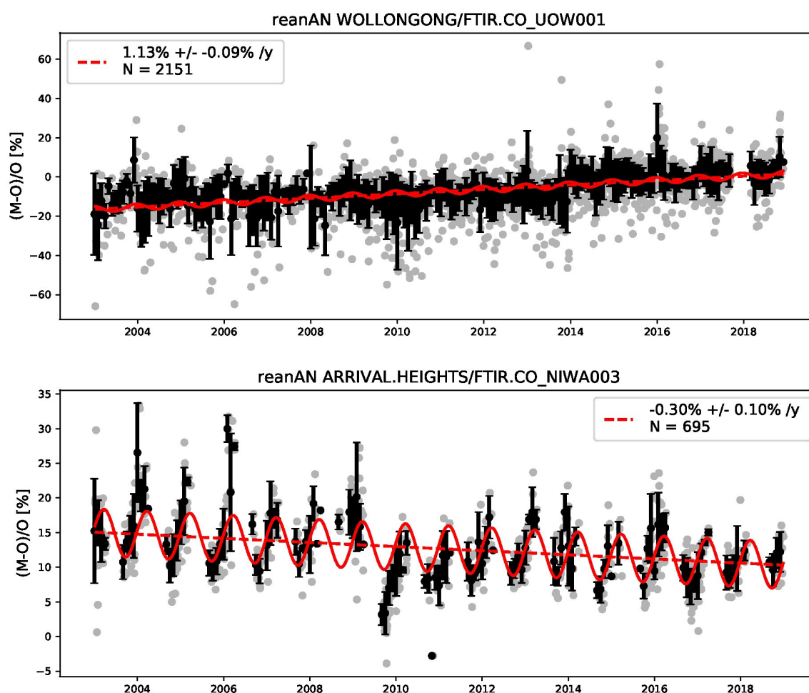
Figure 5.3.5: Trend estimates for the relative bias of the CAMS reanalysis for southern hemispheric NDACC-FTIR stations. At Maitopo, Lauder and Wollongong a positive trend is observed, while at the Antarctic site Arrival Heights a negative trend is seen with a significant seasonal change in the relative differences.
