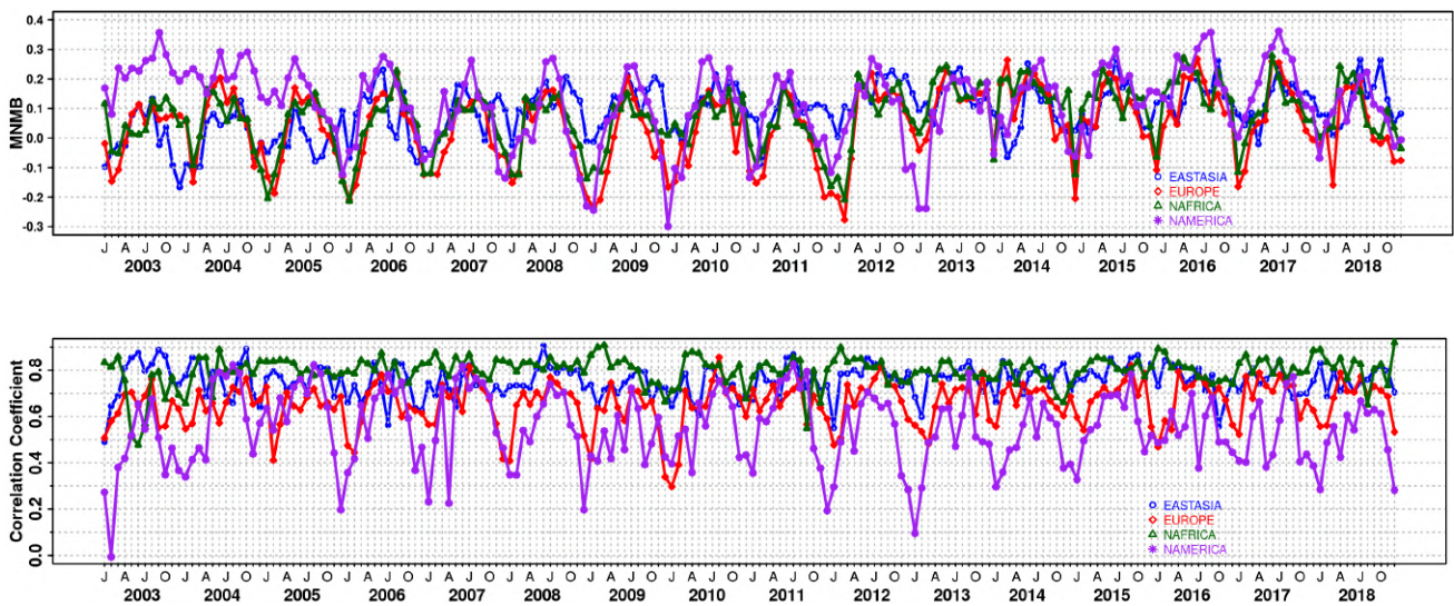
Figure 3.1.7: a) Modified normalized mean bias (MNMB) and b) correlation coefficient in AOD for 2003-2018 based on daily AOD comparison (Aeronet V3 level 1.5) in four world regions [East Asia (blue); Europe (red); North Africa (green); North America (purple)] for the CAMS reanalysis.
