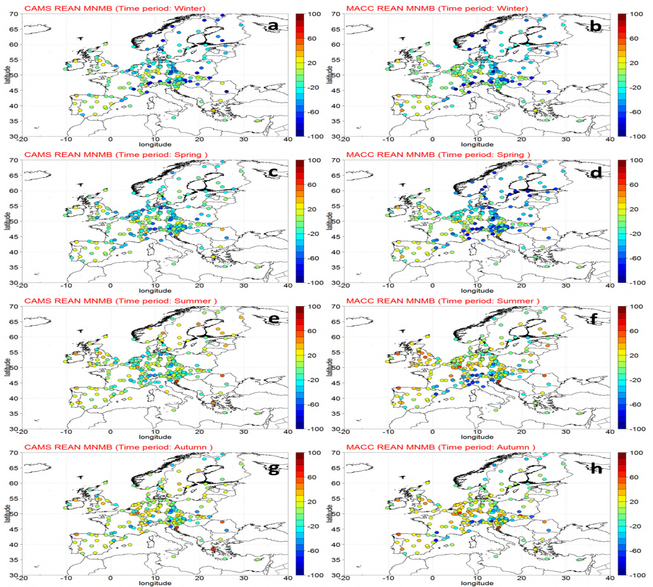
Figure 4.3.5. Modified Normalized Mean Biases (MNMBs) for EMEP data during Winter (1st row, a and b), Spring (2nd row, c and d), Summer (3rd row, e and f) and Autumn (4rd row, g and h) for the CAMS reanalysis (left) and the MACC reanalysis (right).
