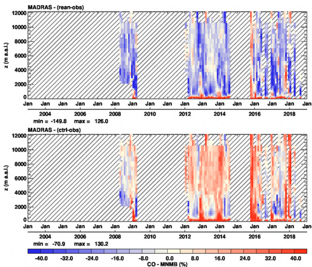
Figure 5.2.5: Time series of the monthly scores (MNMB) for CO at Madras during the period 2003-2018. From top to bottom panel, the scores are for: CAMS reanalysis and control run. Units: %.
