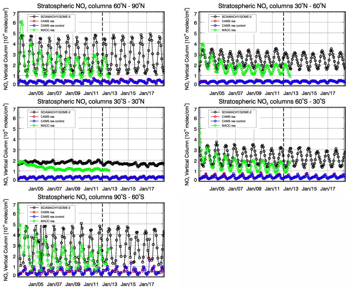
Fig. 8.4.1: Time series of average stratospheric NO 2 columns [10 15 molec. cm -2 ] from SCIAMACHY/GOME-2 compared to model results for different latitude bands. The switch from SCIAMACHY to GOME-2 is indicated by the vertical black dashed lines.
