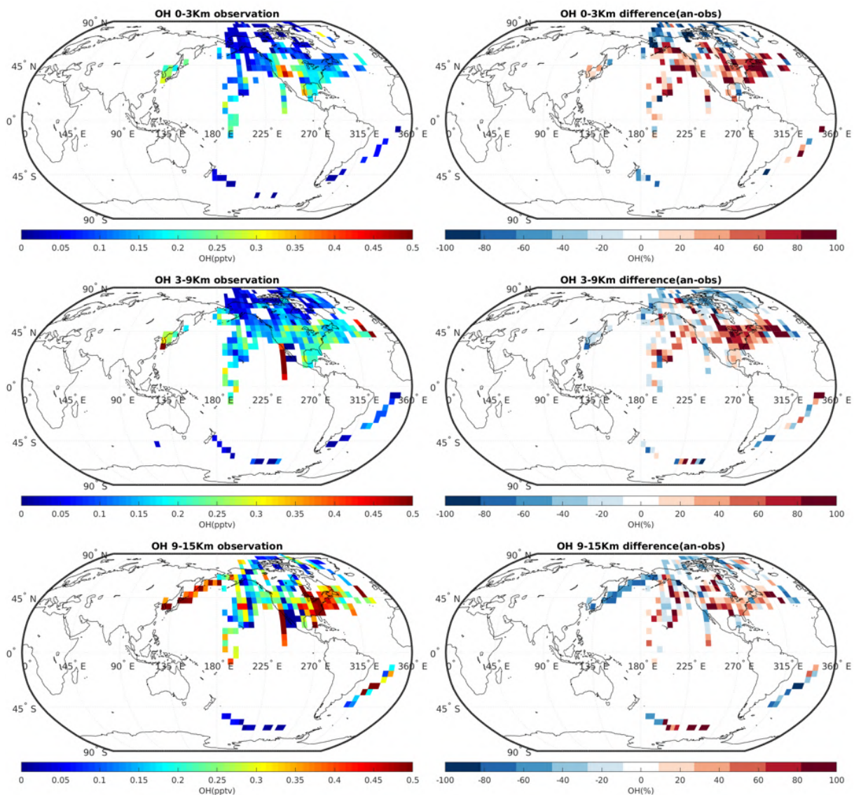
Figure 7.2.9: The campaign observation of OH in pptv (left, see table 7.1.1 and 7.1.2), the difference between the reanalysis and the observation (difference = reanalysis – observation; right). The data are averaged to 5x5 (latitude x longitude) and to three altitude bins: 0-3 Km (top), 3-9 Km (middle), and 9-15Km (bottom).
