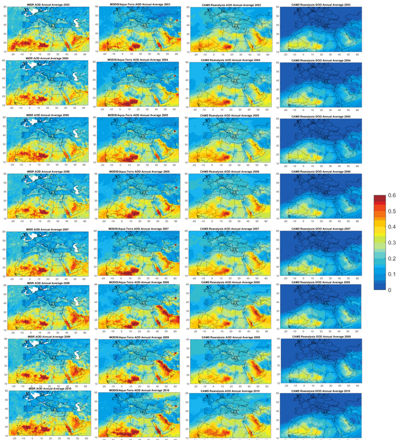
Figure 3.2.1a: Annual averaged AOD from MISR monthly Level 3 monthly 0.5^\circ \times 0.5^\circ global product (first column), MODIS Collection 6 Terra/Aqua merged Dark target and Deep Blue Level 3 daily 1^\circ \times 1^\circ global product (second column), as well as AOD (third column) and DOD from CAMS reanalysis (fourth column) (at 12UTC) for the years 2003-2010.
