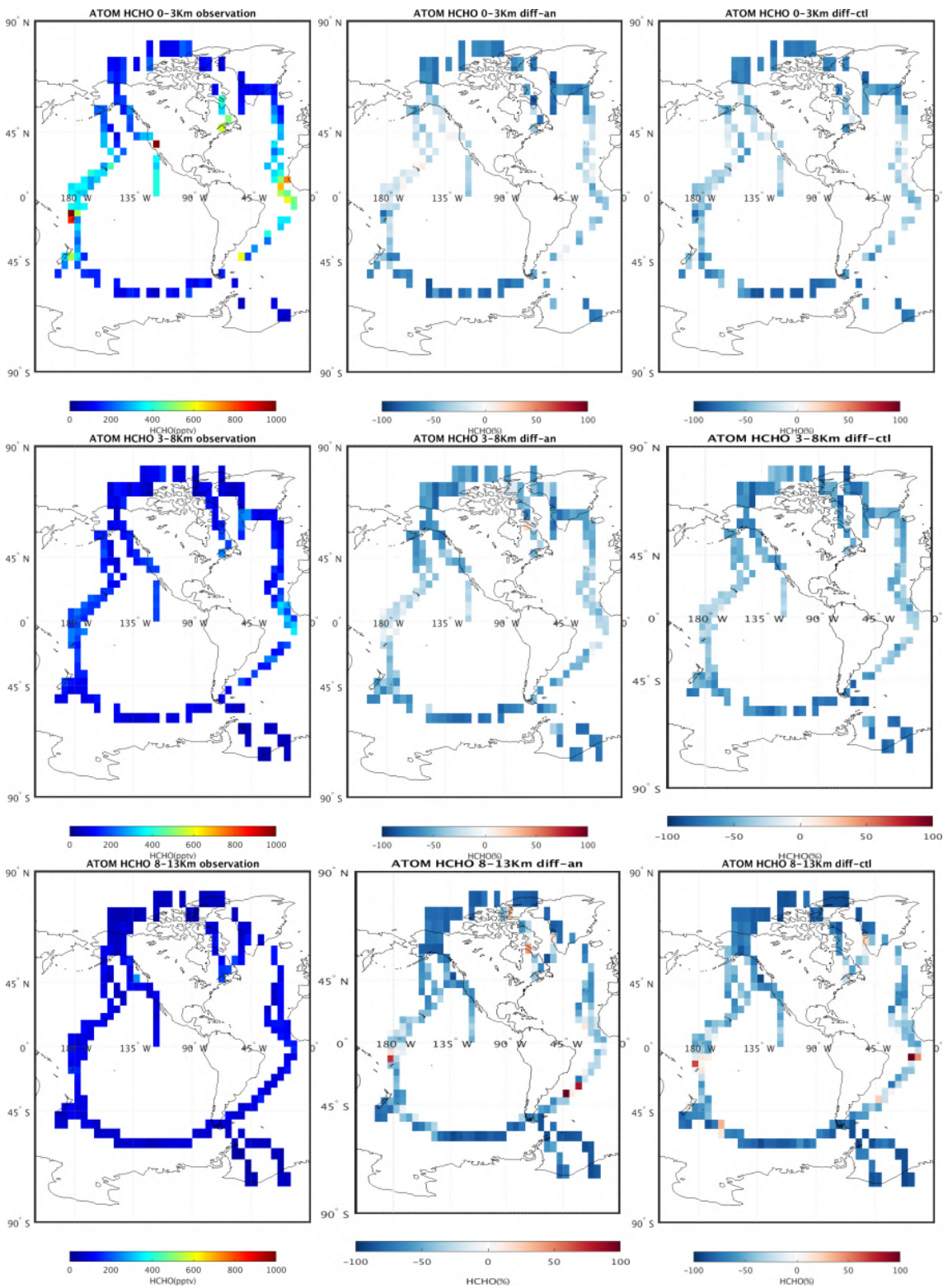
Figure 7.3.3: ATOM campaign observations of HCHO in pptv (left, see table 7.1.1 and 7.1.2), the difference between the reanalysis and the observation (difference = reanalysis – observation; centre), and the difference between the control run and the observation (difference = control – observation; right). The data are averaged to 5°x5° (latitude x longitude) and to three altitude bins: 0-3 km (top), 3-9 km (middle), and 9-15 km (bottom).
