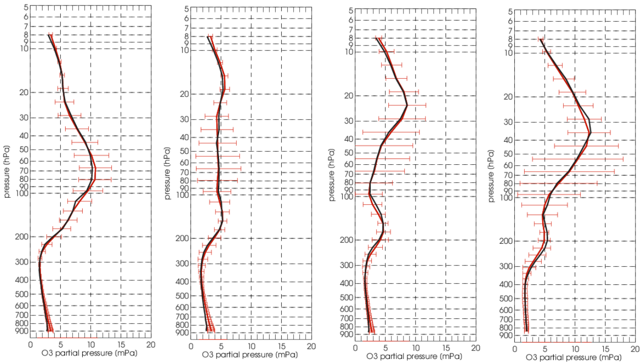
Fig. 8.1.3: Ozone profiles compared with ozone sonde observations in August, September, October and November 2005 (ozone hole period) over the Antarctic.
