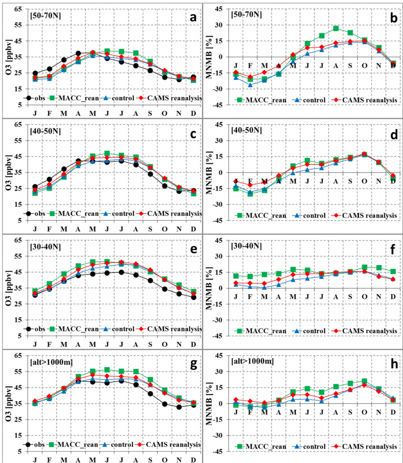
Figure 4.3.1. Mean monthly ozone variability for the period 2003-2018 (left) and the MNMBs (right) of the CAMS reanalysis (red robs), the associated CAMS control run (blue triangles), the MACC reanalysis (green squares), and the EMEP observations (black circles) over Northern Europe (1st row, a and b), Central Europe (2nd row, c and d), Southern Europe (3rd row, e and f) as well as for stations with altitude greater than 1000m above sea level (4rd row, g and h).
