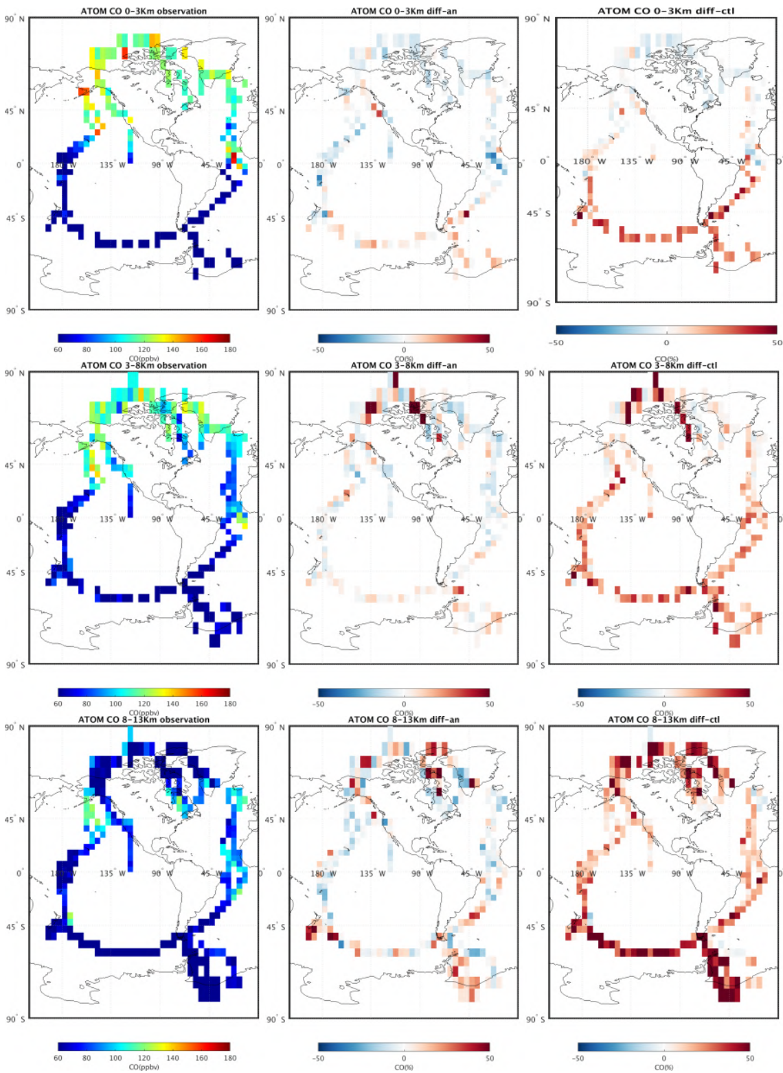
Figure 7.3.2: ATOM campaign observations of CO in ppbv (left, see table 7.1.1 and 7.1.2), the difference between the reanalysis and the observation (difference = reanalysis – observation; centre), and the difference between the control run and the observation (difference = control – observation; right). The data are averaged to 5°x5° (latitude x longitude) and to three altitude bins: 0-3 km (top), 3-9 km (middle), and 9-15 km (bottom).
