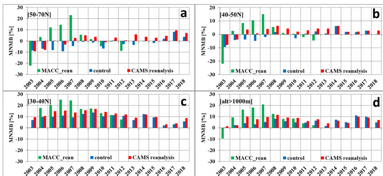
Figure 4.3.3. Annual MNMBs (in %) for the CAMS reanalysis (red), the associated CAMS control run (blue) and MACC reanalysis (green) for the years 2003-2018 of the model simulations and the EMEP observations (black) averaged over European latitudinal zones of 50N-70N (a), 40N-50N (b) and 30N-40N (c) as well as for the group containing stations above 1000m (d).
