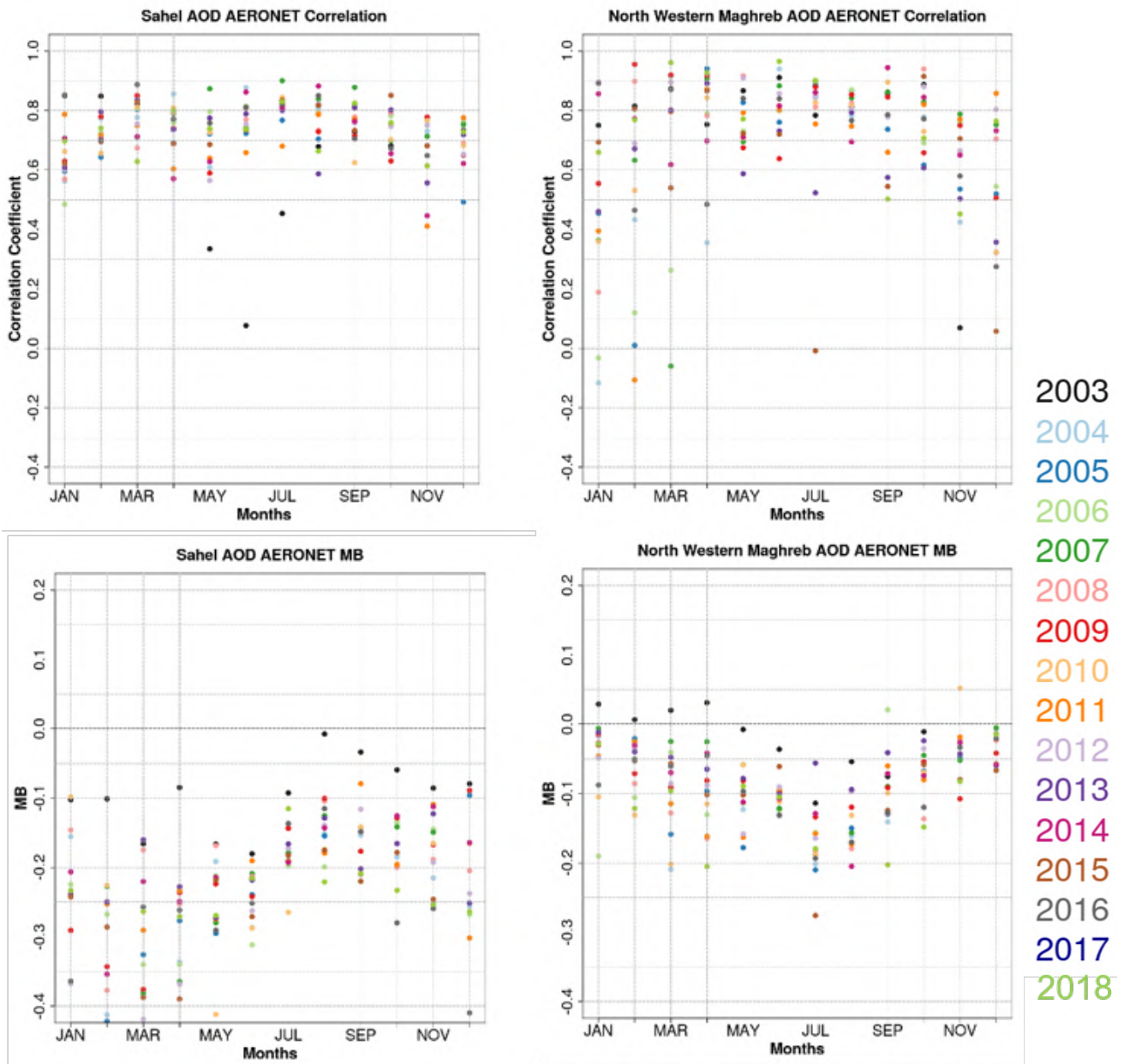
Figure 3.2.3b: Same than Figure 3.2.3a but for the Sahel and North Western Maghreb.
