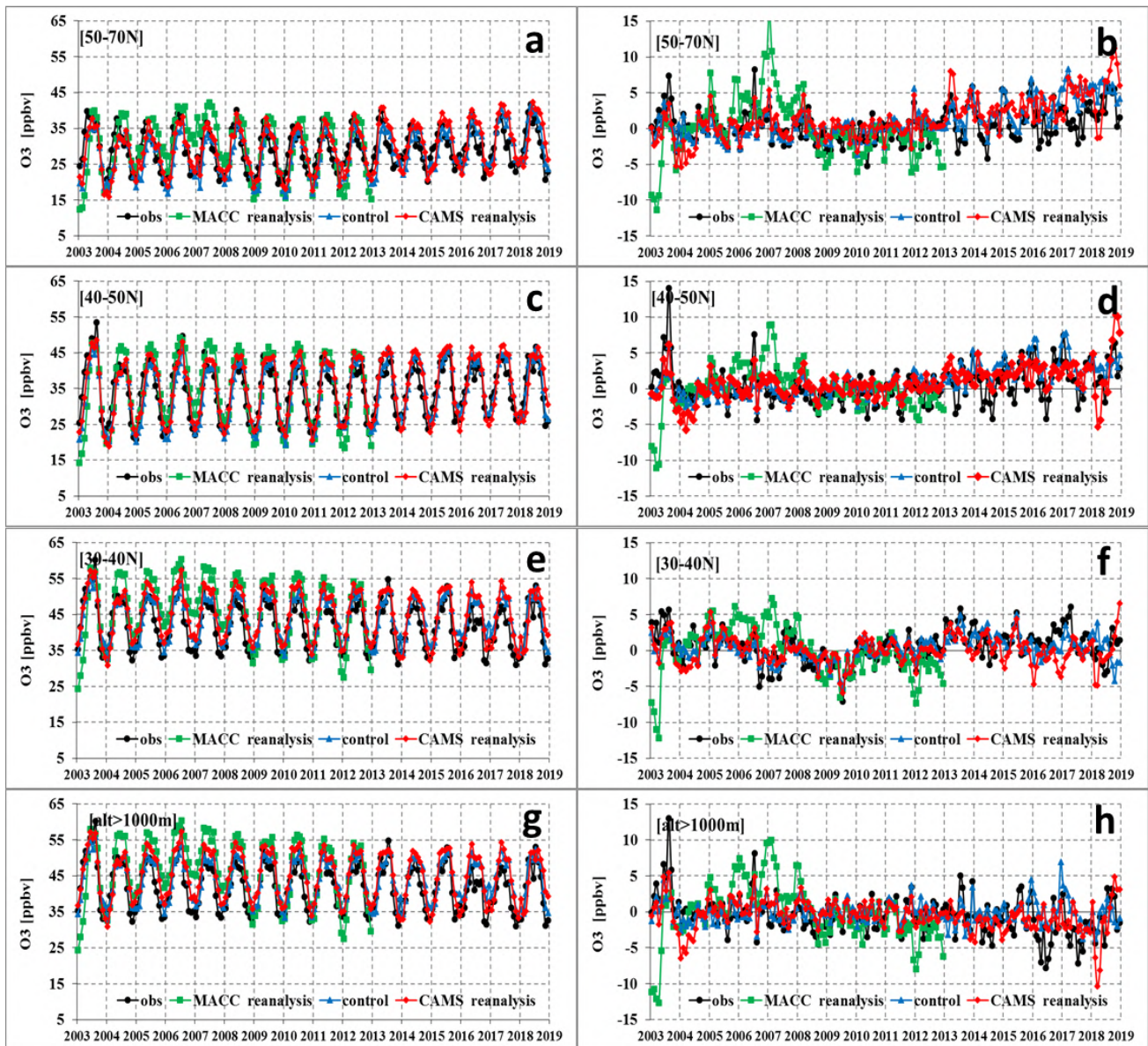
Figure 4.3.2. Monthly mean ozone concentrations during the period 2003-2018 before (left) and after removing the seasonal cycle (right), of CAMS reanalysis (red), the associated CAMS control run (blue), the MACC reanalysis (green) and the EMEP observations (black) averaged over European latitudinal zones of 50N-70N (1st row), 40N-50N (2nd row) and 30N-40N (3rd row) as well as for the group containing stations above 1000m (4th row).
