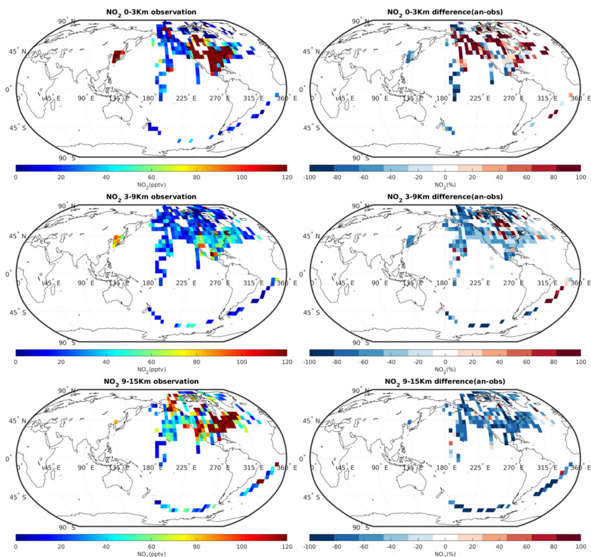
Figure 7.2.7: The campaign observation of NO 2 in pptv (left, see table 7.1.1 and 7.1.2), the difference between the reanalysis and the observation (difference = reanalysis – observation; right). The data are averaged to 5x5 (latitude x longitude) and to three altitude bins: 0-3 Km (top), 3-9 Km (middle), and 9-15Km (bottom).
