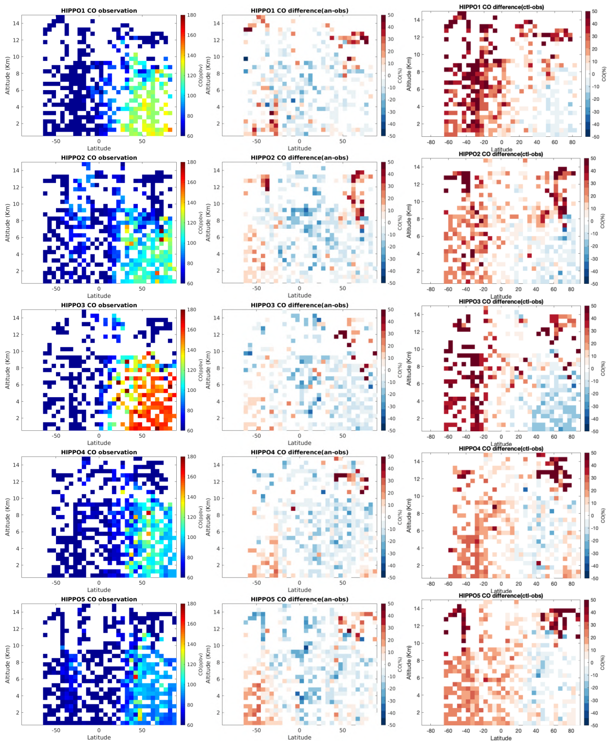
Figure 7.2.4: The HIPPO observation of CO in ppbv (left, see table 7.1.1 and 7.1.2), the difference between the reanalysis and the observation (difference = reanalysis – observation; centre), and the difference between the control run and the observation (difference = control – observation; right) against latitudes and altitudes. The data points are averaged to 5° (latitude) and 0.5 Km (altitude) bins.
