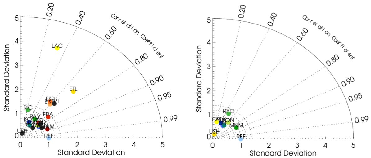
Figure 5.1.5: Taylor diagram for CO for GAW stations in 2003 (first row, left), 2005 (first row, right), 2007, 2009, 2011, 2013, 2015 and 2018 (last row, right).
