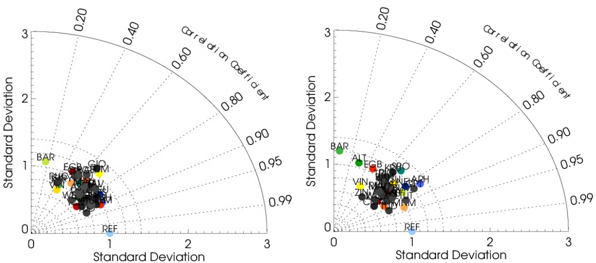
Figure 4.2.3b: Same as Figure 4.2.3a but for the MACC reanalysis
