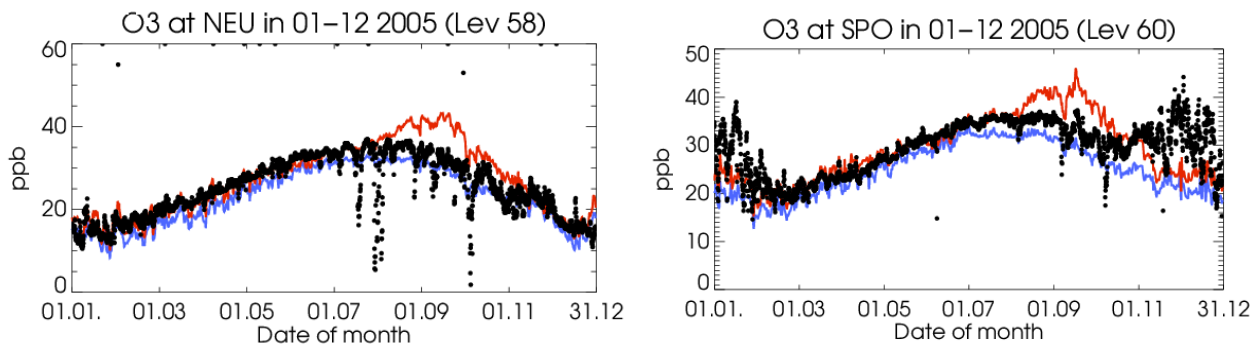
Figure 4.2.11: Time series for O 3 for Neumayer Station (left panel) and South Pole station (right panel) during the year of 2005 (red: analysis, blue: control).
