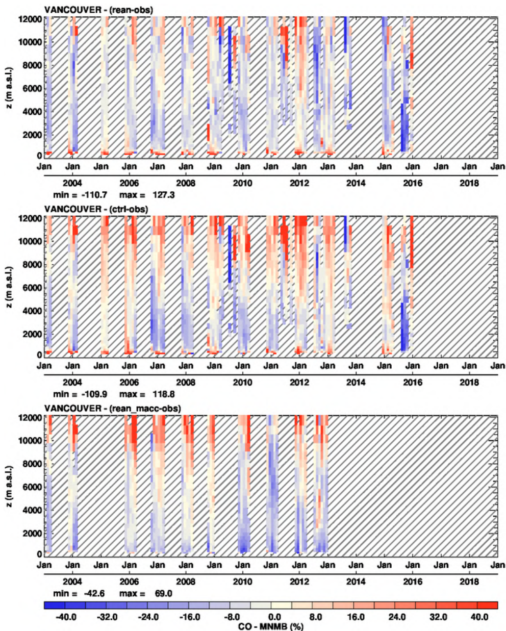
Figure 5.2.3: Time series of the monthly scores against IAGOS (MNMB) for CO at Vancouver during the period 2003-2018. From top to bottom panel, the scores are for: CAMS reanalysis, control run and MACC reanalysis. Units: %.
