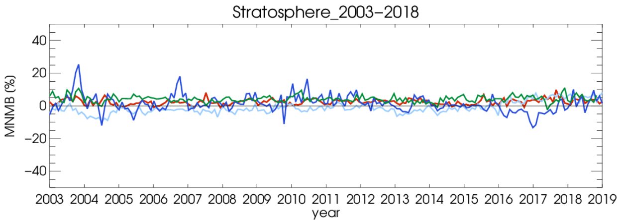
Fig. S.12: Normalised bias of the reanalysis versus ozone sondes, for 4 regions in the stratosphere (dark blue: Antarctic, light blue: Arctic, red: Northern midlatitudes, green: Tropics). The biases are averaged between 90 and 10hPa in the extra-tropics and between 60 and 10hPa in the Tropics.
