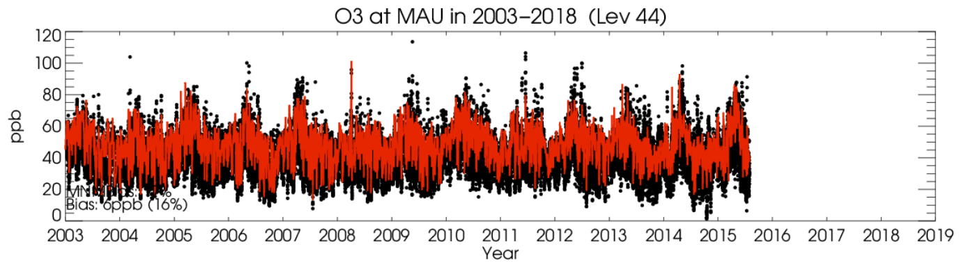
Figure 4.2.9: Timeseries for O 3 in the period 2003-2015 for GAW station Mauwi (MAU) in the Tropics
