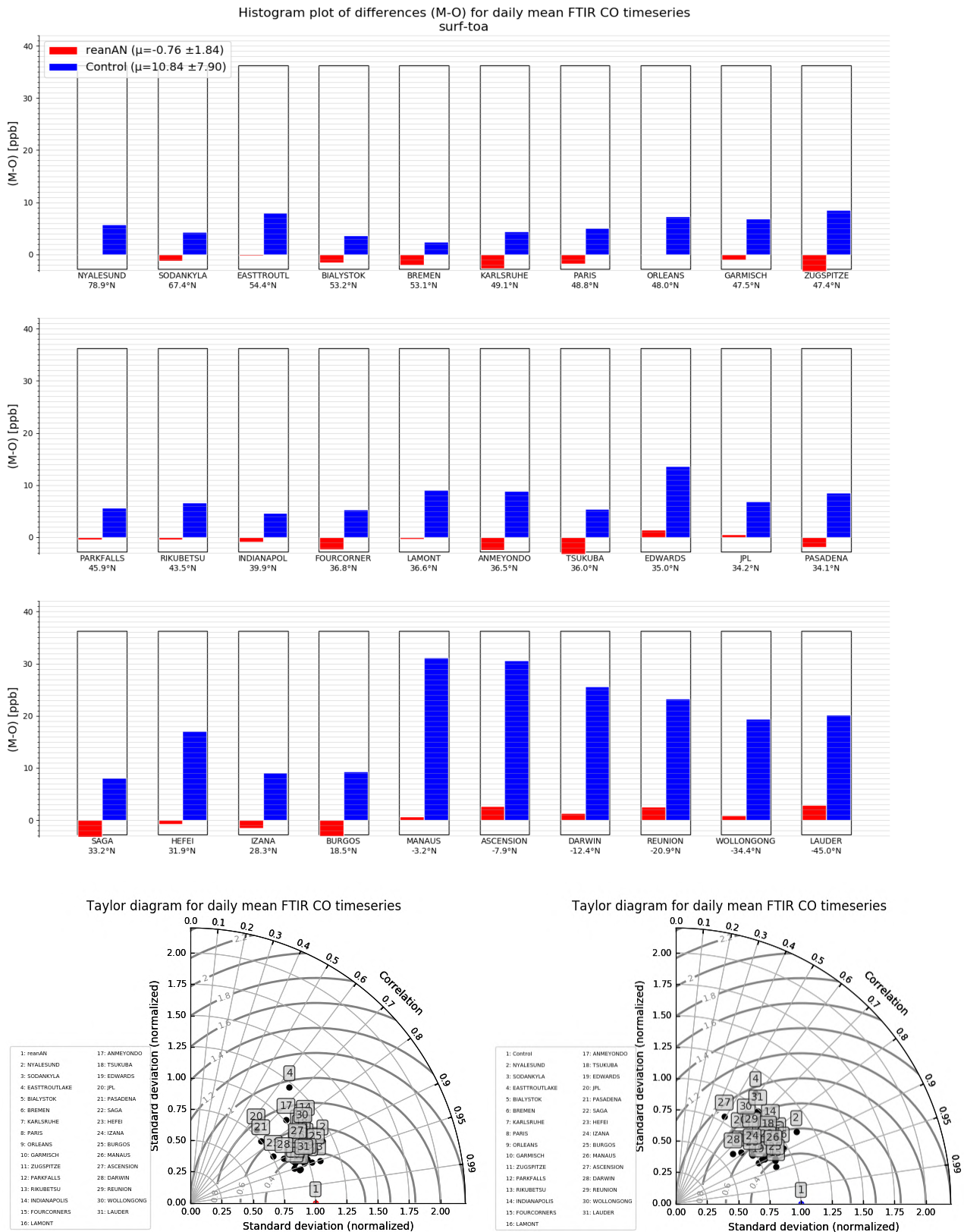
Figure 5.4.2: Histogram plot (top, sorted by decreasing latitude) of averaged daily XCO differences against FTIR for CAMS reanalysis (red) and Control run (blue) and Taylor diagrams (bottom-left: reanalysis; bottom-right: control run).
