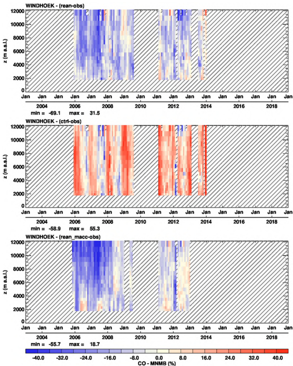
Figure 5.2.9: Time series of the monthly scores against IAGOS (MNMB) for CO at Windhoek during the period 2003-2018. From top to bottom panel, the scores are for: CAMS reanalysis, control run and MACC reanalysis. Units: %.
