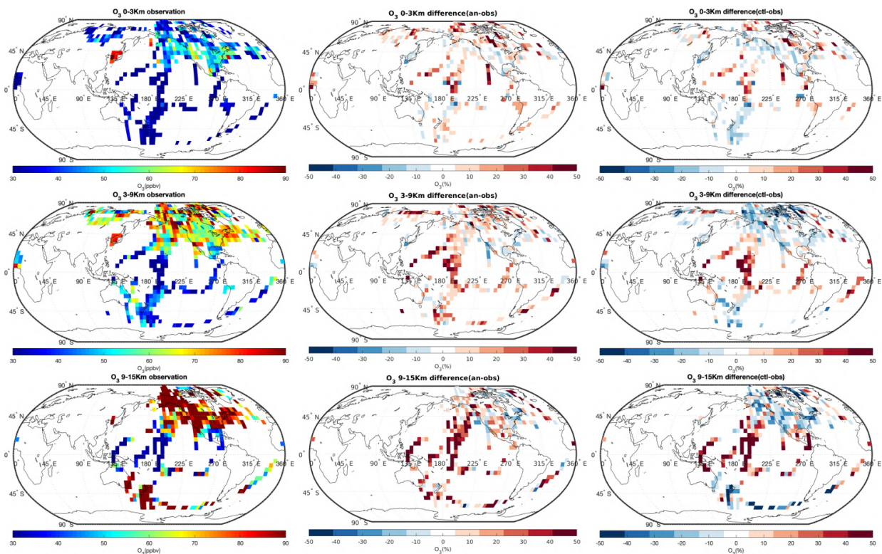
Figure 7.2.1: The campaign observations of O_3 in ppbv (left, see table 7.1.1 and 7.1.2), the difference between the reanalysis and the observation (difference = reanalysis – observation; centre), and the relative difference in % between the control run and the observation (difference = control – observation; right). The data are averaged to 5^\circ \times 5^\circ (latitude x longitude) and to three altitude bins: 0-3 km (top), 3-9 km (middle), and 9-15 km (bottom).
