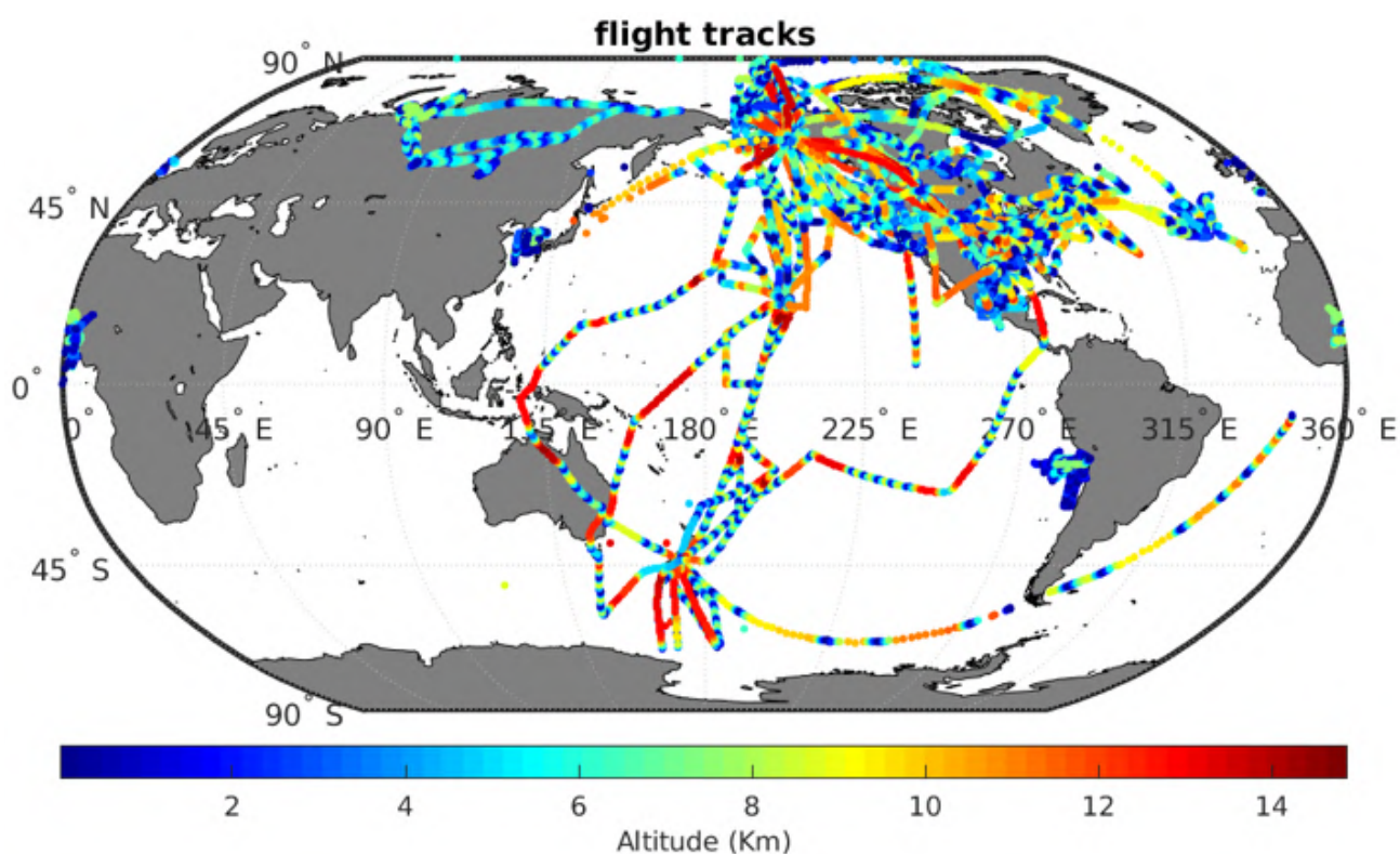
Figure 7.1.1: Flight tracks of the campaigns included in Table 7.1.1 and 7.1.2.
