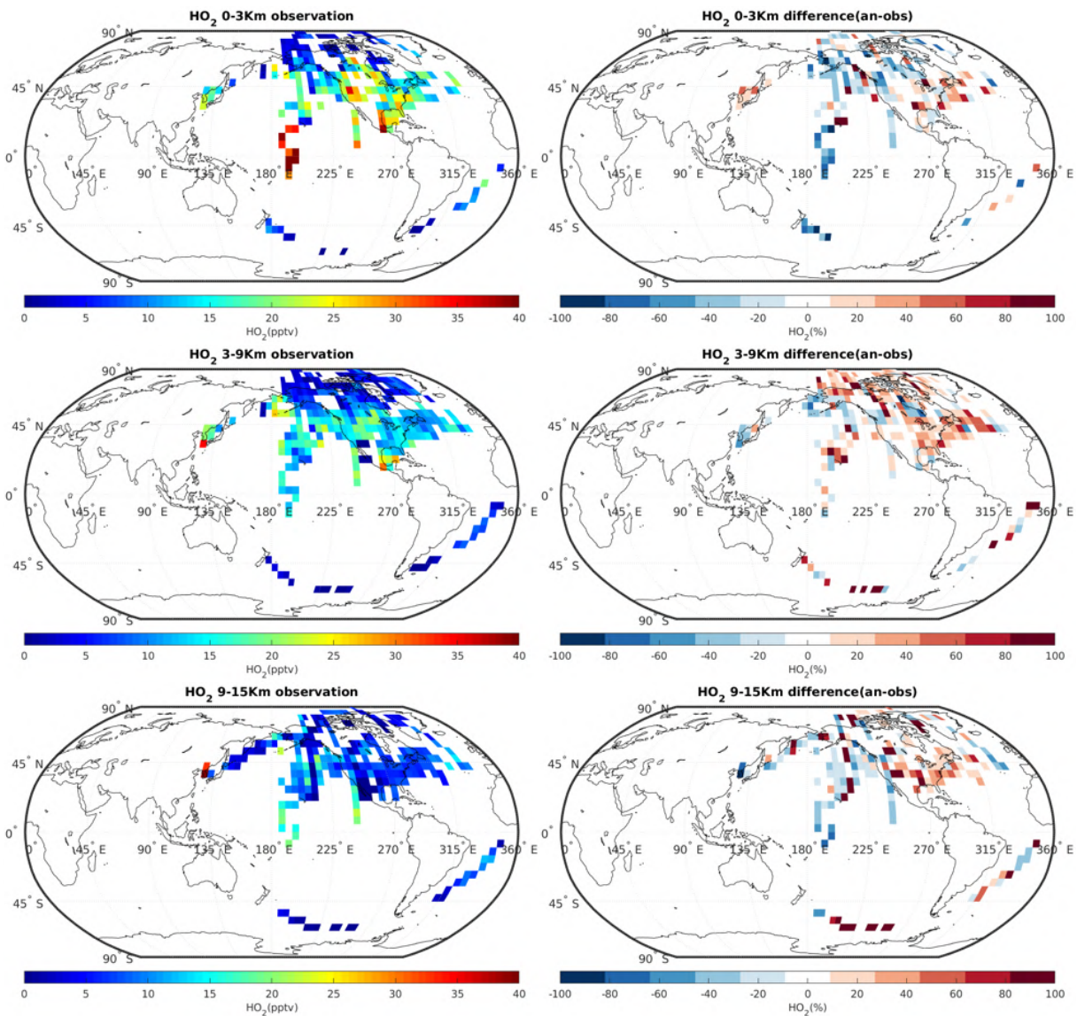
Figure 7.2.10: The campaign observation of HO 2 in pptrv (left, see table 7.1.1 and 7.1.2) and the difference between the reanalysis and the observation (difference = reanalysis – observation; right). The data are averaged to 5x5 (latitude x longitude) and to three altitude bins: 0-3 Km (top), 3-9 Km (middle), and 9-15Km (bottom).
