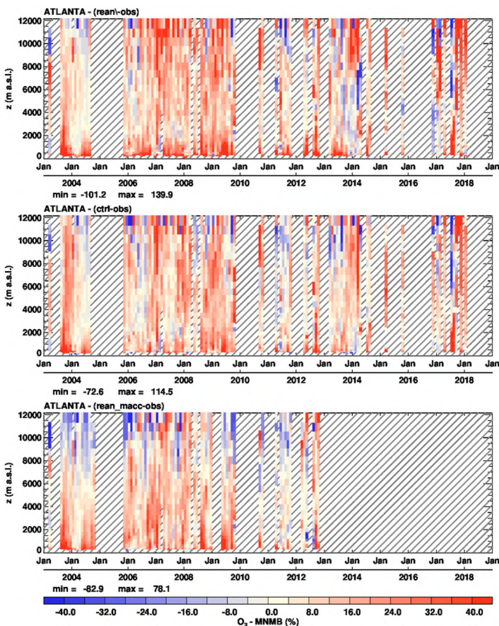
Figure 4.4.3: Time series of the monthly scores (MNMB) for ozone at Atlanta during the period 2003-2018. From top to bottom panel, the scores are for: CAMS reanalysis, control run and MACC reanalysis. Units: %.
