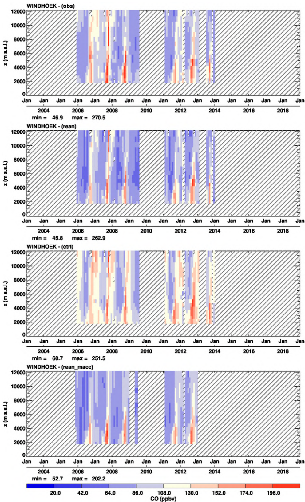
Figure 5.2.8: Time series of the monthly profiles for CO at Windhoek during the period 2003-2018. From top to bottom panel the time series correspond to: IAGOS (MOZAIC), CAMS reanalysis, control run and MACC reanalysis. Units: ppbv.
