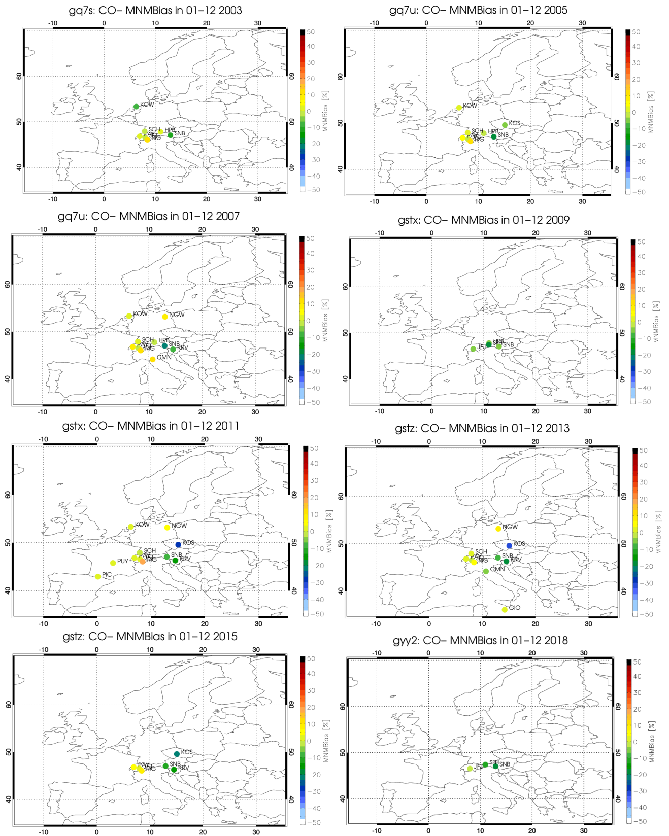
Figure 5.1.4: Distribution of overall MNMBs for the CAMS reanalysis against GAW for CO for the years 2003, 2005, 2007, 2009, 2011, 2013, 2015 and 2018.
