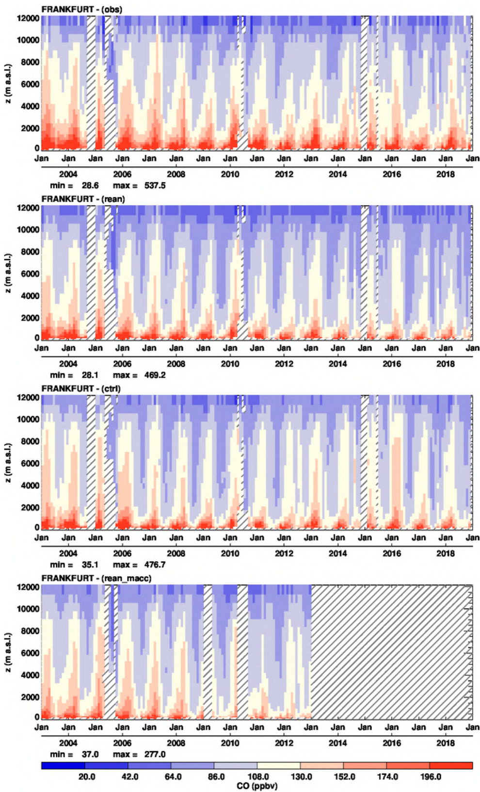
Figure 5.2.1: Time series of the monthly profiles for CO at Frankfurt during the period 2003-2018. From top to bottom panel the time series correspond to: IAGOS (MOZAIC), CAMS reanalysis, control run and MACC reanalysis. Units: ppbv.
