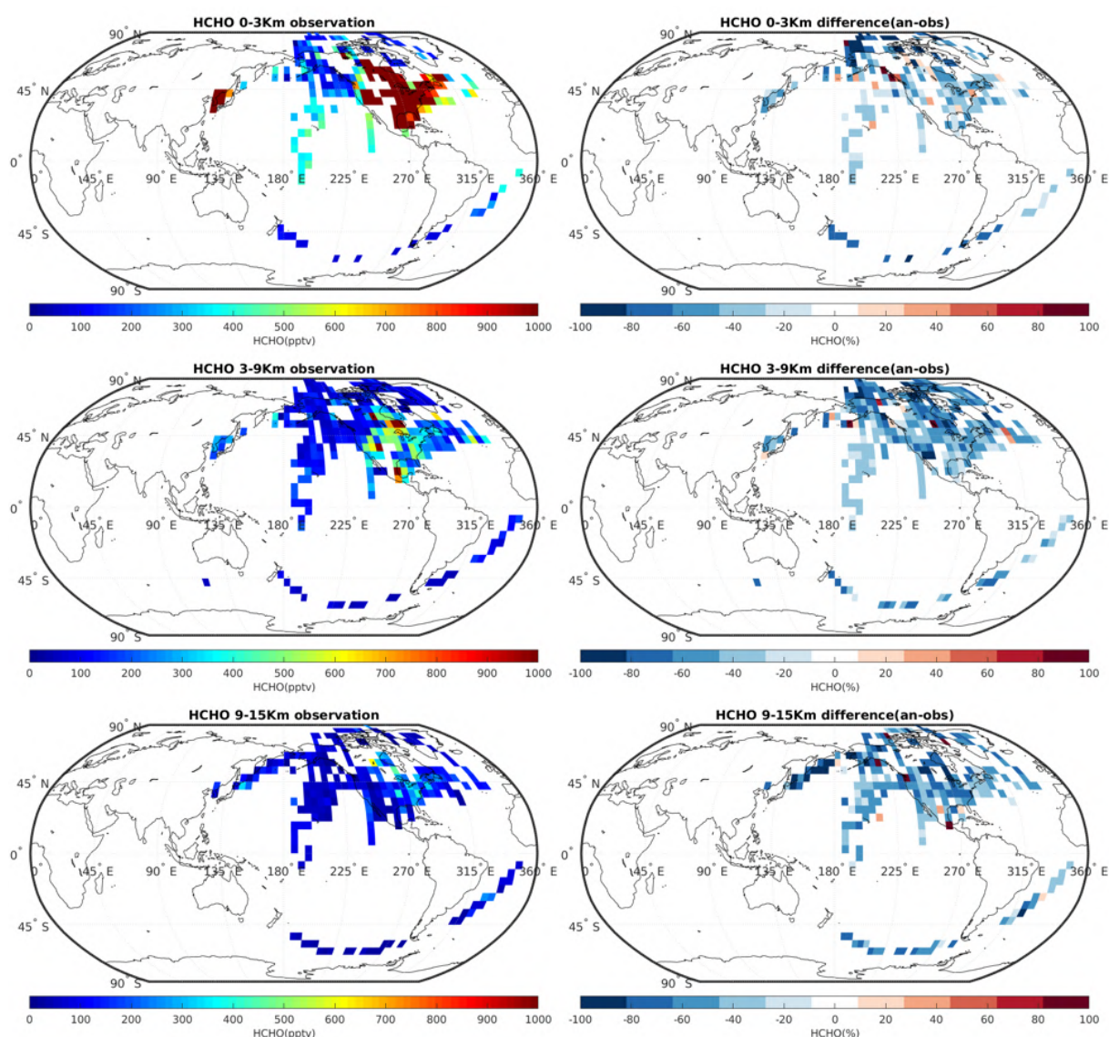
Figure 7.2.5: The campaign observation of HCHO in pptv (left, see table 7.1.1 and 7.1.2), the difference between the reanalysis and the observation (difference = reanalysis – observation; right). The data are averaged to 5^{\circ} \times 5^{\circ} (latitude x longitude) and to three altitude bins: 0-3 Km (top), 3-9 Km (middle), and 9-15Km (bottom).
