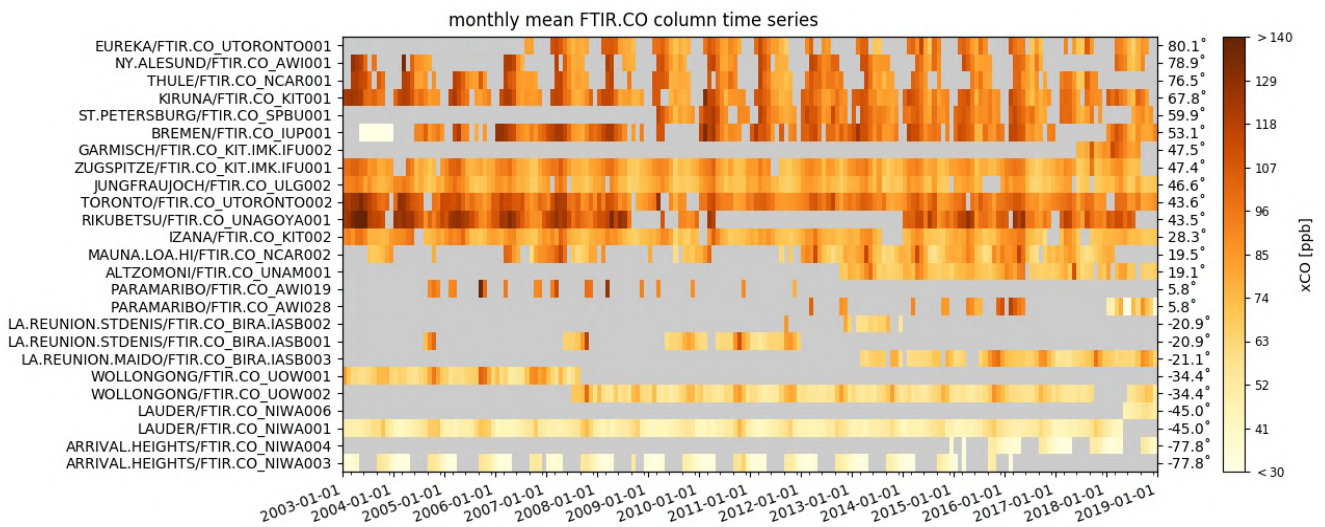
Figure 5.3.1: Overview of CO data product time series available on NDACC. Most FTIR data products are used in this study. Sites are sorted by latitude. The plot shows dry air column averaged CO.
