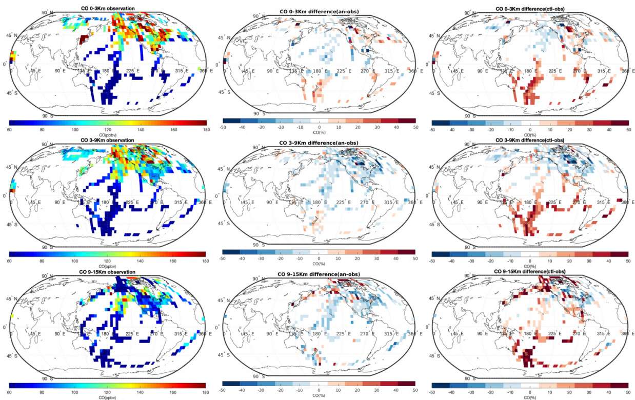
Figure 7.2.3: The campaign observation of CO in ppbv (left, see table 7.1.1 and 7.1.2), the difference between the reanalysis and the observation (difference = reanalysis – observation; centre), and the difference between the control run and the observation (difference = control – observation; right). The data are averaged to 5^{\circ} \times 5^{\circ} (latitude x longitude) and to three altitude bins: 0-3 Km (top), 3-9 Km (middle), and 9-15Km (bottom).
