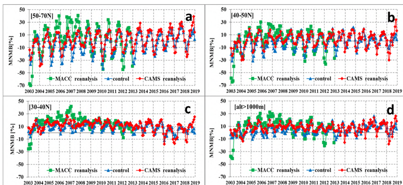
Figure 4.3.4. Monthly MNMBs (in %) for the CAMS reanalysis (red), the associated CAMS control run (blue) and MACC reanalysis (green) for the years 2003-2018 of the model simulations and the EMEP observations (black) averaged over European latitudinal zones of 50N-70N (a), 40N-50N (b) and 30N-40N (c) as well as for the group containing stations above 1000m (d).
