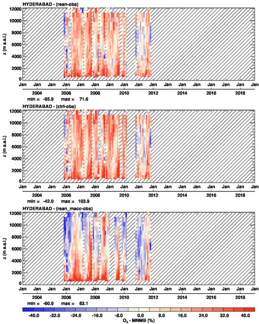
Figure 4.4.5: Time series of the monthly scores (MNMB) for ozone at Hyderabad during the period 2003-2018. From top to bottom panel, the scores are for: CAMS reanalysis, control run and MACC reanalysis. Units: %.
