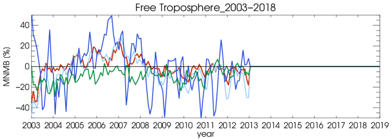
Figure 4.1.1b: like Figure 4.1.1a but for the MACC reanalysis
