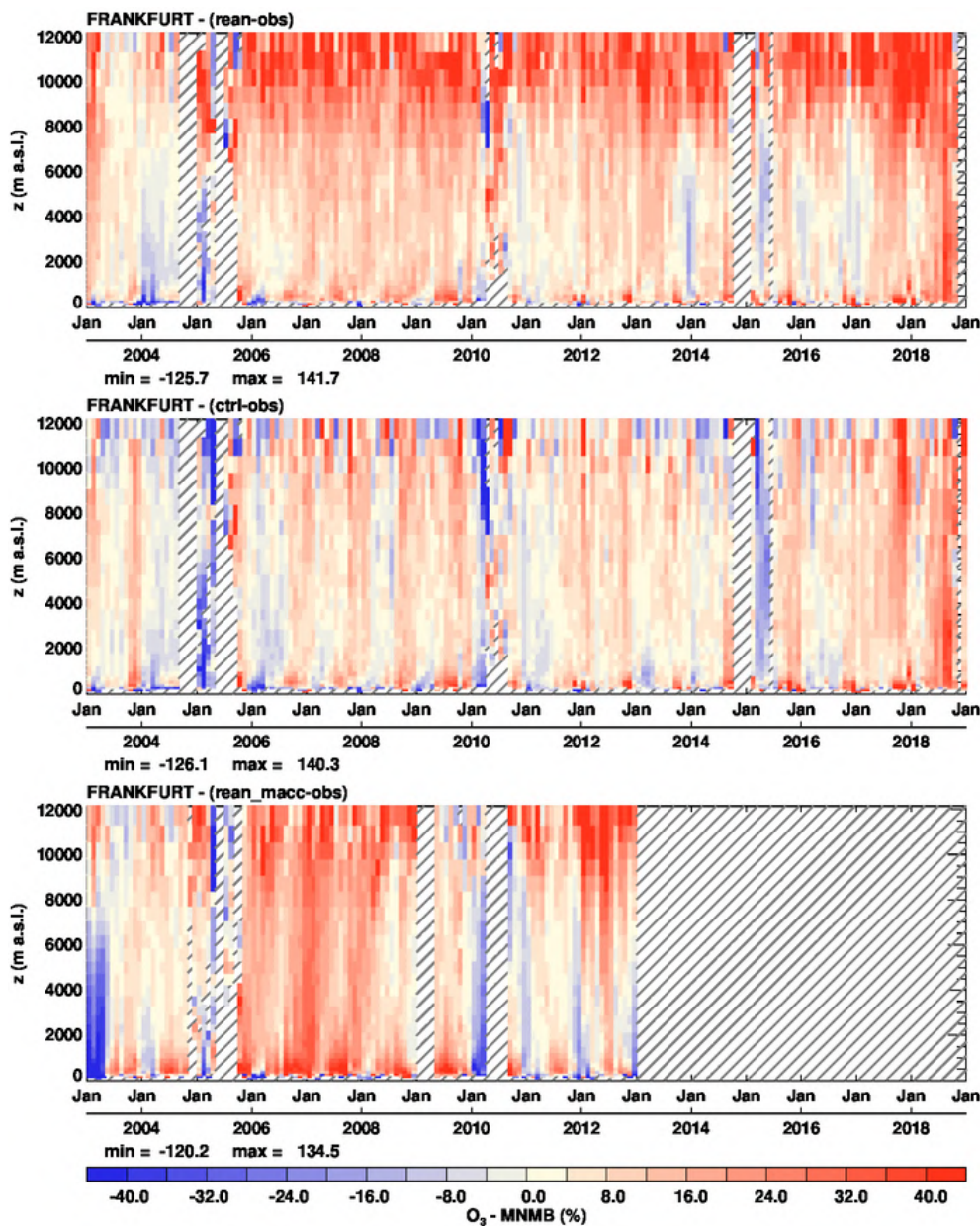
Figure 4.4.2: Time series of the monthly scores (MNMB) for ozone at Frankfurt during the period 2003-2018. From top to bottom panel, the scores are for: CAMS reanalysis, control run and MACC reanalysis. Units: %.
