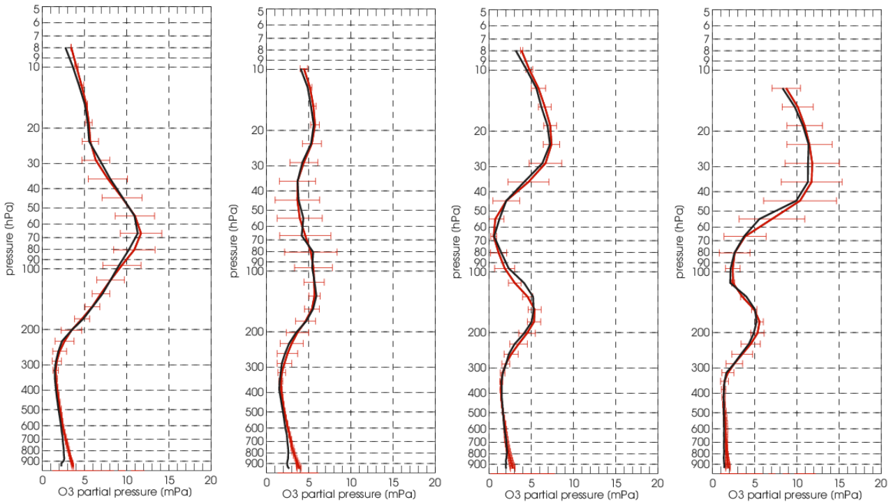
Fig. 8.1.5: Ozone in August, September, October and November 2009 (ozone hole period) over the Antarctic.
