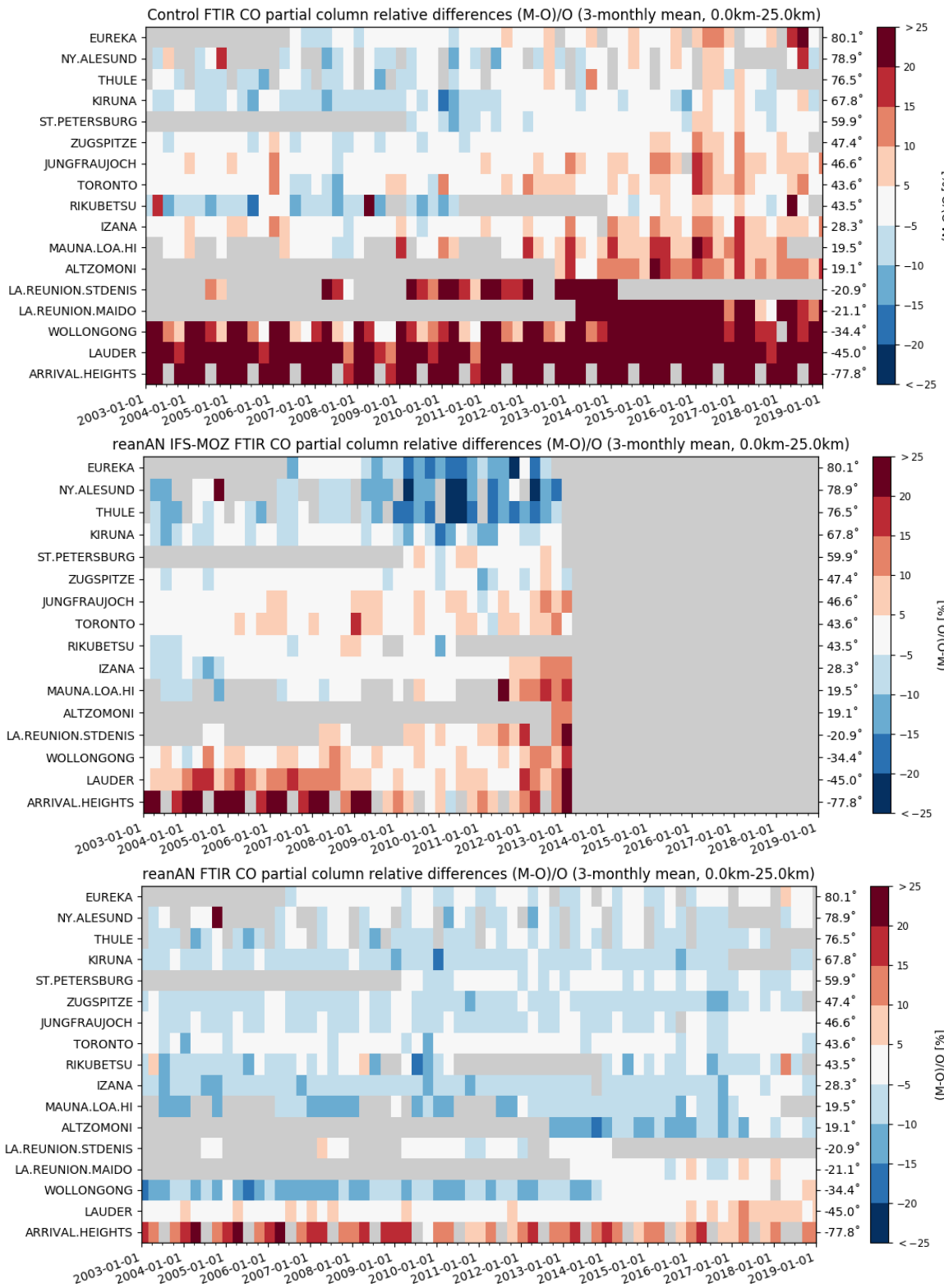
Figure S.6: Mosaic plot of seasonal relative biases in CO ( [\text{reanalysis-observation}]/\text{observation} ) at all NDACC FTIR sites. The CAMS reanalysis (bottom) performs more stable compared to the MACC reanalysis (middle). A slight negative bias is found in the NH. At the tropical sites in the northern hemisphere the negative bias reaches values up to 10% (Izana, Mauna Loa, Altzomoni). The control run shows a strong positive bias in the southern hemisphere efficiently corrected by the assimilation.
