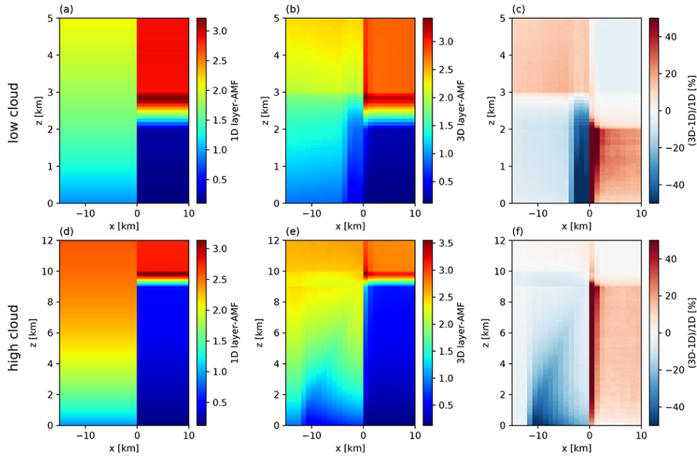
Figure 7. Layer air mass factors for the two base cases ( \text{SZA} = 50^\circ , surface albedo = 0.05) for cloud shadow geometry: layer-AMFs calculated using 1D approximation (clear sky from x = -15 to x = 0 km and 1D cloud layer from x = 0 to x = 10 km) for low cloud (a) and high cloud (d), 3D simulation of layer-AMFs for low cloud (b) and high cloud (e), and relative difference between 1D and 3D simulation for low cloud (c) and high cloud (f). Note that the altitude range z in the upper panels (a–c) is from 0 to 5 km and in the lower panels (d–f) from 0 to 12 km.
