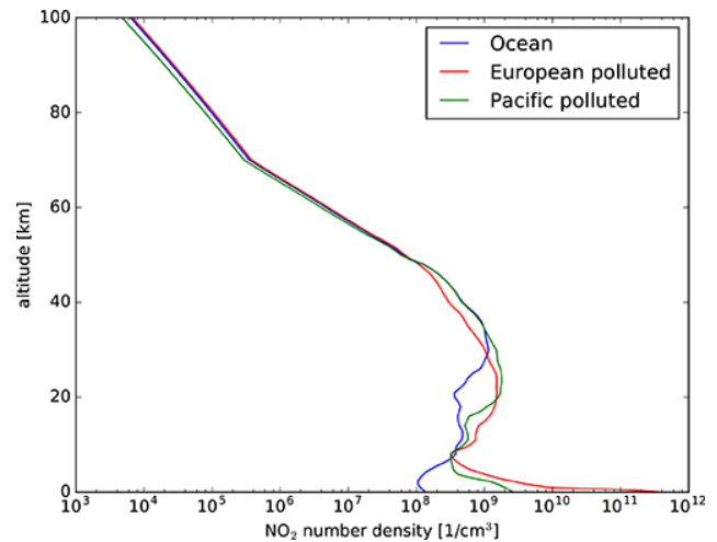
Figure 1. NO 2 number concentration profiles for typical scenarios taken from the CAMELOT study (Levelt et al., 2009).
