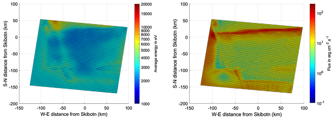
Figure 8. (Left) Mean energy map (in eV) and (right) energy flux map (in \text{erg}\cdot\text{cm}^{-2}\cdot\text{s}^{-1} ), resulting from the optimization method applied to the VER measurements for dataset 2, with a Maxwellian energy distribution. The geographic coordinates here correspond, arbitrarily, to the ones at a 100 km altitude.
