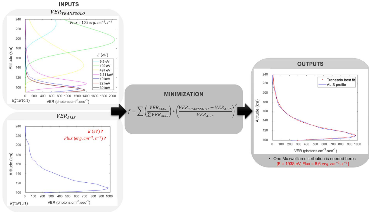
Figure 5. Simplified diagram of the optimization method. INPUTS – (top) Example of few Transsollo runs for mean energies of 9.5 eV, 102 eV, 497 eV, 3.3 keV, 10 keV, 22 keV and 30 keV, and energy flux set at 10.8 \text{ erg}\cdot\text{cm}^{-2}\cdot\text{s}^{-1} , with a Maxwellian distribution; (bottom) Example of an VER field-aligned profile for a given location in the map of the dataset 1 ( X = -46.6 \text{ km} and Y = -13.4 \text{ km} at 100 km altitude). MINIMIZATION – Cost function from the least-square method to minimize the difference between the VER measurements and the VER simulations. OUTPUTS – Result of the minimization. For this example, only one energy distribution is needed to find the best fit: a mean energy of 1.9 keV and an energy flux of 8.6 \text{ erg}\cdot\text{cm}^{-2}\cdot\text{s}^{-1} .
