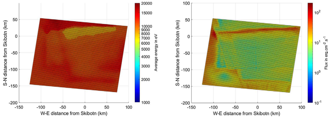
Figure 10. (Left) Mean energy map (in eV) and (right) energy flux map (in \text{erg}\cdot\text{cm}^{-2}\cdot\text{s}^{-1} ), resulting from the optimization method applied to the VER measurements for dataset 2, with a quasi-monoenergetic energy distribution. The geographic coordinates here correspond, arbitrarily, to the ones at a 100 km altitude.
