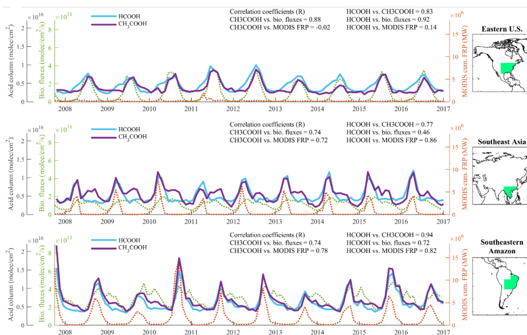
Figure 20. Time series of monthly mean \text{HCOOH} and \text{CH}_3\text{COOH} total column (blue and purple solid lines, respectively), MEGAN–MOHYCAN isoprene and monoterpenes emission fluxes (green dotted line), and cumulative MODIS fire radiative power (orange dotted line) over regions of interest.
