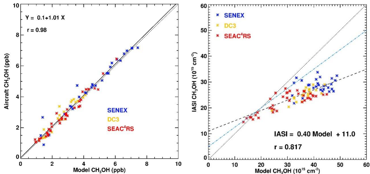
Figure 31. Left: Campaign-averaged CH 3 OH mixing ratios measured in 3 aircraft campaigns vs. model values constrained by those data. Right: Campaign-averaged IASI columns vs. corresponding model values constrained by aircraft data. Only 2°×2.5° pixels with at least 30 aircraft data are used. The linear regression is the dashed line. For comparison, the regression of IASI versus FTIR columns at 3 continental sites is shown as the blue dash-dotted line.
