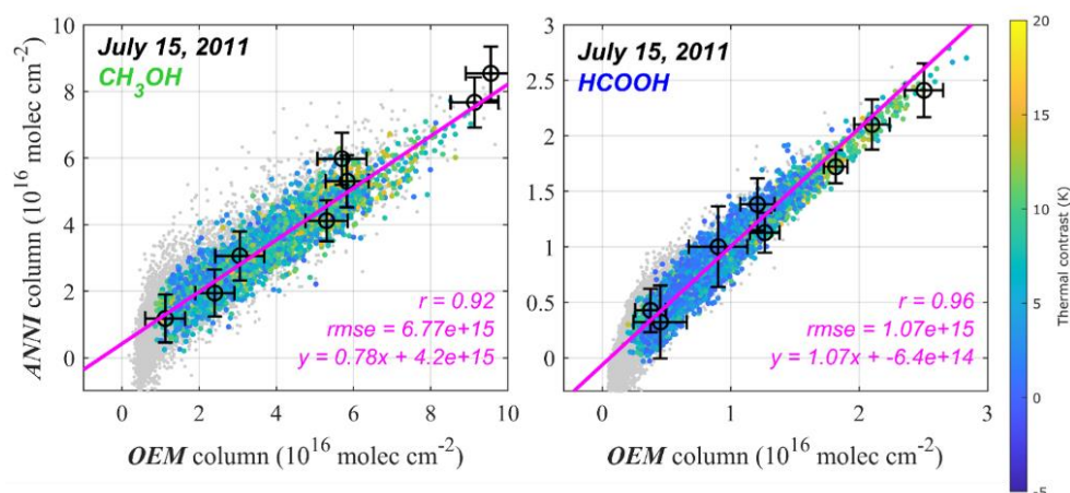
Figure 16. Comparison between CH 3 OH and HCOOH total columns from the ANNI processing (y axis) and retrieved with an OEM (x axis). Pixels are colored by thermal contrast. The measurements filtered out of the comparison are depicted as gray dots. The linear regression, root-mean-square error (rmse) and coefficient of correlation (r) between the two data sets are given in magenta. The ANNI and OEM uncertainties for random measurements are indicated in black.
