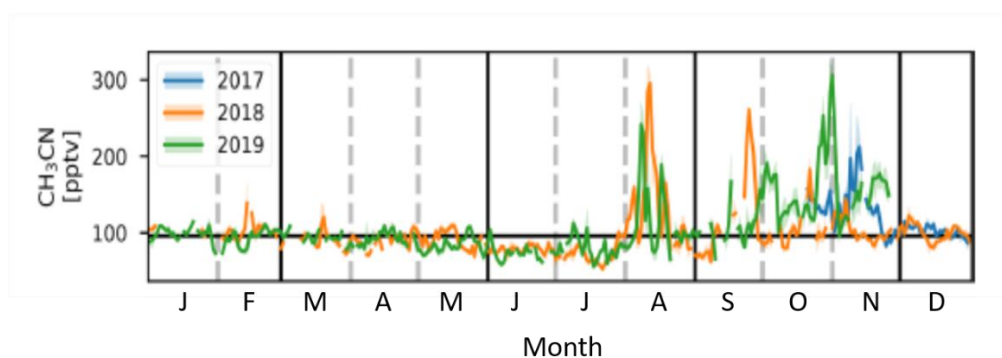
Figure 8. Seasonal variability of daily averaged CH 3 CN concentrations in 2017, 2018 and 2019.
