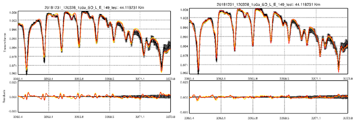
Fig. 12. Retrieval of CO 2 in order 149, showing how the ILS parameters can be used to improve the retrieval forward model fit in a nearby diffraction order. Left: retrieval with a single fixed-width Gaussian ILS; right: with a double Gaussian with parameters as a function of pixel number, derived from order 140. The residual fit is clearly smaller with the double Gaussian, hence the forward model simulation fits the data better.
